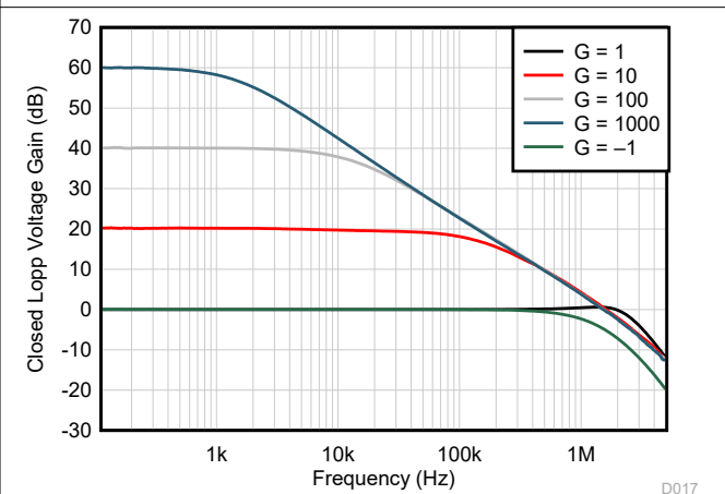
Figure 7-6. Closed-Loop Gain vs Frequency
