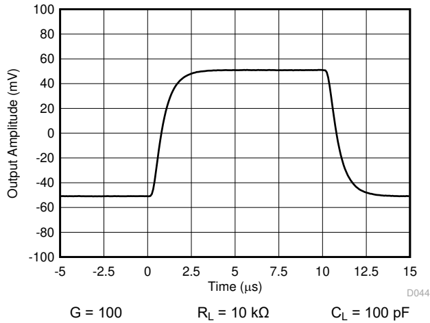
Figure 7-45. Small-Signal Response
