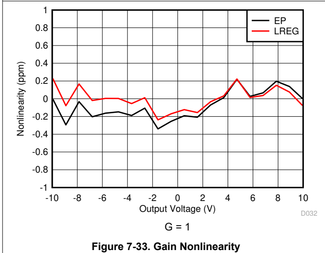
Figure 7-33. Gain Nonlinearity
