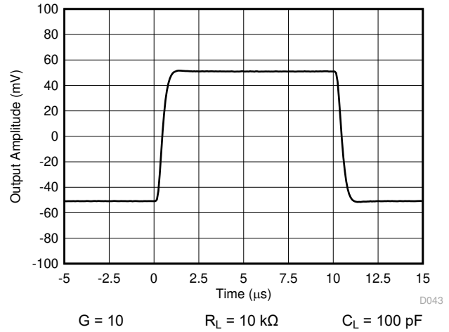
Figure 7-44. Small-Signal Response
