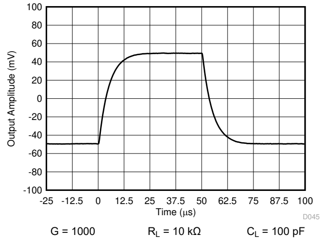
Figure 7-46. Small-Signal Response
