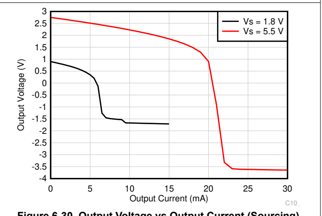
Figure 6-30. Output Voltage vs Output Current (Sourcing)
