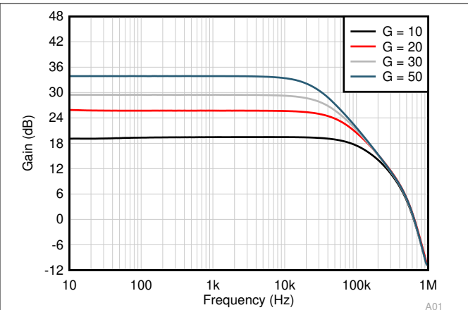
Figure 6-32. Closed-Loop Gain vs Frequency
