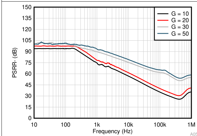
Figure 6-35. PSRR- (Referred to Input) vs Frequency
