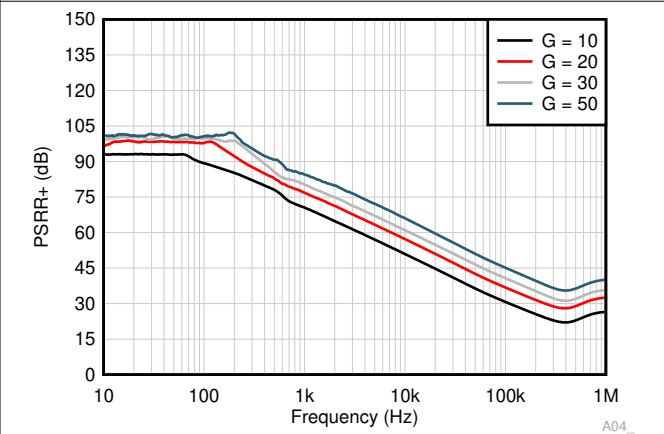
Figure 6-34. PSRR+ (Referred to Input) vs Frequency
