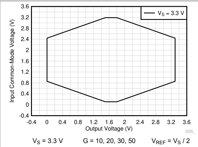
Figure 6-62. Input Common-Mode Voltage vs Output Voltage
