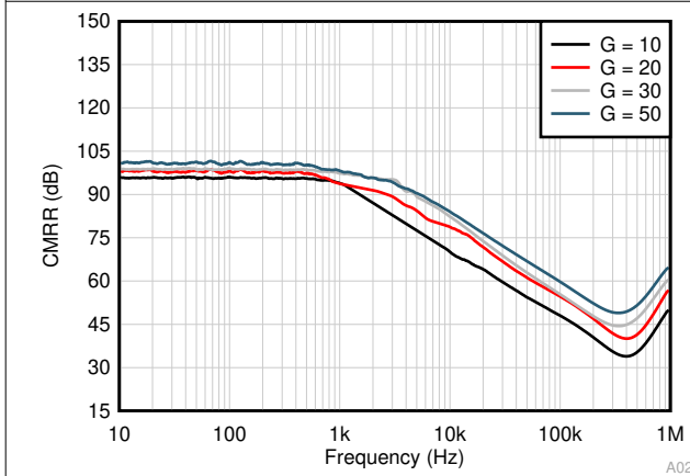
Figure 6-33. CMRR (Referred to Input) vs Frequency
