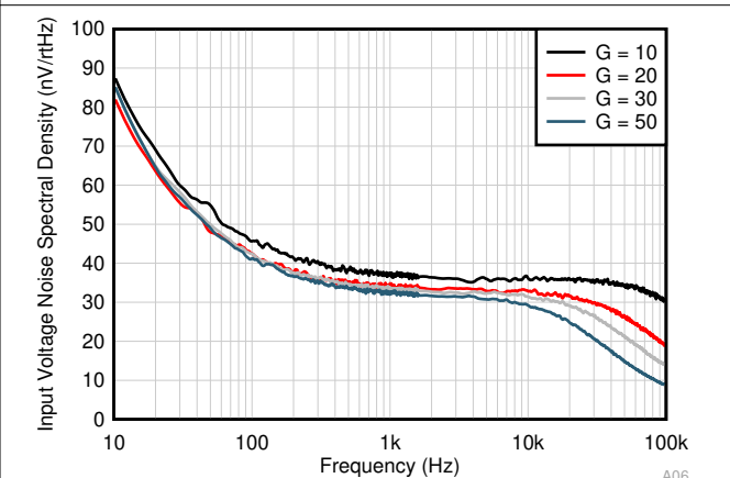
Figure 6-36. Input Referred Voltage Noise Spectral Density
