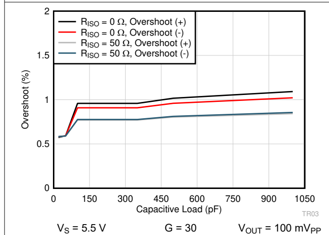
Figure 6-45. Small-Signal Overshoot vs Capacitive Load
