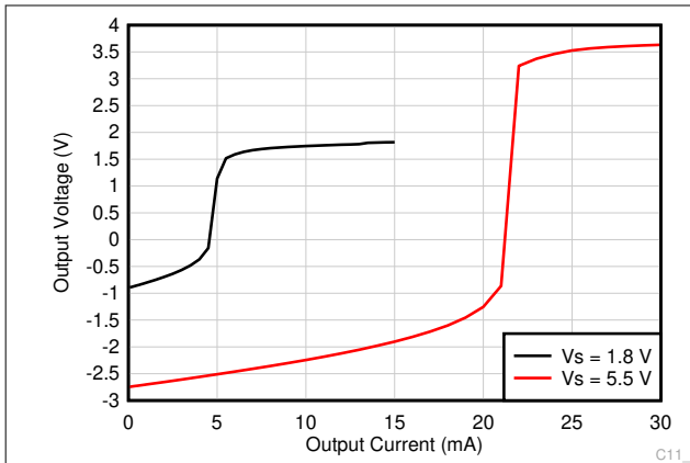
Figure 6-31. Output Voltage vs Output Current (Sinking)
