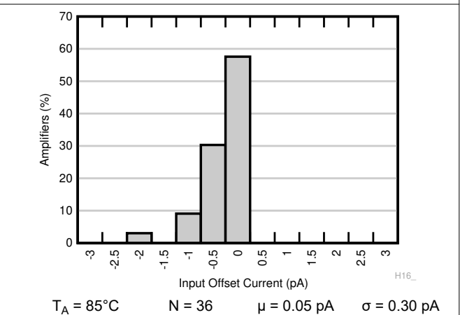
Figure 6-6. Typical Distribution of Input Offset Current
