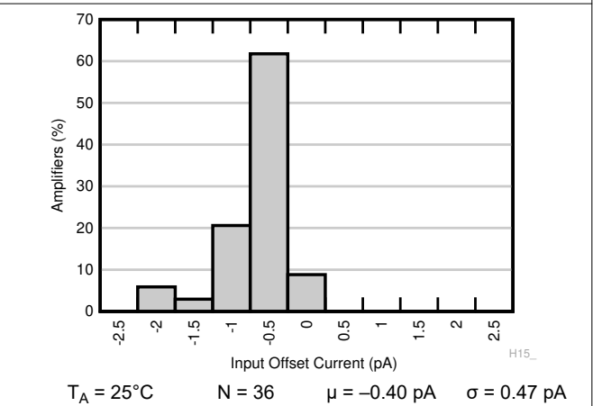
Figure 6-4. Typical Distribution of Input Offset Current
