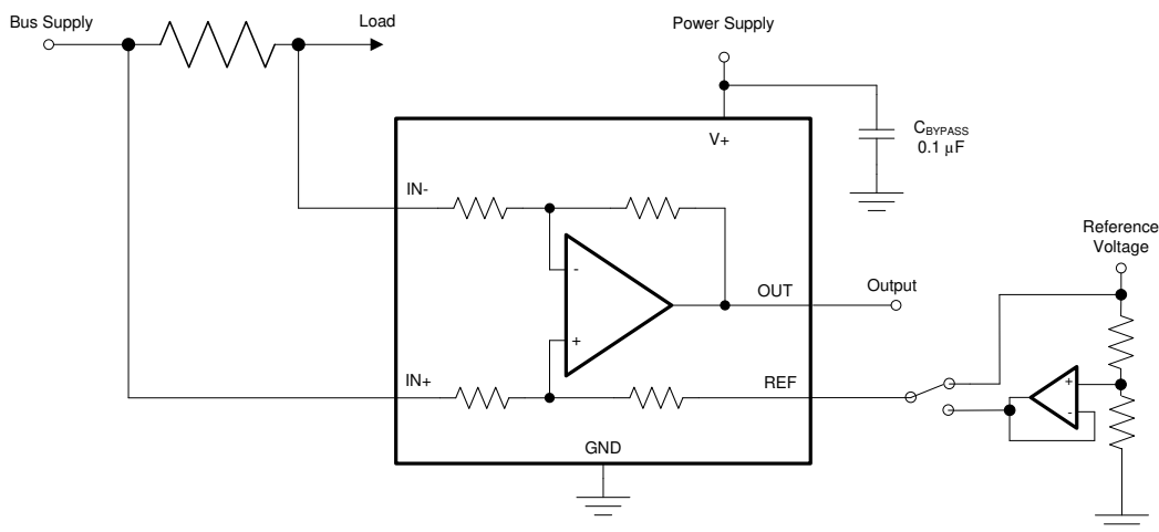
Figure 8-3. Bidirectional Application Schematic
