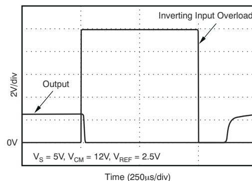
Figure 6-16. Inverting Differential Input Overload
