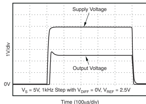
Figure 6-18. Start-Up Response
