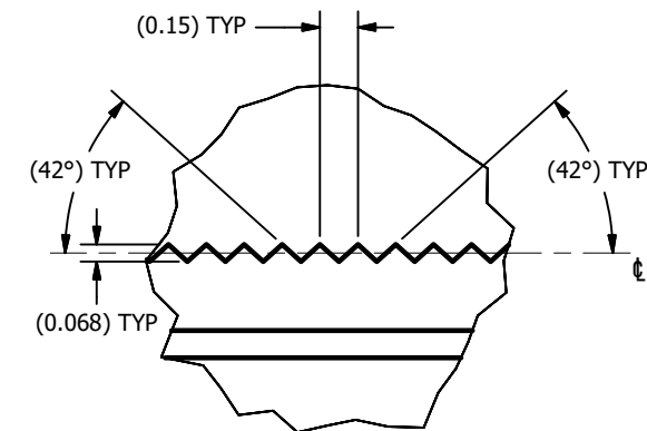
DETAIL F APERTURE TOP AND BOTTOM EDGES (GLASS OMITTED FOR CLARITY) SCALE 60 : 1
