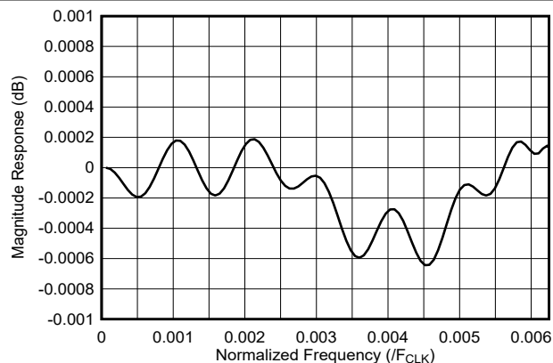
Figure 7-35. 64x Interpolation Filter Passband Response
