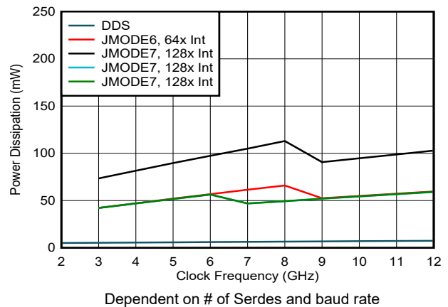
Figure 6-55. VDDT Current vs Clock Frequency and Interface Mode
