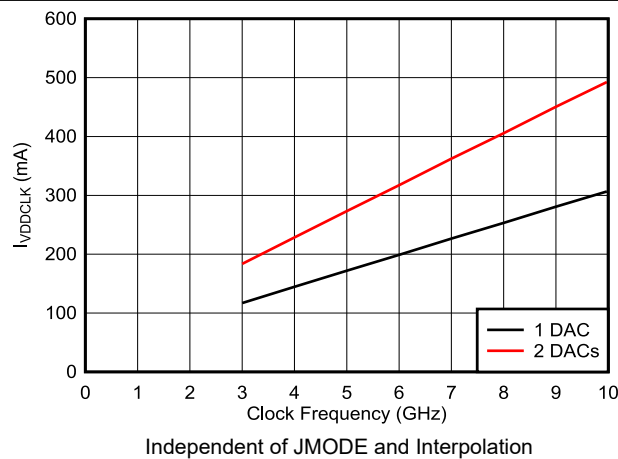
Figure 6-52. VDDCLK Current vs Clock Frequency
