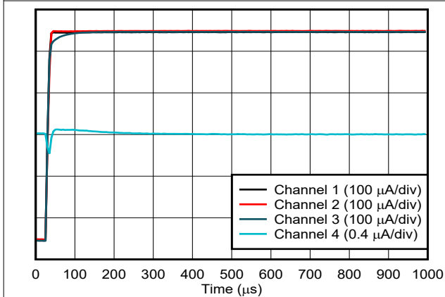
Figure 6-51. Current Output Power-On Glitch
