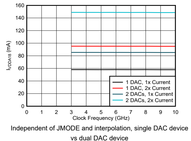
Figure 6-94. VDDA18 Current vs Clock Frequency and DAC Mode
