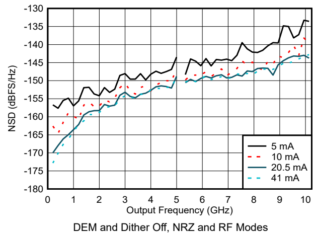
Figure 6-61. NSD vs Output Frequency and Output Current
