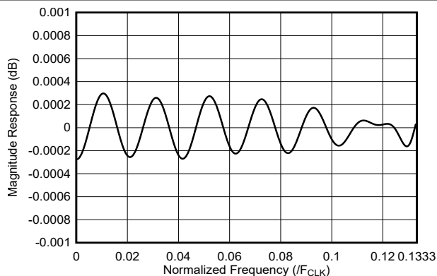
Figure 7-17. 3x Interpolation Filter Passband Response
