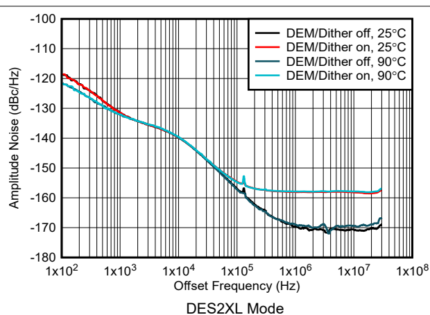
Figure 6-225. Amplitude Noise vs Offset Frequency and Temperature at 1GHz
