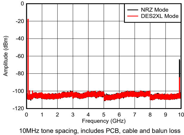
Figure 6-39. Dual Tone, f_{\text{OUT}} = 97\text{ MHz} , -6dBFS (0 - f_{\text{CLK}} )
