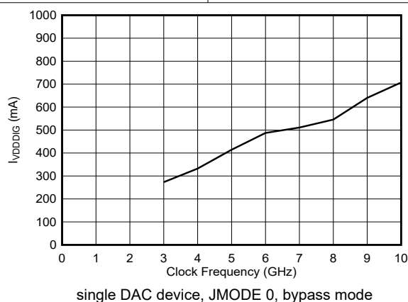
Figure 6-103. VDDDIG Current vs Clock Frequency
