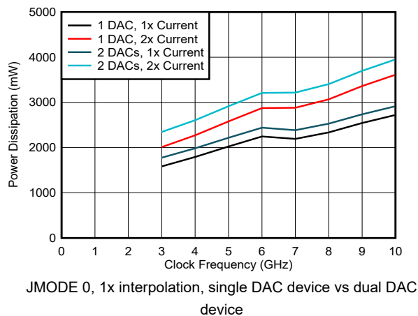
Figure 6-93. Power Dissipation vs Clock Frequency and DAC Mode
