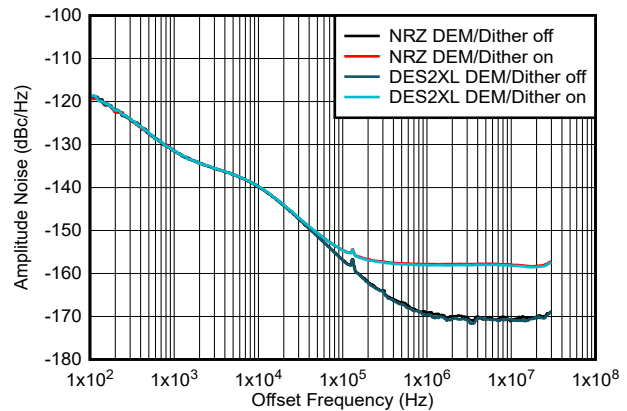
Figure 6-223. Amplitude Noise vs Offset Frequency at 1GHz
