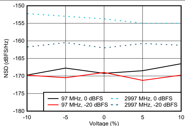
Figure 6-87. NSD vs Supply Voltage
