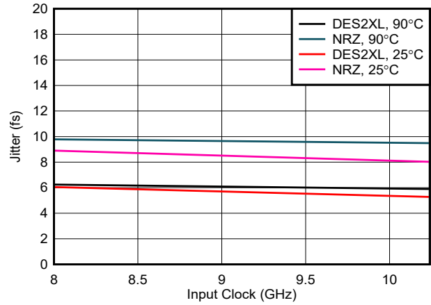
Figure 6-221. Jitter vs Input Clock
