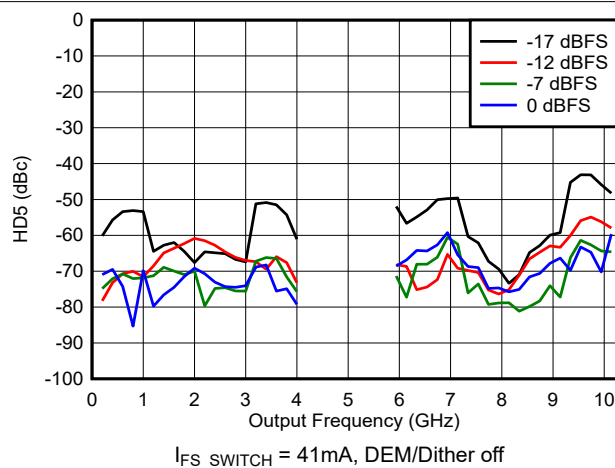
Figure 6-202. HD5 vs Frequency and Digital Amplitude in DES2X Modes
