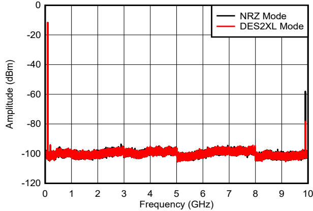
Figure 6-37. Dual Tone, f_{\text{OUT}} = 97\text{ MHz} , 0dBFS (0 - f_{\text{CLK}} )
