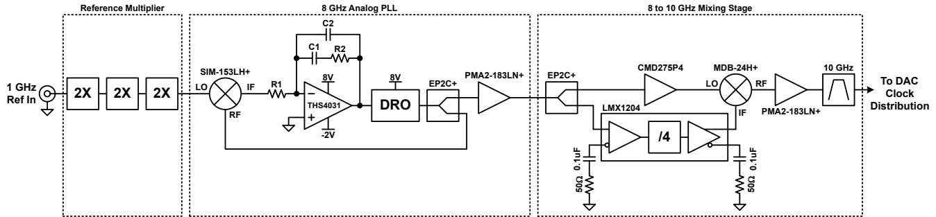
Figure 9-11. 10GHz Clock Synthesizer
