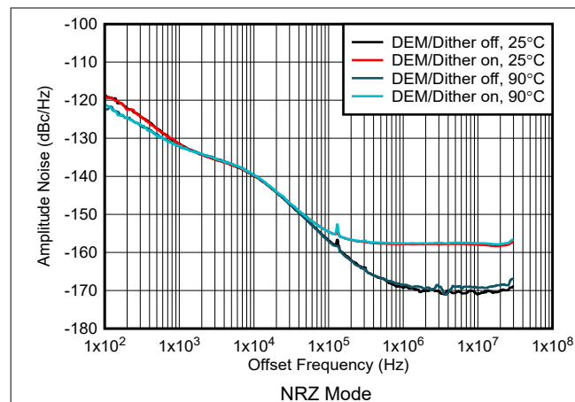
Figure 6-224. Amplitude Noise vs Offset Frequency and Temperature at 1GHz
