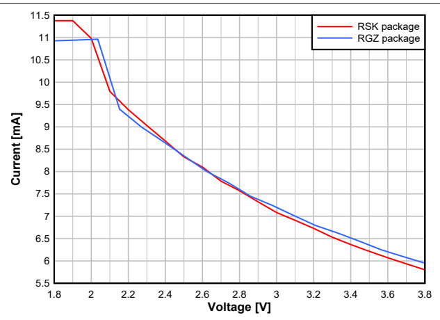
Figure 7-13. TX Current vs. Supply Voltage (VDD5) (BLE 1 Mbps, 2.44GHz, 0dBm)
