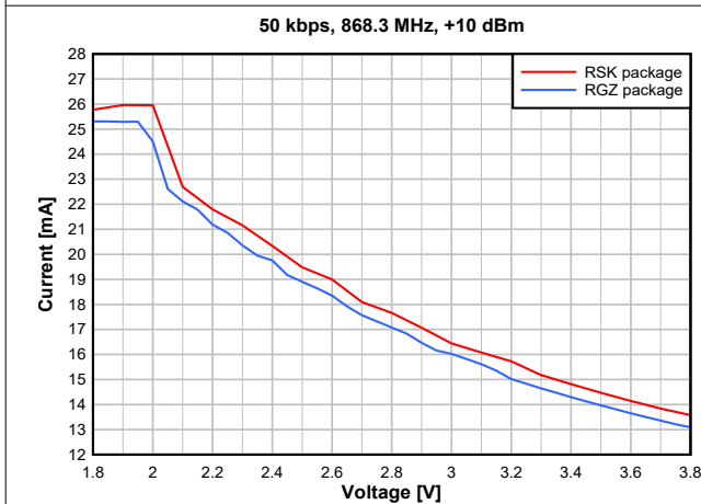
Figure 7-12. TX Current vs. Supply Voltage (VDD5) (50kbps, 868.3MHz)
