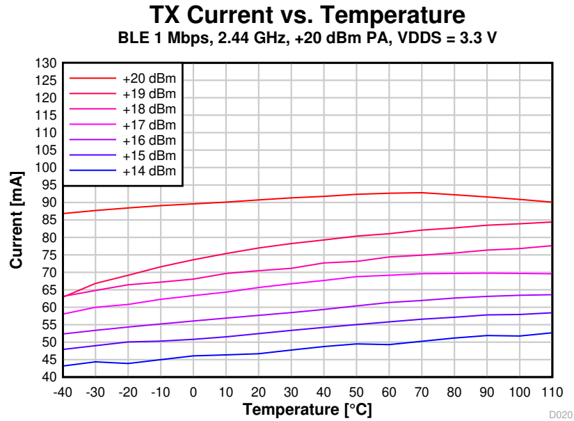
Figure 8-16. TX Current vs. Temperature (BLE 1 Mbps, 2.44 GHz, VDD5 = 3.3 V)
