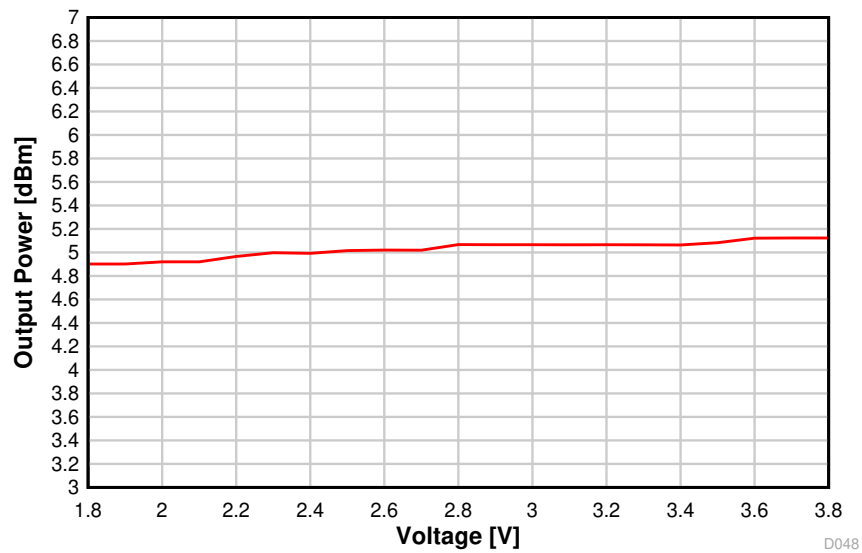
Figure 8-48. Output Power vs. Supply Voltage (VDD5) (BLE 1 Mbps, 2.44 GHz, +5 dBm)
