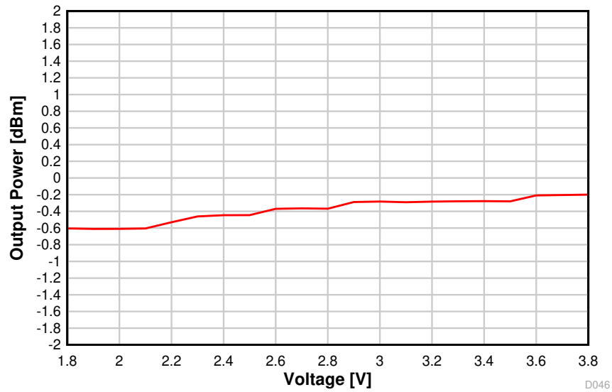
Figure 8-47. Output Power vs. Supply Voltage (VDD5) (BLE 1 Mbps, 2.44 GHz)
