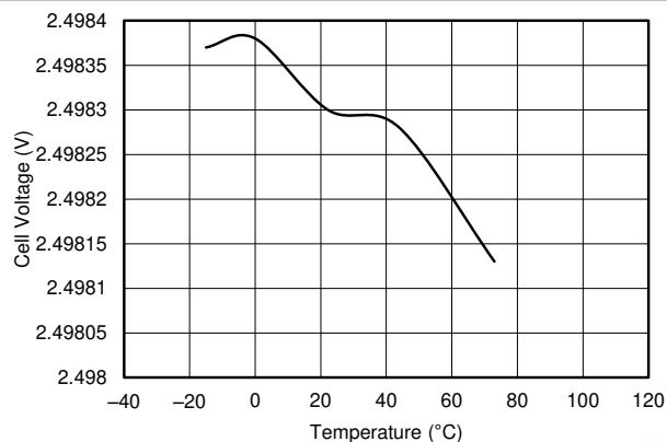
Figure 7-14. V_{\text{CELL}} Measurement at 2.5-V vs. Temperature
