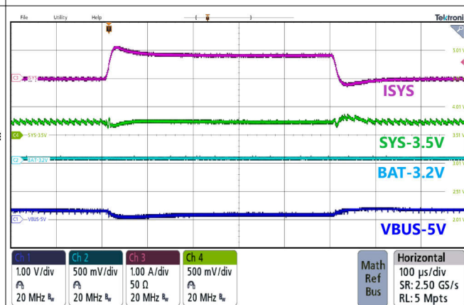
Figure 8-5. Charge Enable
