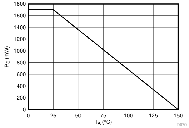
Figure 5-4. Thermal Derating Curve for Safety-Limiting Power Per VDE
