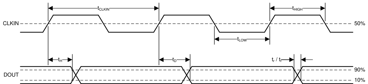
Figure 5-1. Digital Interface Timing
