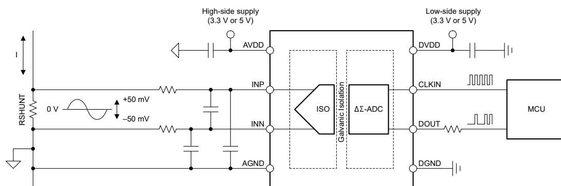
Typical Application
