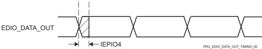
Figure 6-114. PRUSS IEP Digital IOs Timing Requirements
