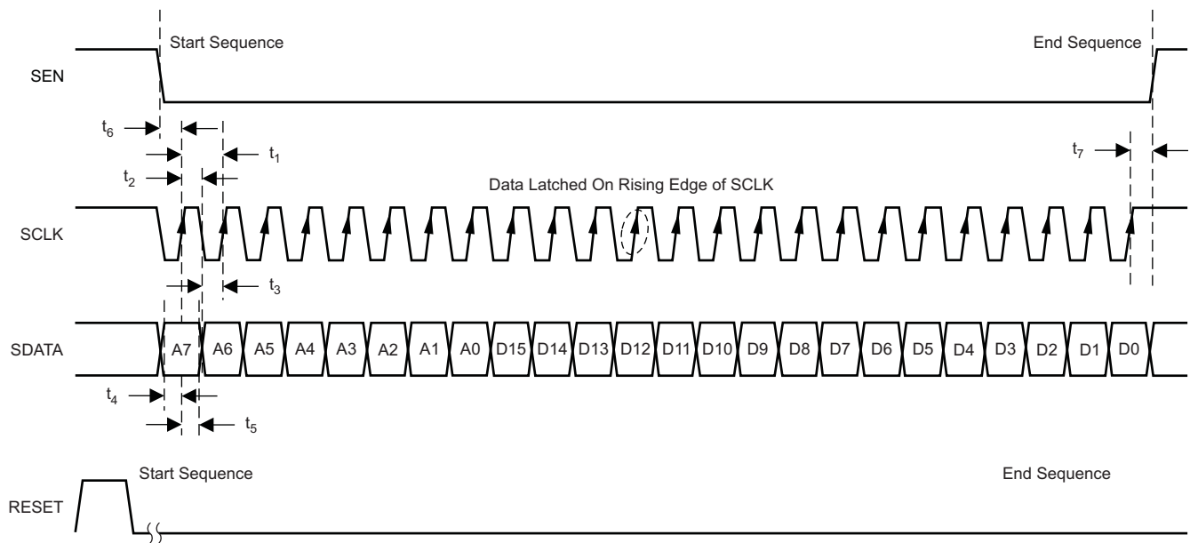
Figure 77. SPI Timing
