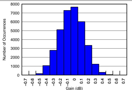
Figure 4. Gain Matching Histogram
