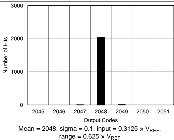
Figure 13. DC Histogram for Mid-Scale Inputs ( 0.625 \times V_{REF} )
