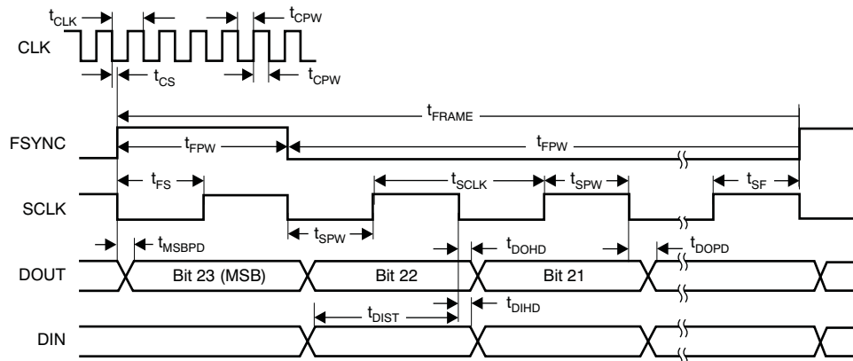
Figure 2. Frame-Sync Format Timing Characteristics
