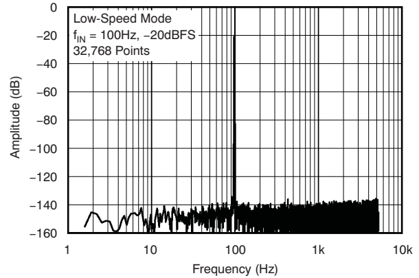
Figure 16. Output Spectrum
