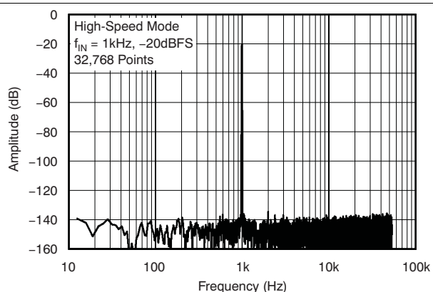
Figure 4. Output Spectrum
