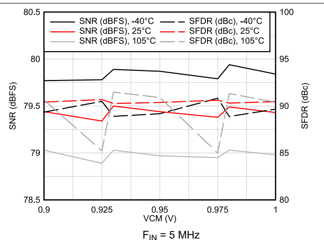
Figure 6-54. AC Performance vs VCM vs Temperature
