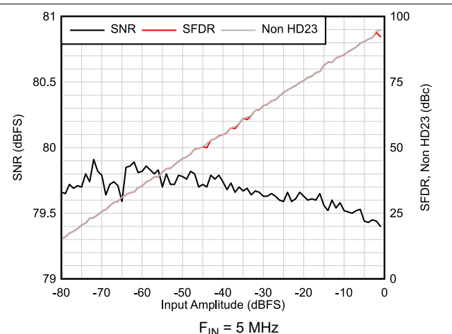
Figure 6-50. AC Performance vs Input Amplitude
