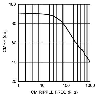
Figure 37. Analog Input CMRR vs. Frequency
