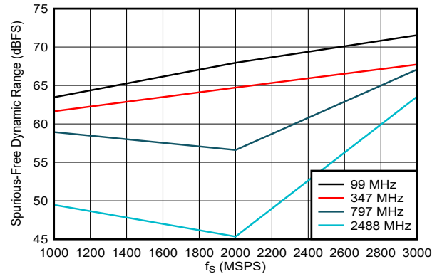
Figure 5-117. SFDR vs Sampling Rate
