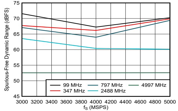
Figure 5-229. SFDR vs Sampling Rate
