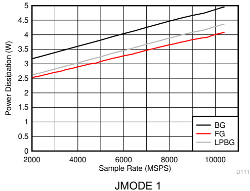
Figure 5-127. DES Mode: Power Dissipation vs Sample Rate
