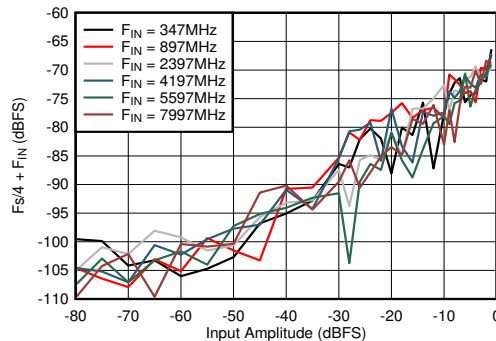
Figure 5-67. DES Mode: F_s/4 + F_{\text{IN}} vs Input Amplitude and Frequency
