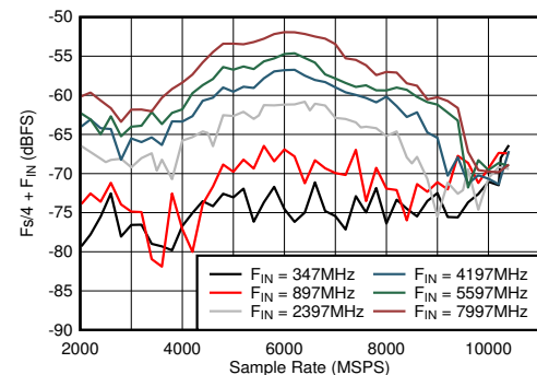
Figure 5-42. DES Mode: \text{Fs}/4 + F_{\text{IN}} vs Sample Rate and Input Frequency
