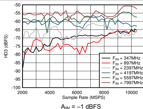
Figure 5-38. DES Mode: HD3 vs Sample Rate and Input Frequency
