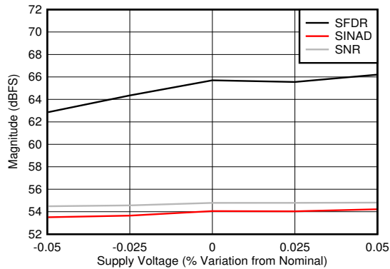
Figure 5-95. Dual Channel Mode: SNR, SINAD and SFDR vs Supply Voltage
