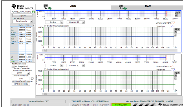
Figure 7-10. Idle-Channel Noise (No Input) for 2.5-GSPS, Dual-Channel Oscilloscope
