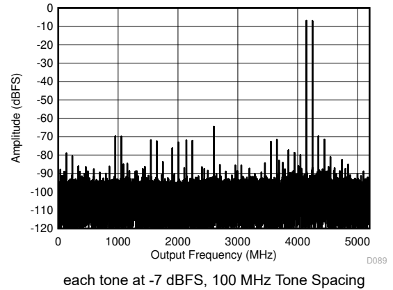
Figure 5-14. DES Mode: Two Tone FFT at 4197 MHz
