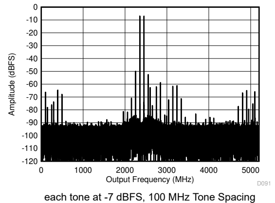
Figure 5-16. DES Mode: Two Tone FFT at 7997 MHz
