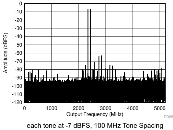
Figure 5-13. DES Mode: Two Tone FFT at 2397 MHz
