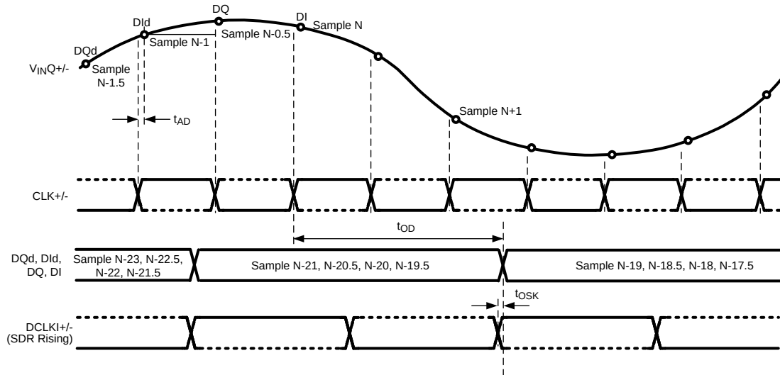
Figure 4-5. Clocking in 1:4 Demux DES Mode*
