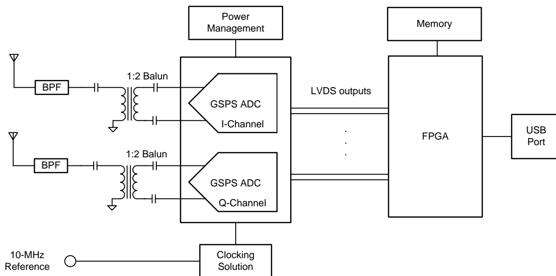
Figure 72. Simplified Schematic
