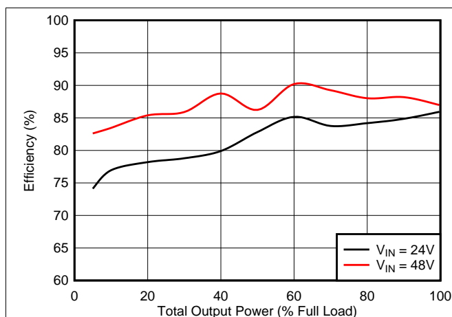
Figure 52. Efficiency
