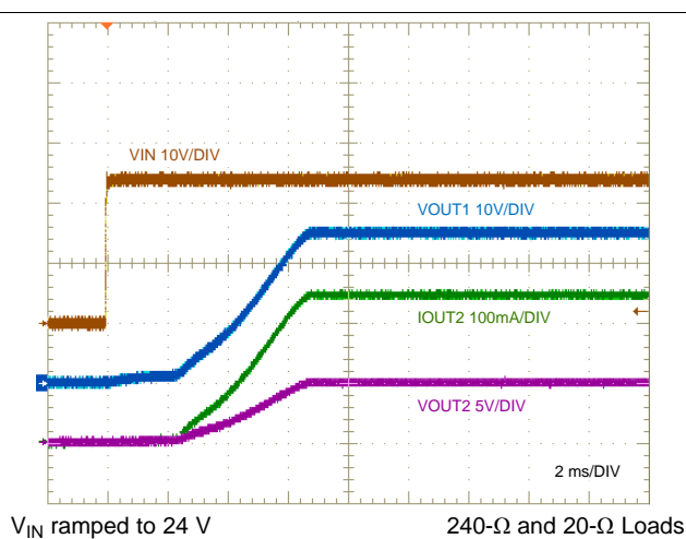
Figure 53. Start-Up Characteristic
