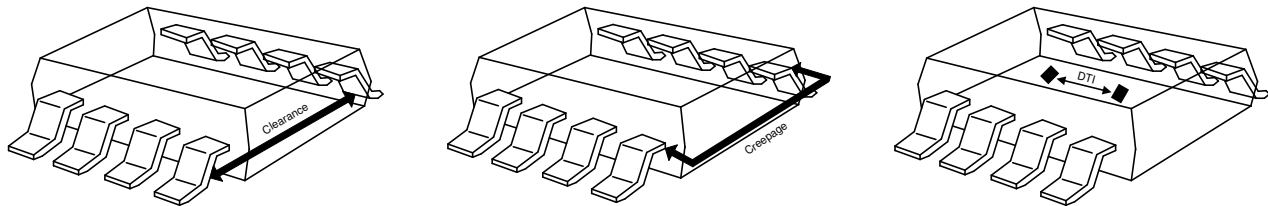
Figure 1-1. Clearance, Creepage, and DTI
