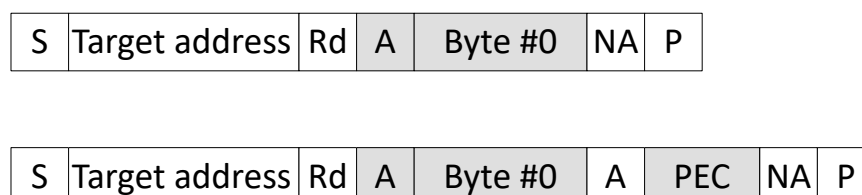
Figure 34-17. Receive Byte Message With and Without PEC
