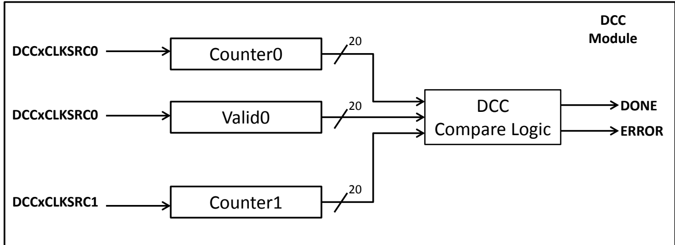
Figure 11-2. DCC Operation
