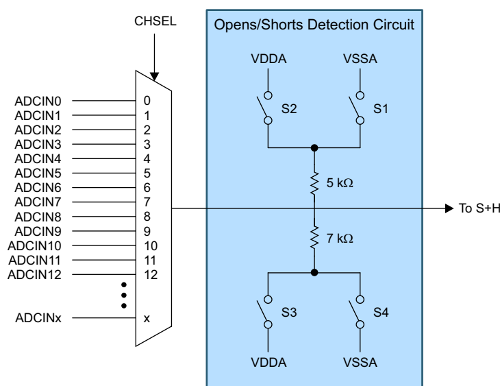
Figure 22-30. Opens/Shorts Detection Circuit
