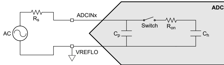
Figure 22-11. Single-Ended Input Model
