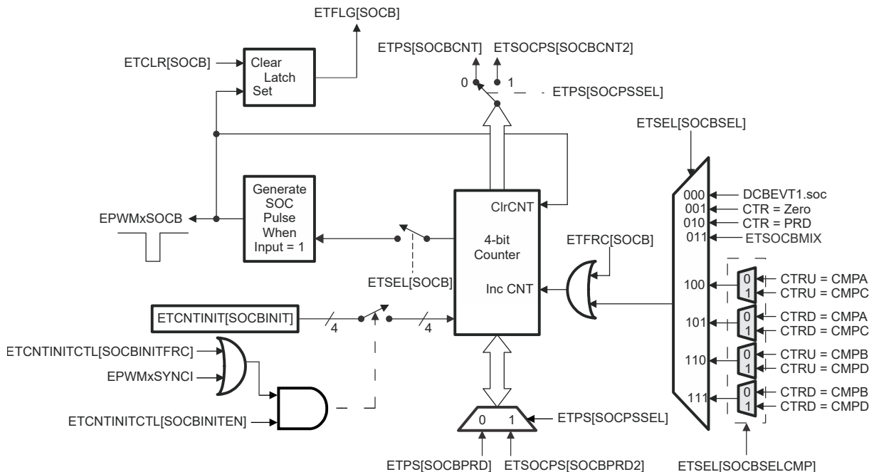
Figure 27-73. Event-Trigger SOCB Pulse Generator
