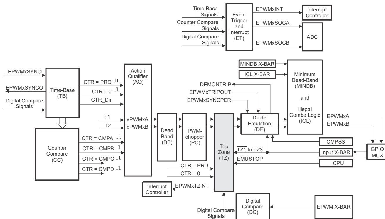
Figure 27-48. Trip-Zone Submodule
