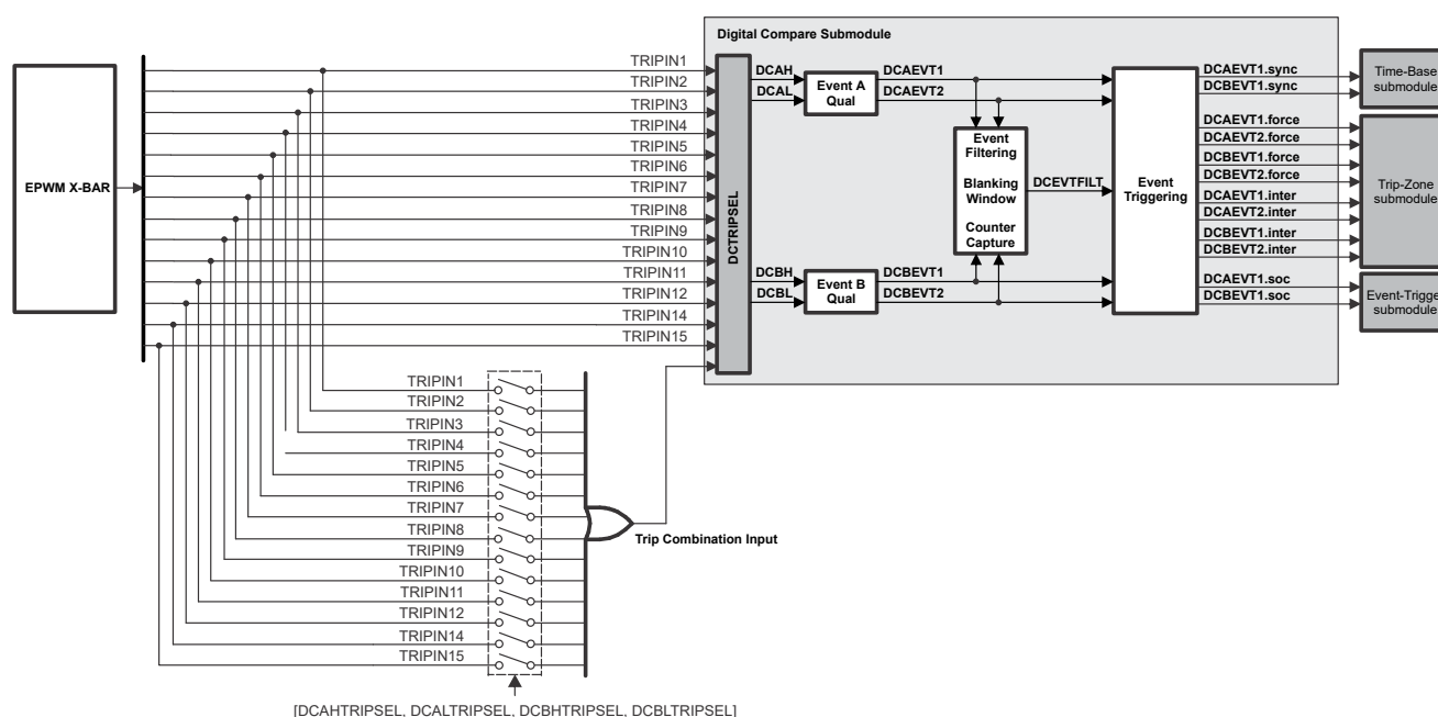
Figure 27-74. Digital-Compare Submodule High-Level Block Diagram
