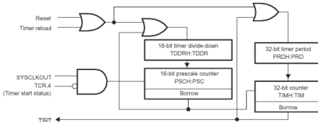
Figure 2-12. CPU Timers
