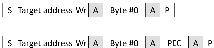
Figure 34-16. Send Byte Message With and Without PEC
