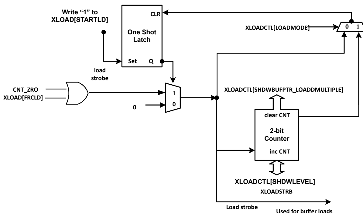
Figure 27-38. Global Load: Signals and Registers
