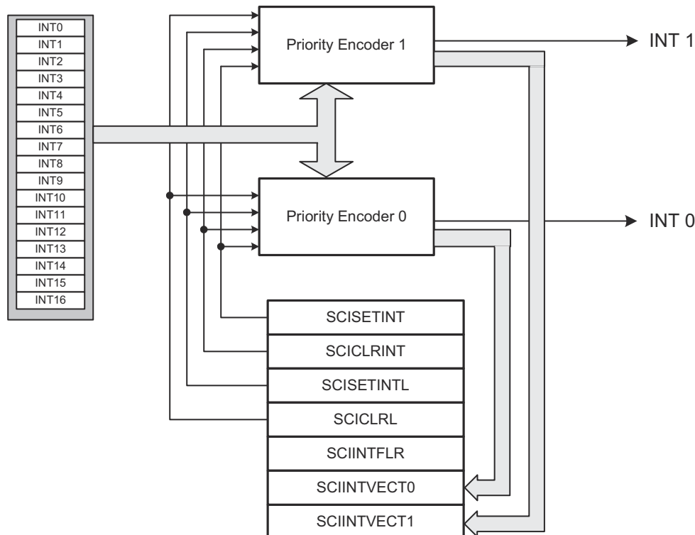
Figure 36-10. General Interrupt Scheme
