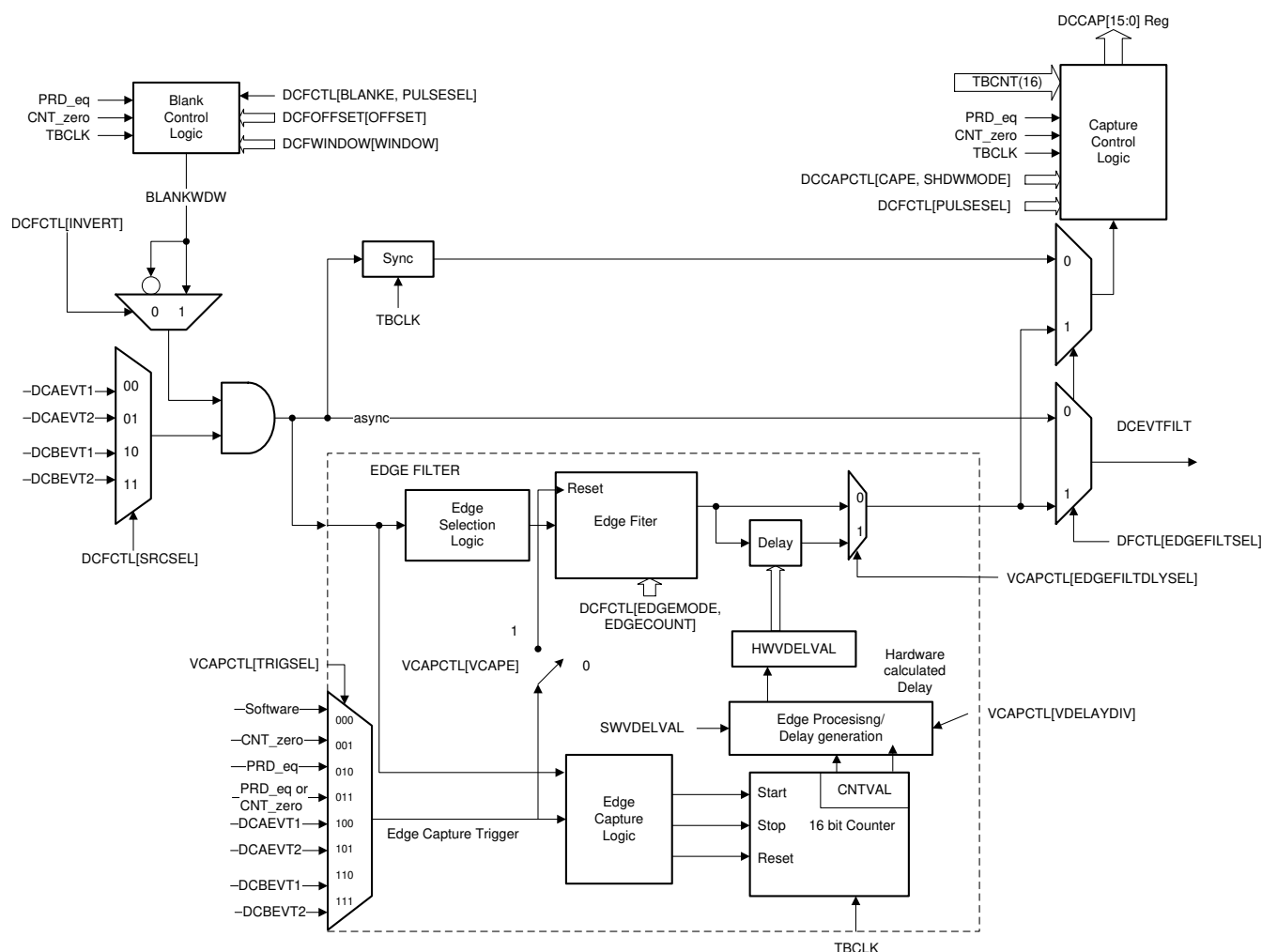
Figure 27-81. Valley Switching
