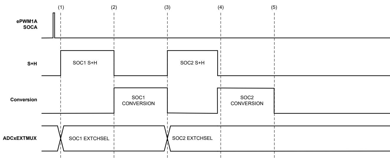
Figure 22-15. ADC External Channel Select Timing Example
