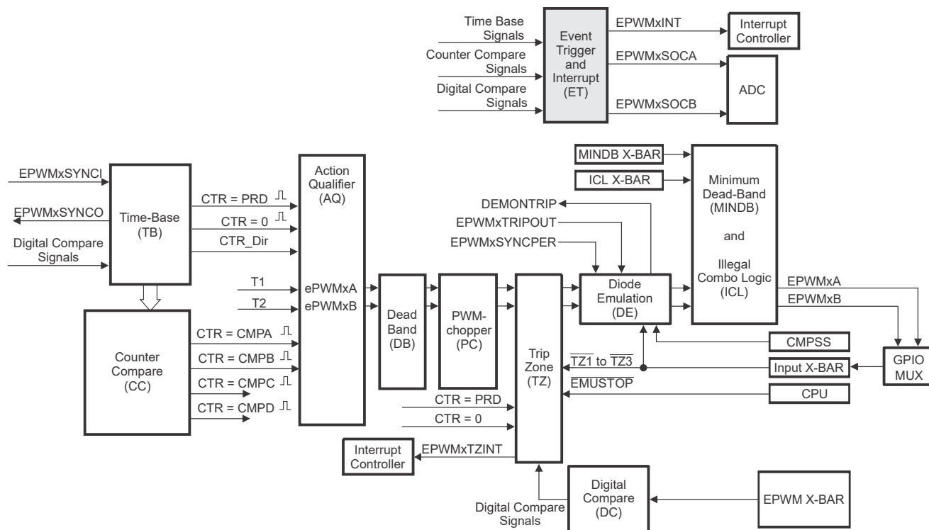
Figure 27-69. Event-Trigger Submodule
