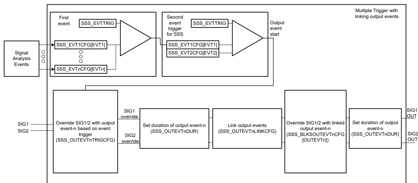
Figure 18-11. Linking Output Events for Generating Pattern Output Events
