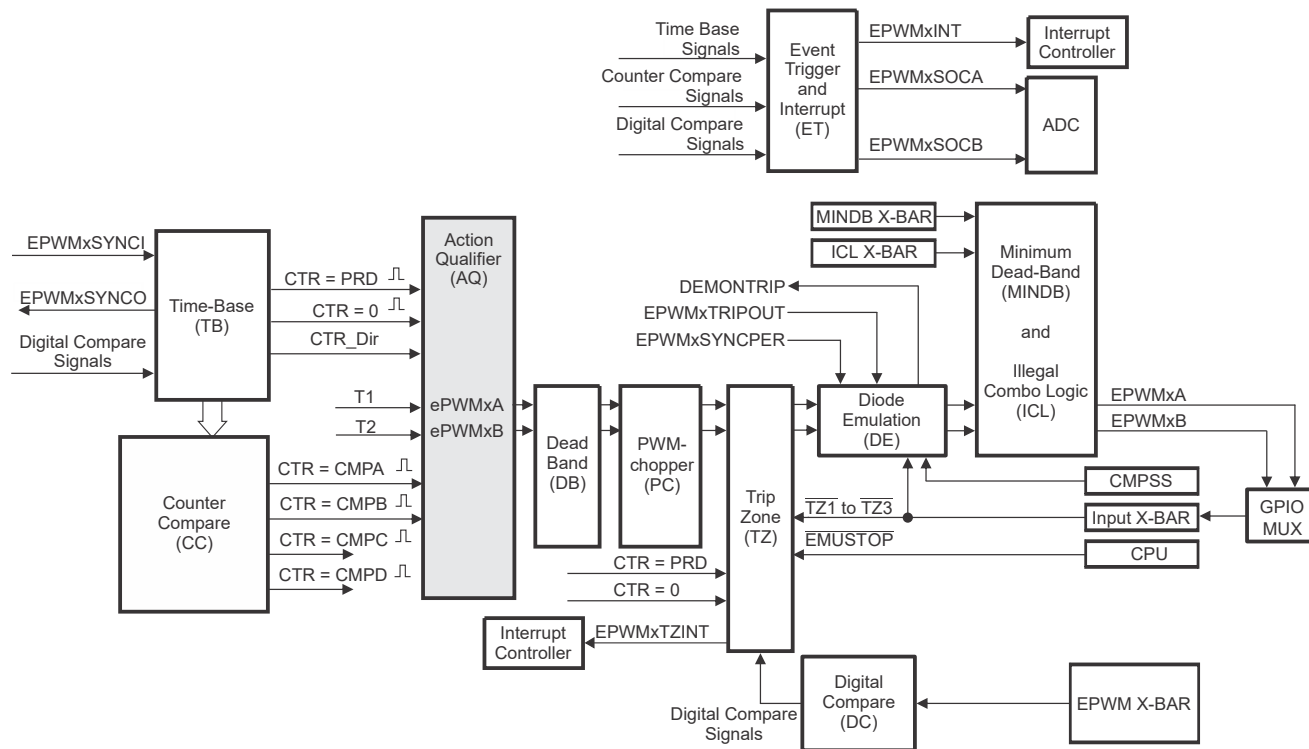
Figure 27-21. Action-Qualifier Submodule
