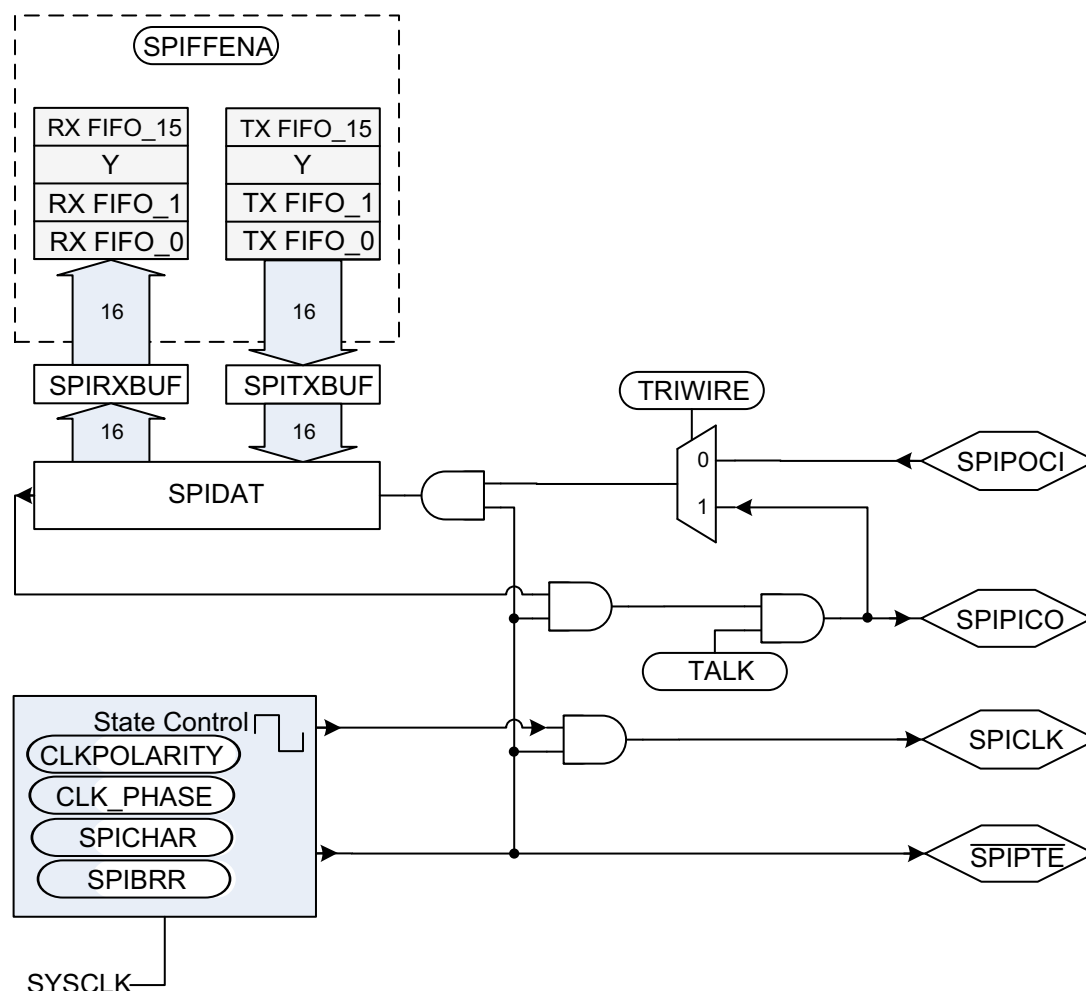
Figure 37-5. SPI Module Controller Configuration
