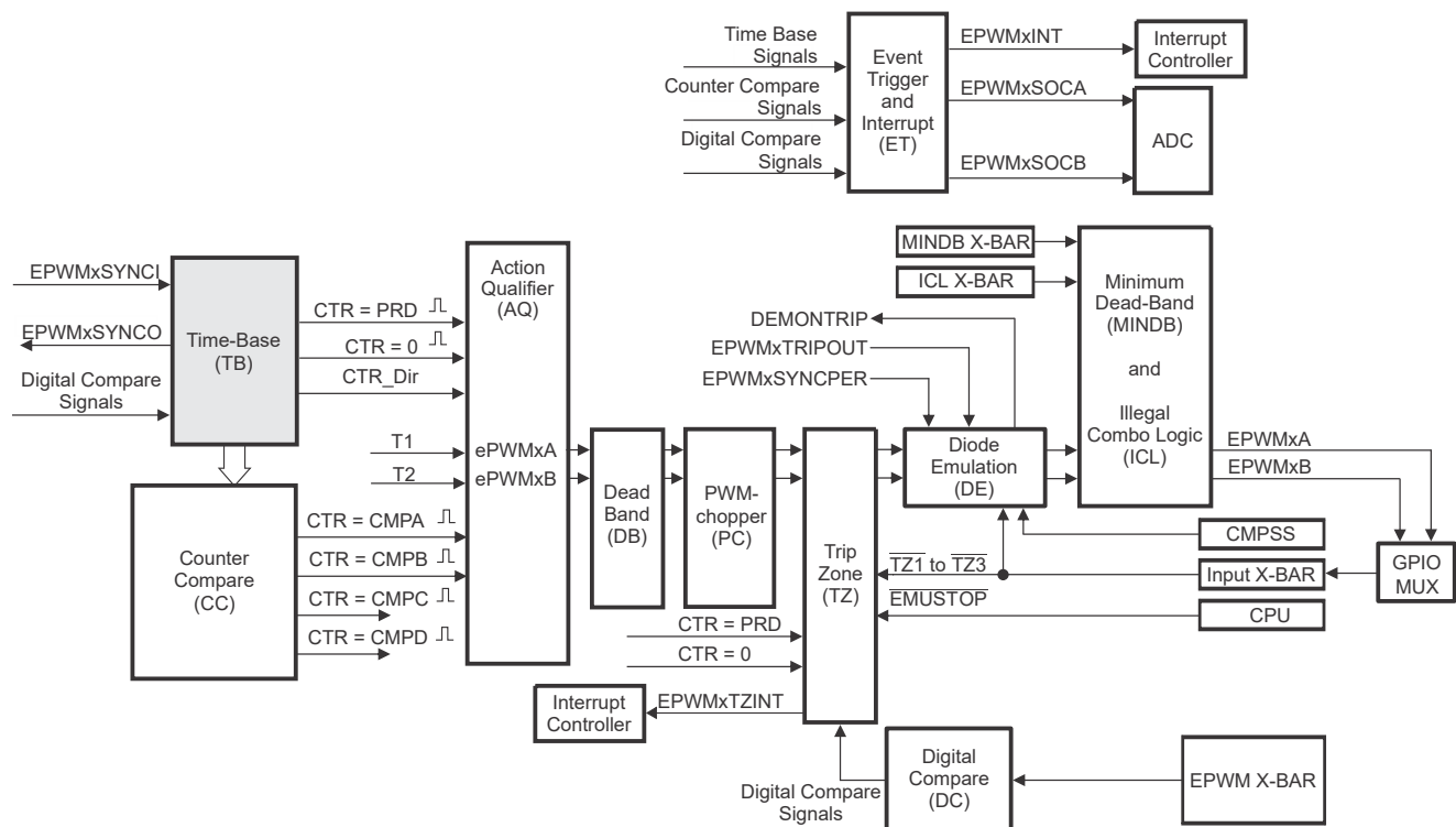
Figure 27-4. Time-Base Submodule
