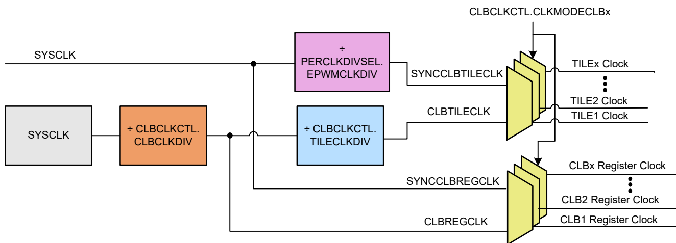
Figure 10-3. CLB Clocking
