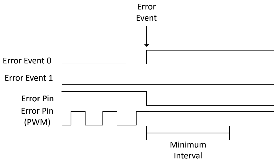
Figure 7-9. ESM Error Pin Assertion
