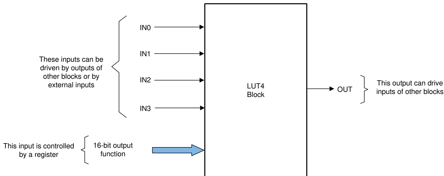
Figure 10-16. LUT4 Block
