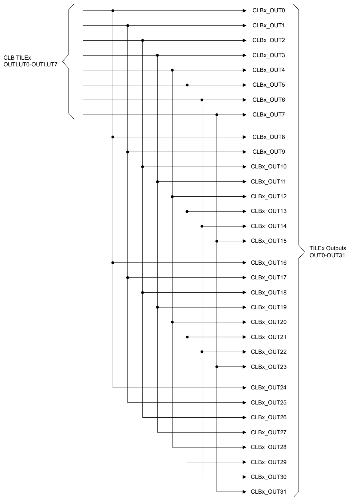
Figure 10-9. CLB Outputs
