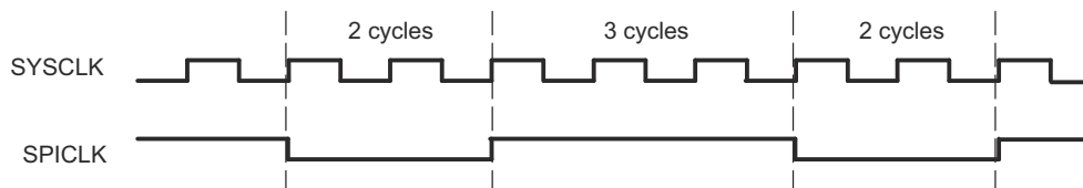
Figure 37-8. SPI: SPICLK-SYSCLOCK Characteristic when (BRR + 1) is Odd, BRR > 3 , and CLKPOLARITY = 1
