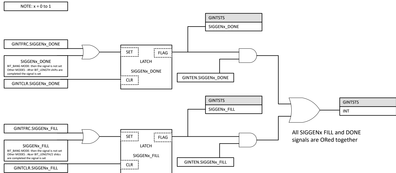
Figure 20-7. EPG Interrupt
