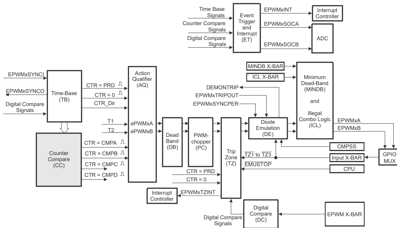
Figure 27-15. Counter-Compare Submodule
