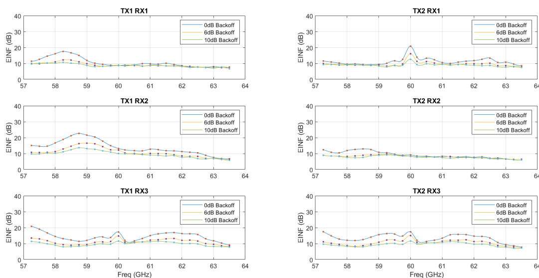
Figure 2-1. EINF With Single TX on Across Frequencies
