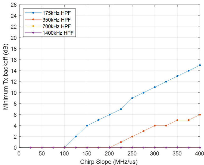
Figure 4-3. Minimum TX Backoff for 61 to 63.5GHz
