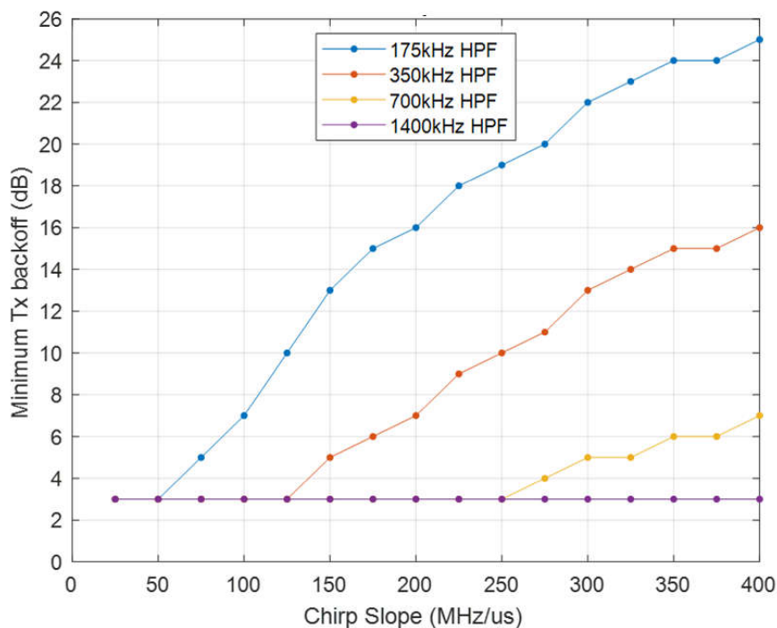
Figure 4-2. Minimum TX Backoff for 57 to 63.5GHz
