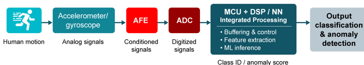
Figure 4. Signal-chain block diagram for a gesture-recognition wearable application
