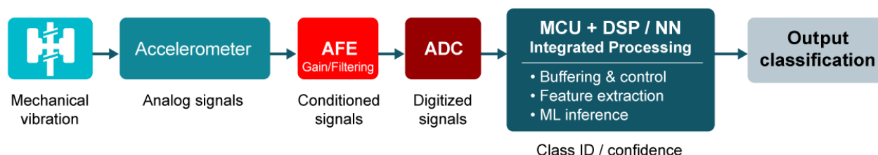
Figure 6. Signal-chain block diagram for mechanical vibration monitoring in an industrial motor
