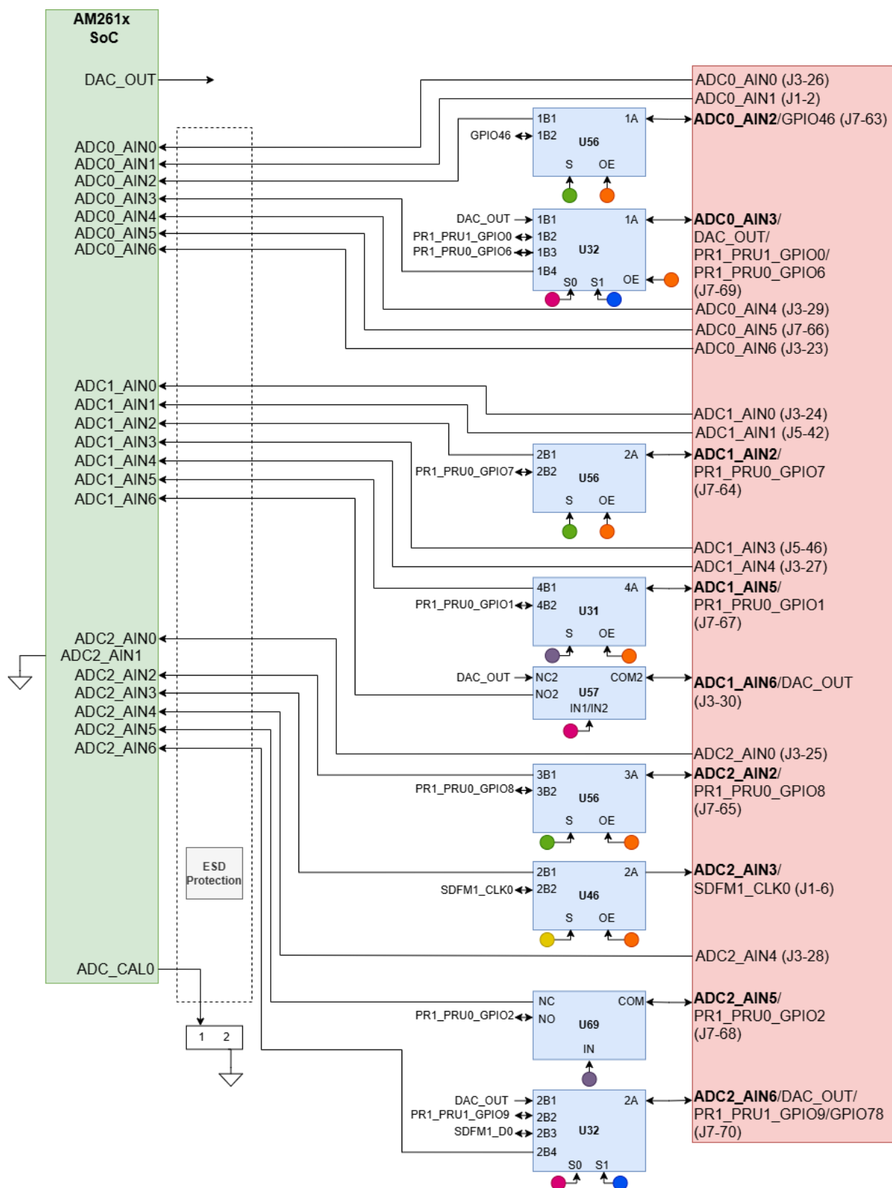
Figure 2-30. ADC/DAC Interface
