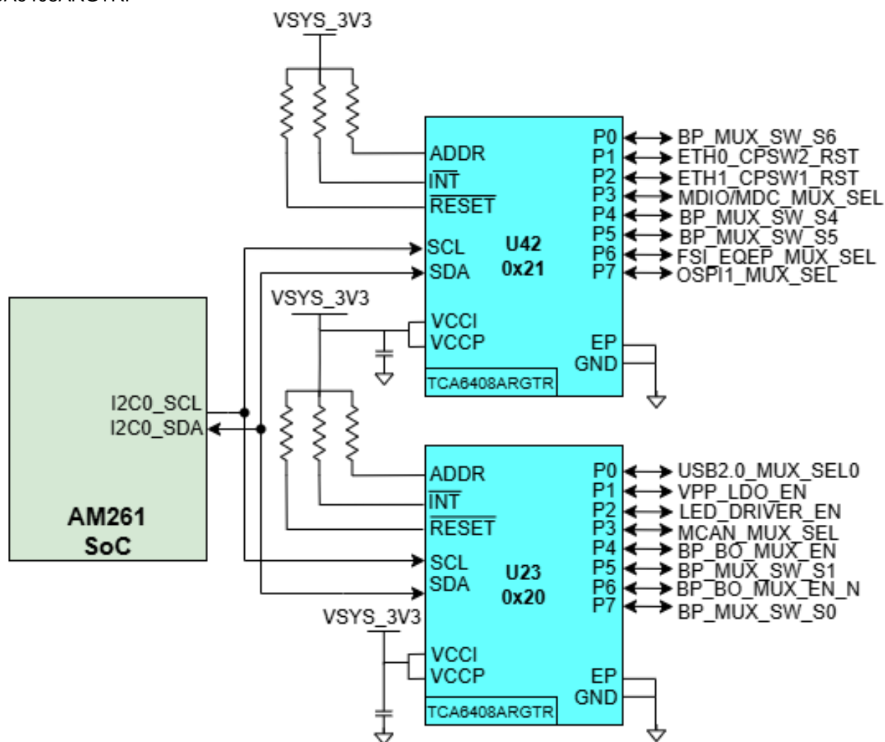
Figure 2-12. IO Expander
