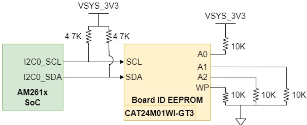
Figure 2-16. Board ID EEPROM
