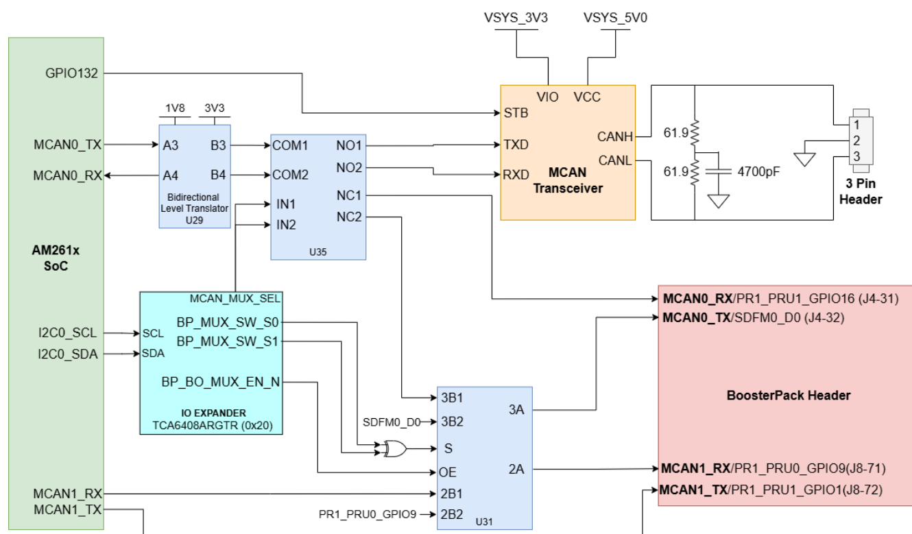
Figure 2-23. LP-AM261x MCAN Interface
