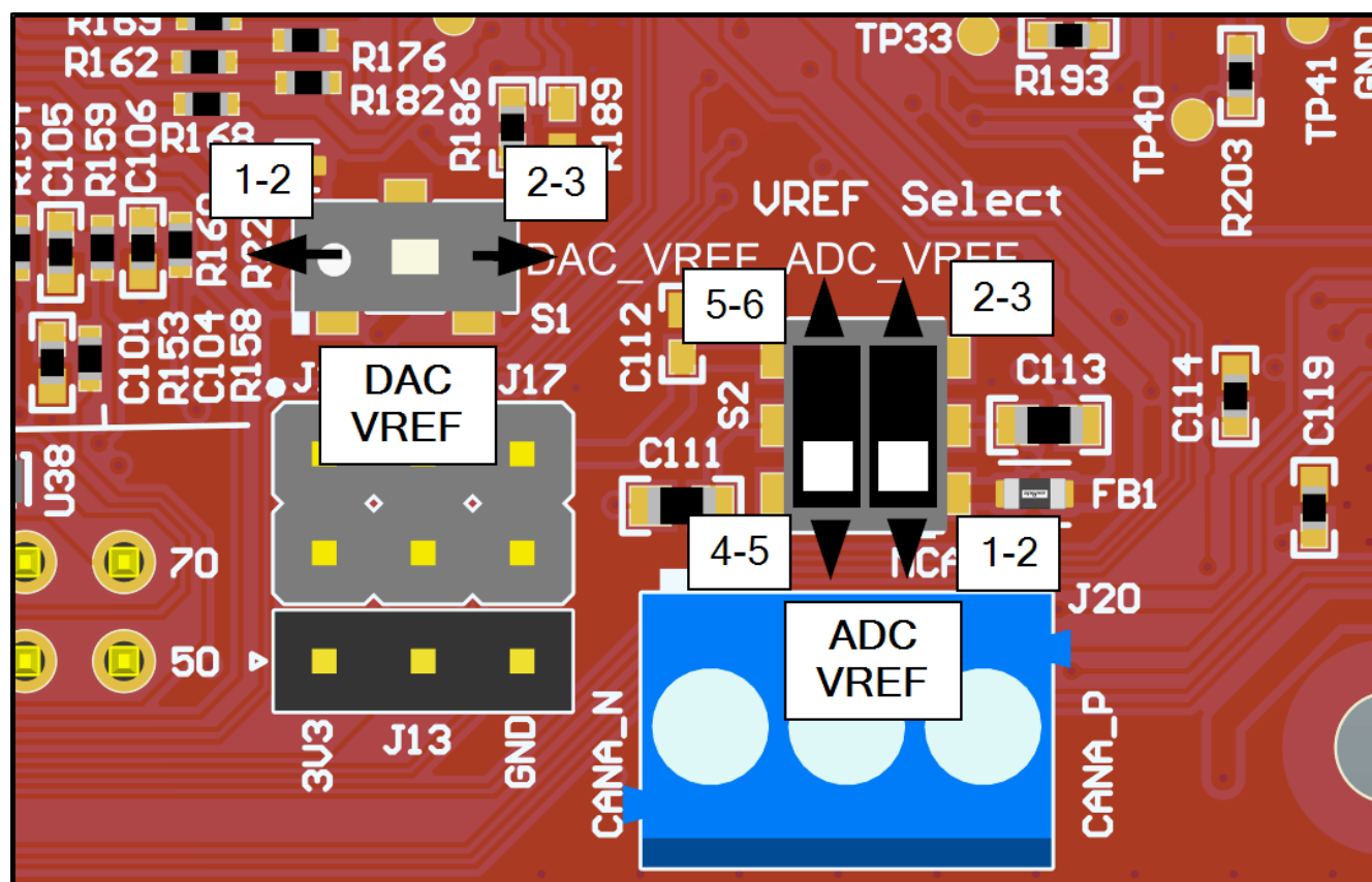
Figure 2-32. LP-AM261 ADC/DAC VREF Switches
