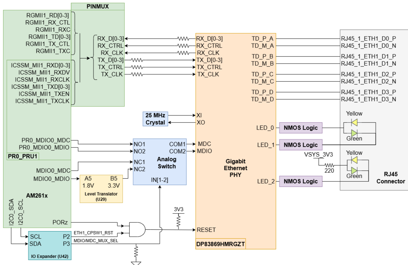
Figure 2-18. Ethernet PHY 1
