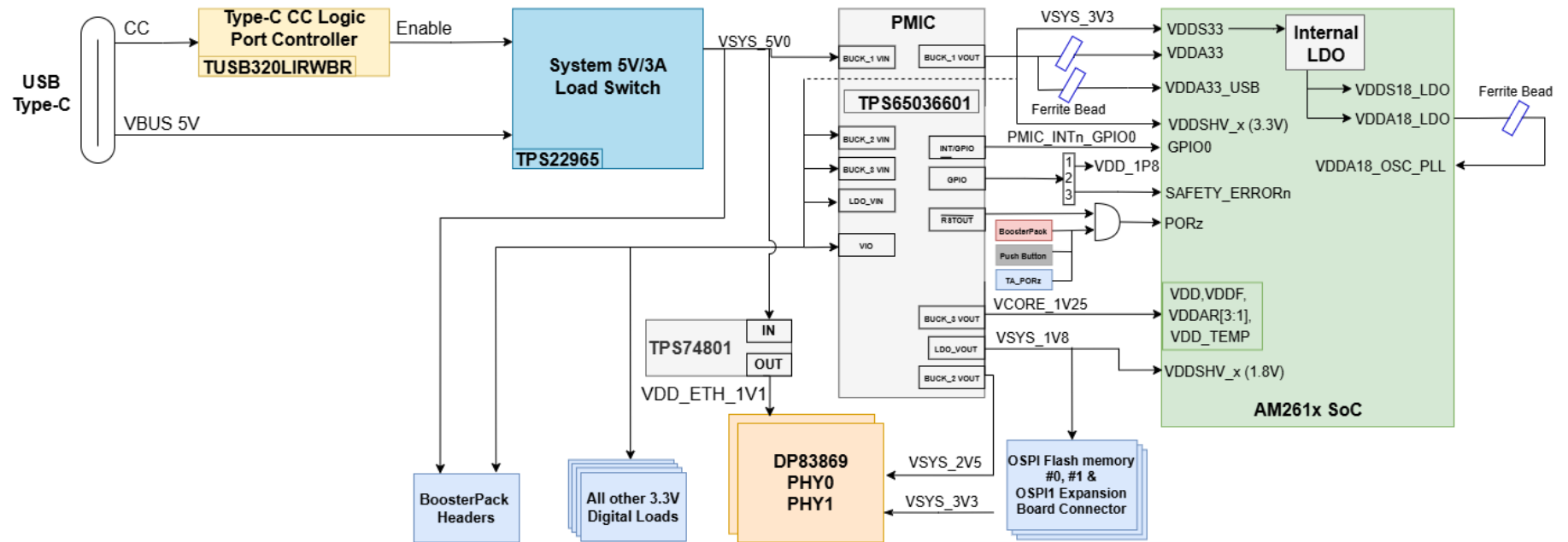
Figure 2-4. Power Tree Diagram of AM261x LaunchPad
