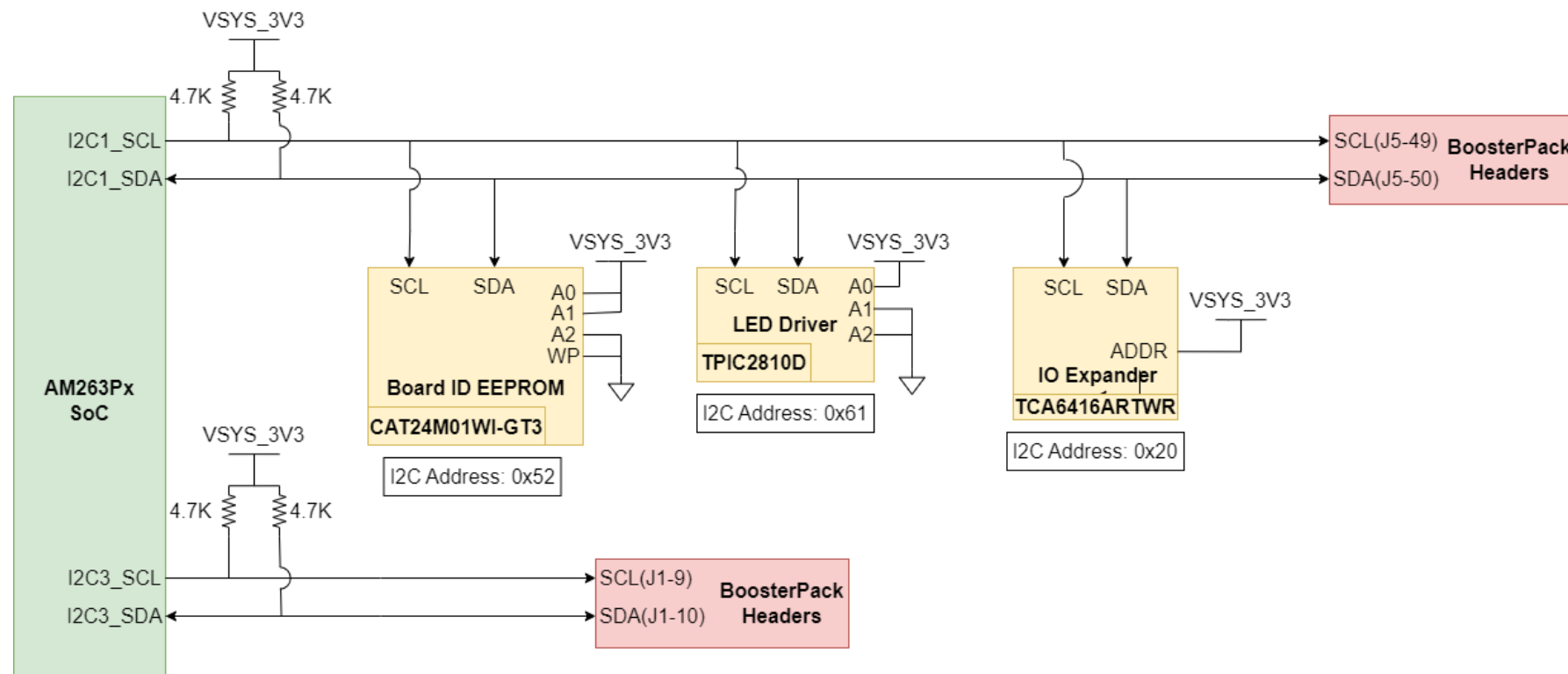
Figure 2-18. I2C Targets
