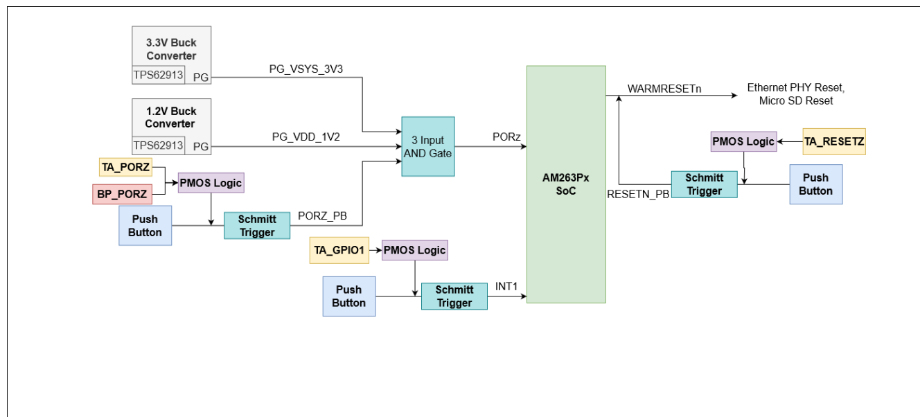
Figure 2-9. Reset Architecture
