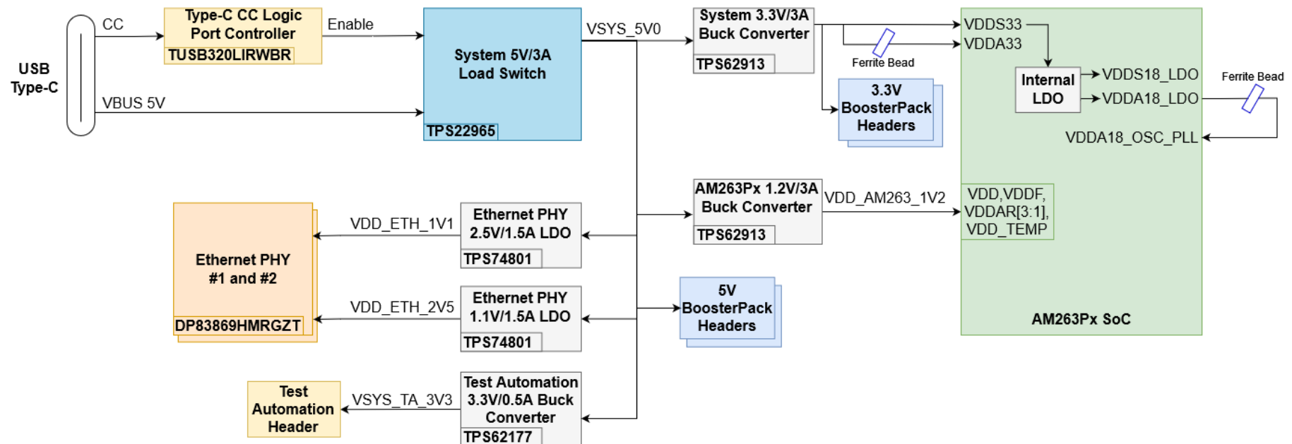
Figure 2-4. Power Tree Diagram of AM263Px LaunchPad
