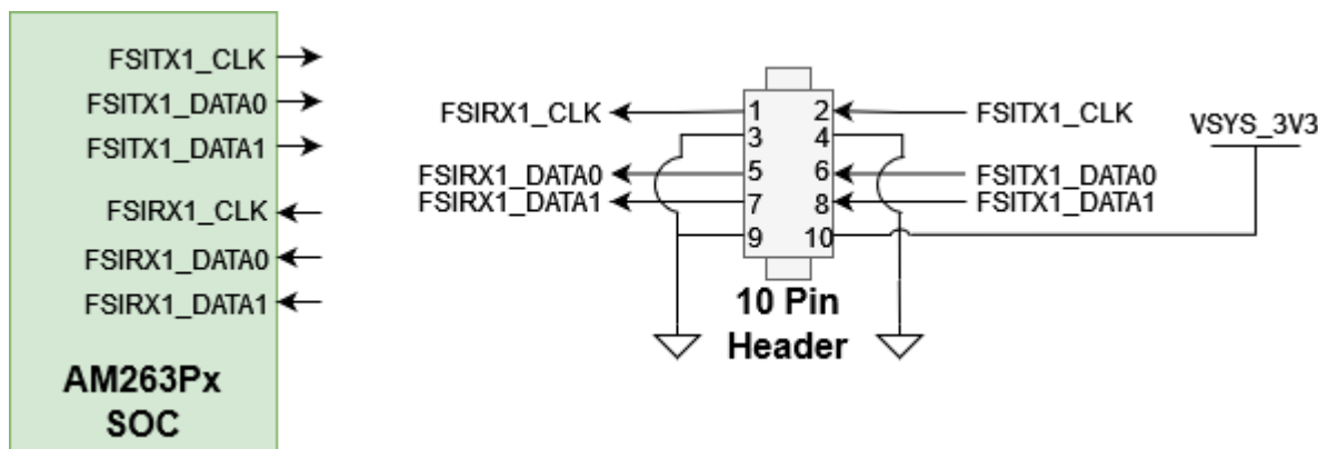
Figure 2-24. FSI 10-Pin Header
