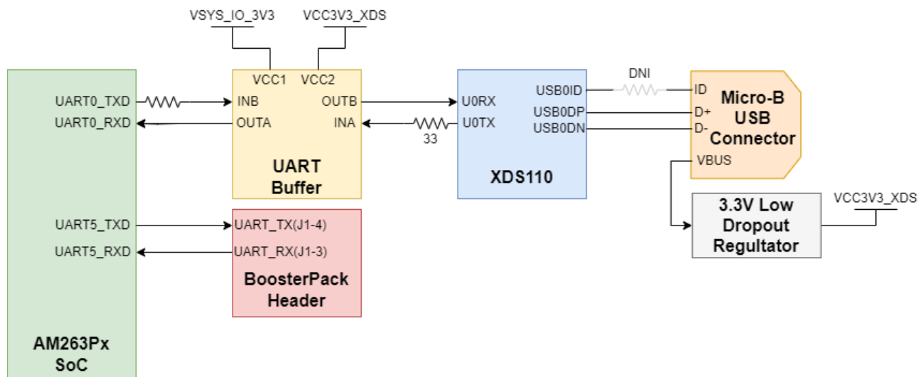
Figure 2-22. UART
