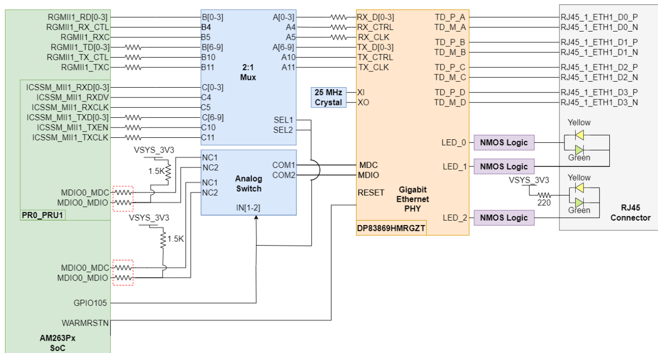
Figure 2-16. Ethernet PHY #1
