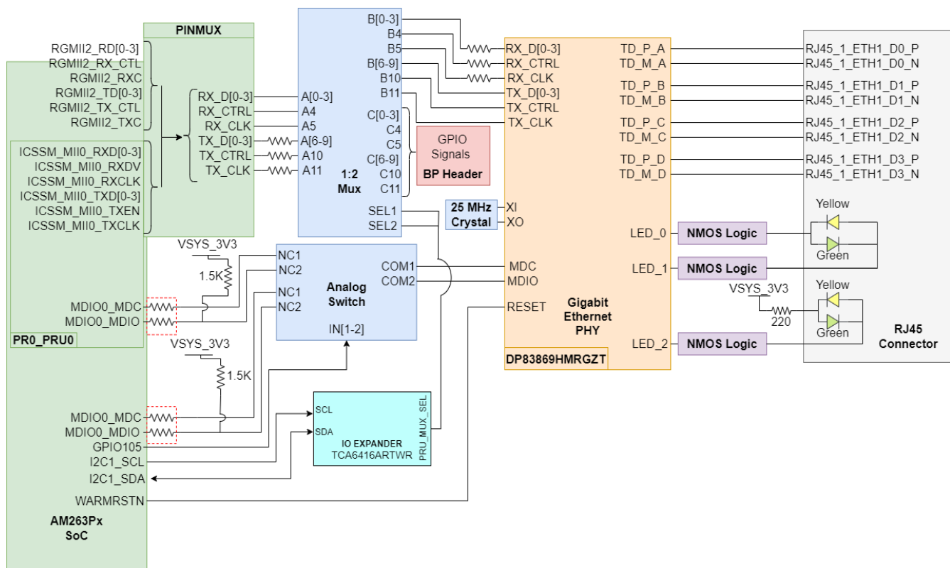
Figure 2-17. Ethernet PHY #2
