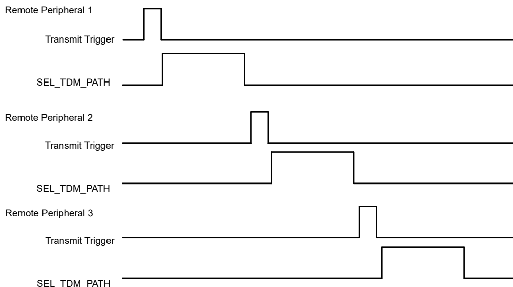
Figure 32-12. Generated Signals for FSI Multi-Node TDM Configuration
