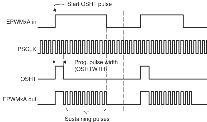
Figure 27-46. PWM Chopper Submodule Waveforms Showing the First Pulse and Subsequent Sustaining Pulses
