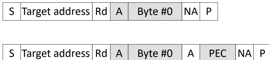
Figure 34-4. Receive Byte Message With and Without PEC
