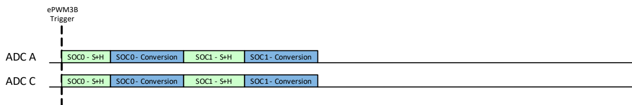
Figure 22-36. Example: Basic Synchronous Operation
