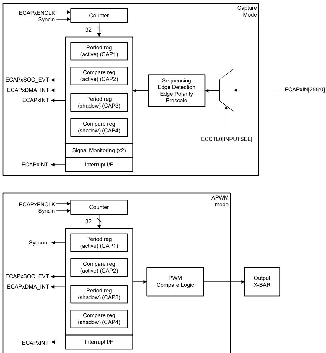
Figure 25-1. Capture and APWM Modes of Operation
