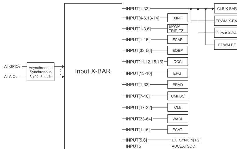
Figure 19-1. Input X-BAR
