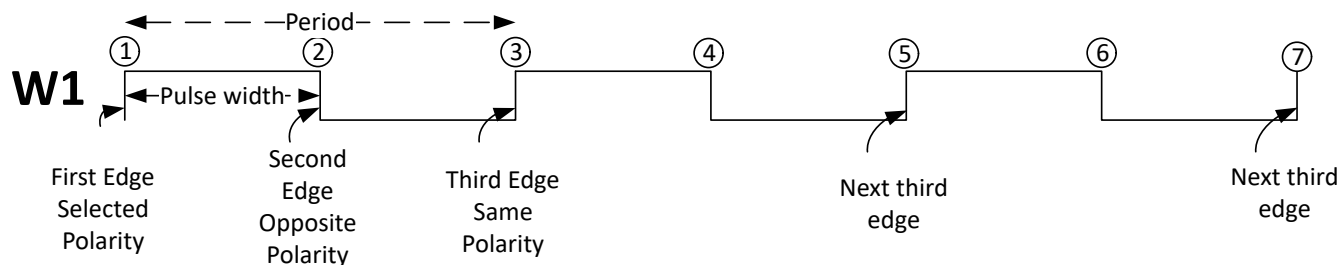
Figure 18-3. Pulse Width Diagram
