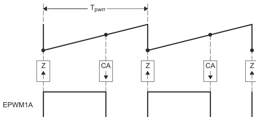
Figure 27-119. PWM Waveform Generated for Simple Buck Controlled Converter
