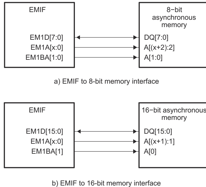
Figure 13-9. EMIF to 8-bit/16-bit Memory Interface
