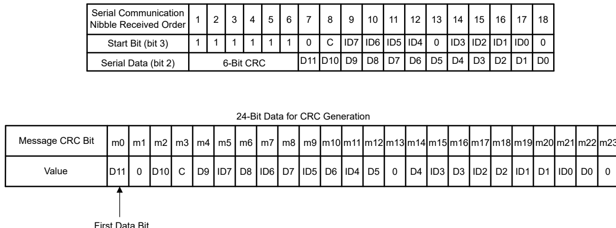
Figure 38-7. Enhanced Serial Message Data Order for CRC Generation
