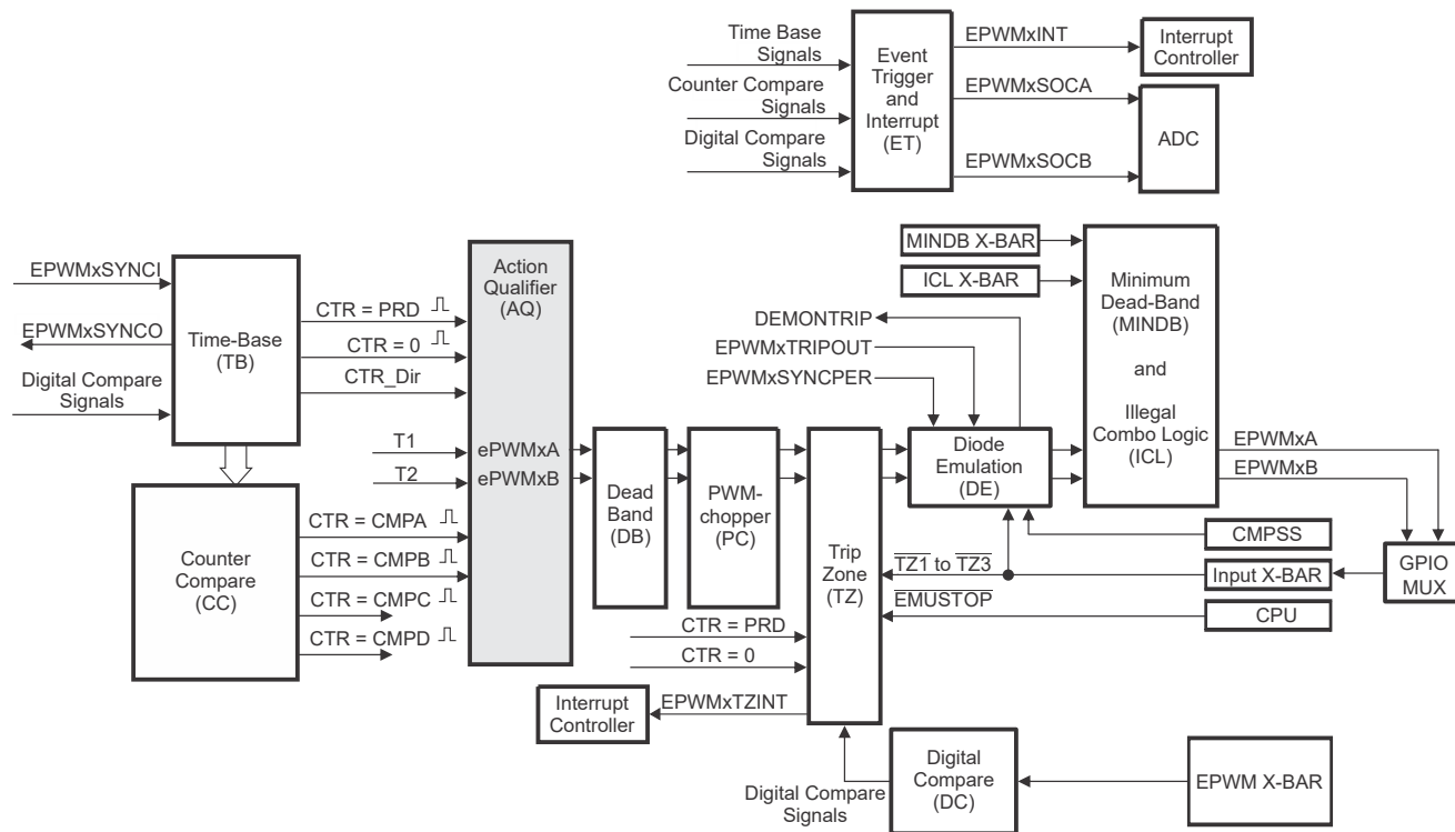
Figure 27-21. Action-Qualifier Submodule
