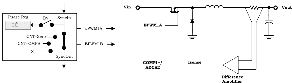
Figure 27-104. Peak Current Mode Control of Buck Converter
