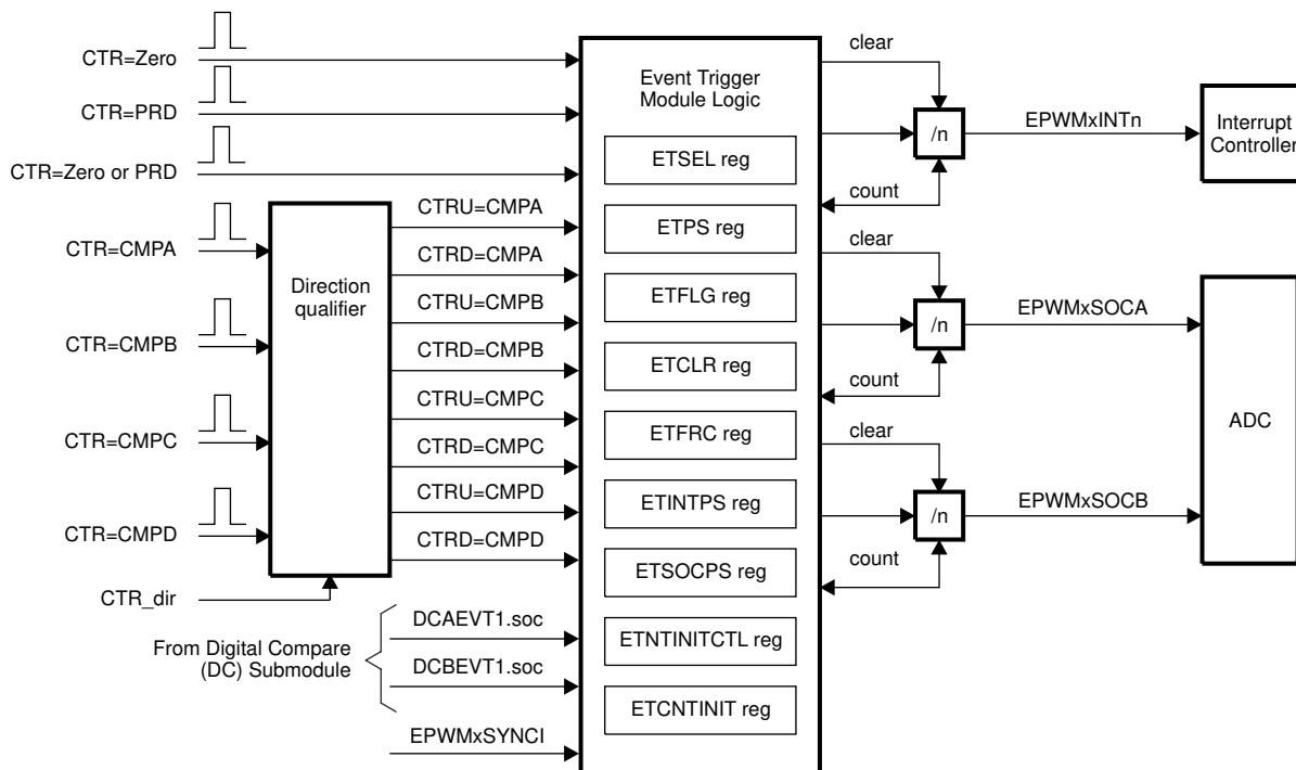
Figure 27-70. Event-Trigger Submodule Showing Event Inputs and Prescaled Outputs
