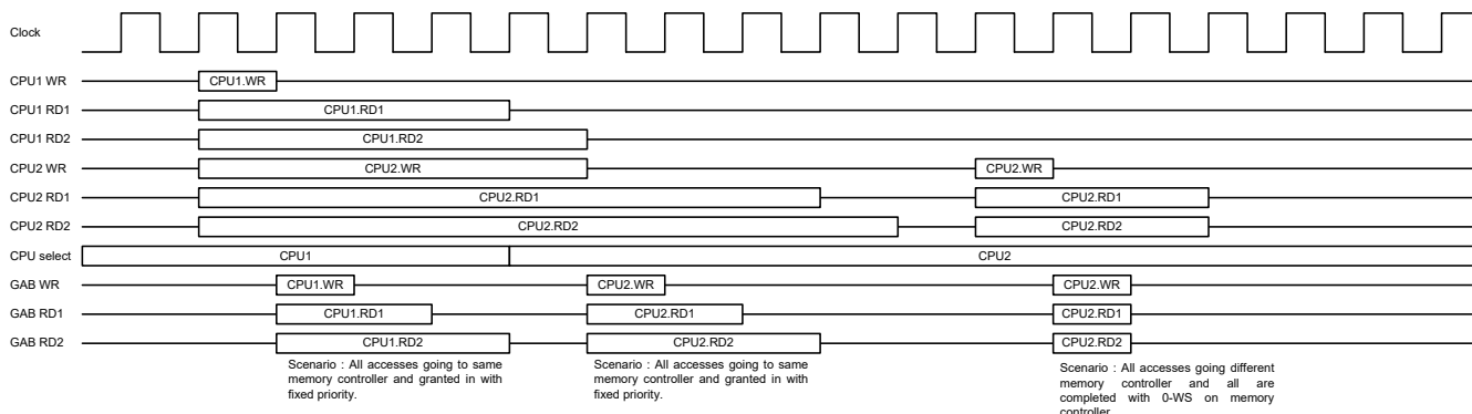
Figure 2-25. Global Access Bridge Arbitration
