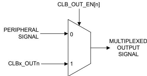
Figure 10-10. CLB Output Signal Multiplexer
