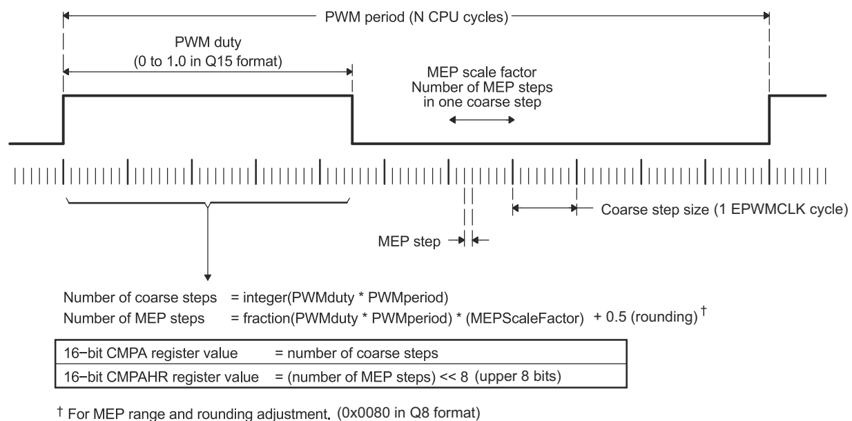
Figure 27-110. Operating Logic Using MEP
