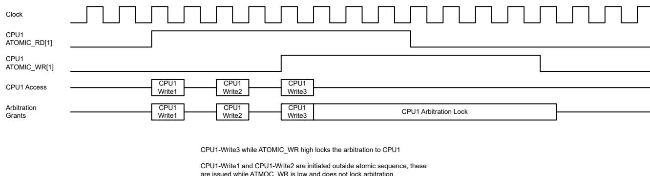
Figure 2-20. Atomic Operations in the MEMSS
