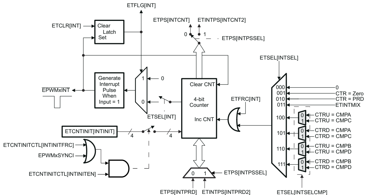
Figure 27-71. Event-Trigger Interrupt Generator
