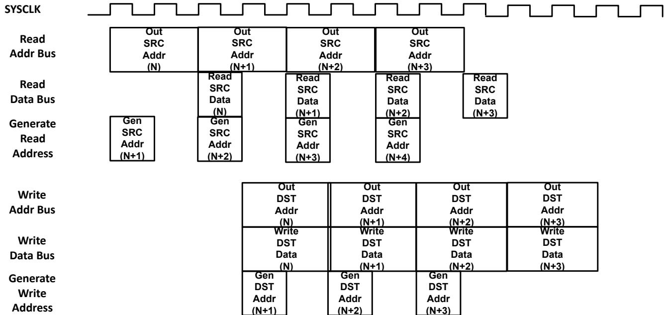
Figure 12-4. 3-stage Pipeline: With One Read Stall
