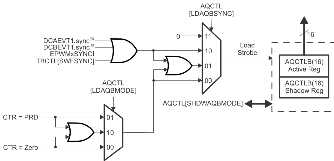
Figure 27-24. AQCTL[SHDWAQAMODE]
