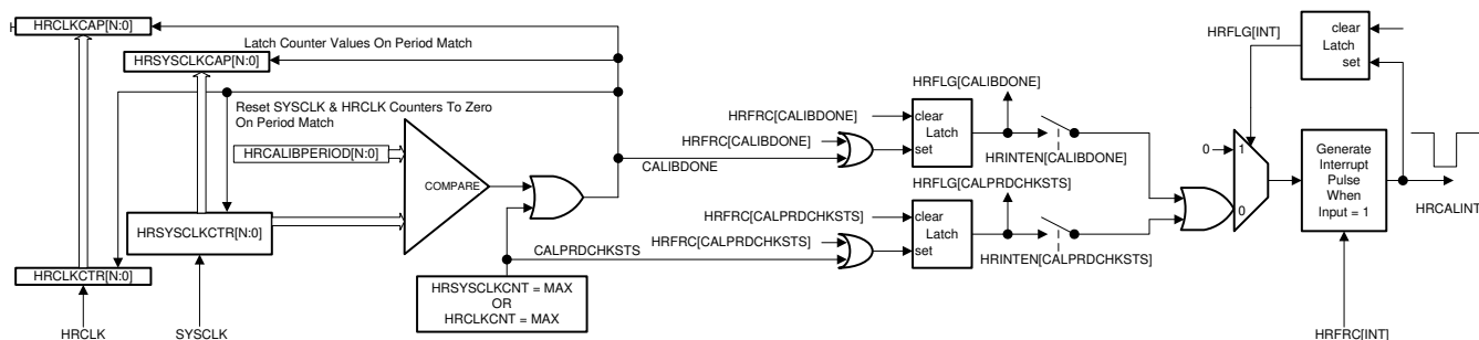
Figure 26-2. HRCAP Calibration
