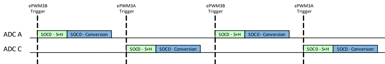
Figure 22-42. Example: Synchronous Equivalent Operation with Non-Overlapping Conversions
