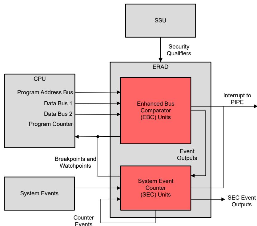
Figure 16-1. ERAD Overview
