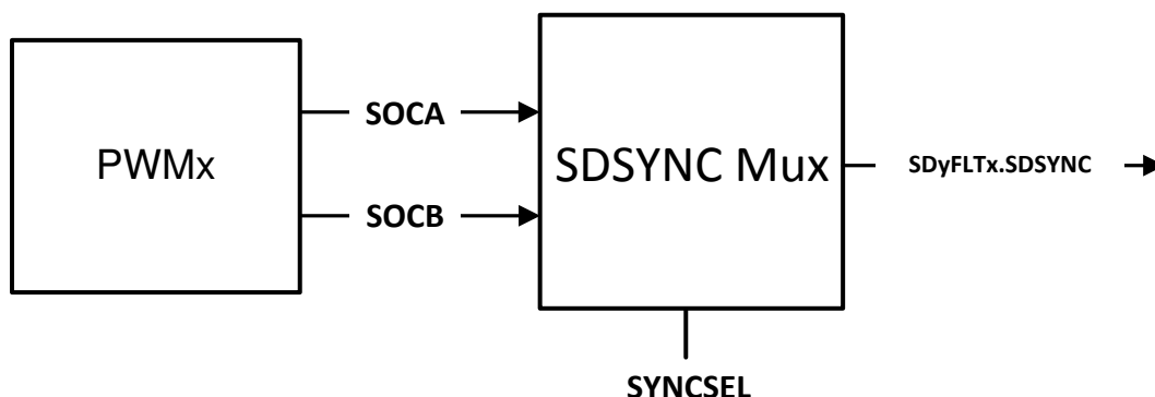
Figure 29-10. SDSYNC Event
