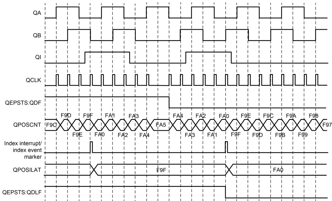
Figure 28-11. Software Index Marker for 1000-line Encoder (QEPCTL[IEL] = 1)
