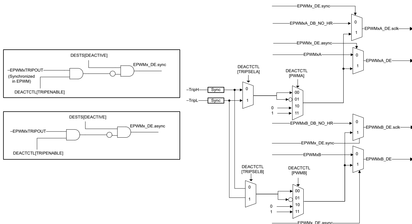
Figure 27-58. Diode Emulation Circuit
