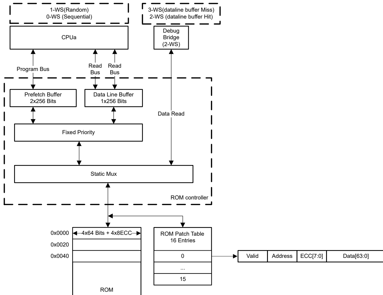
Figure 2-27. ROM Controller
