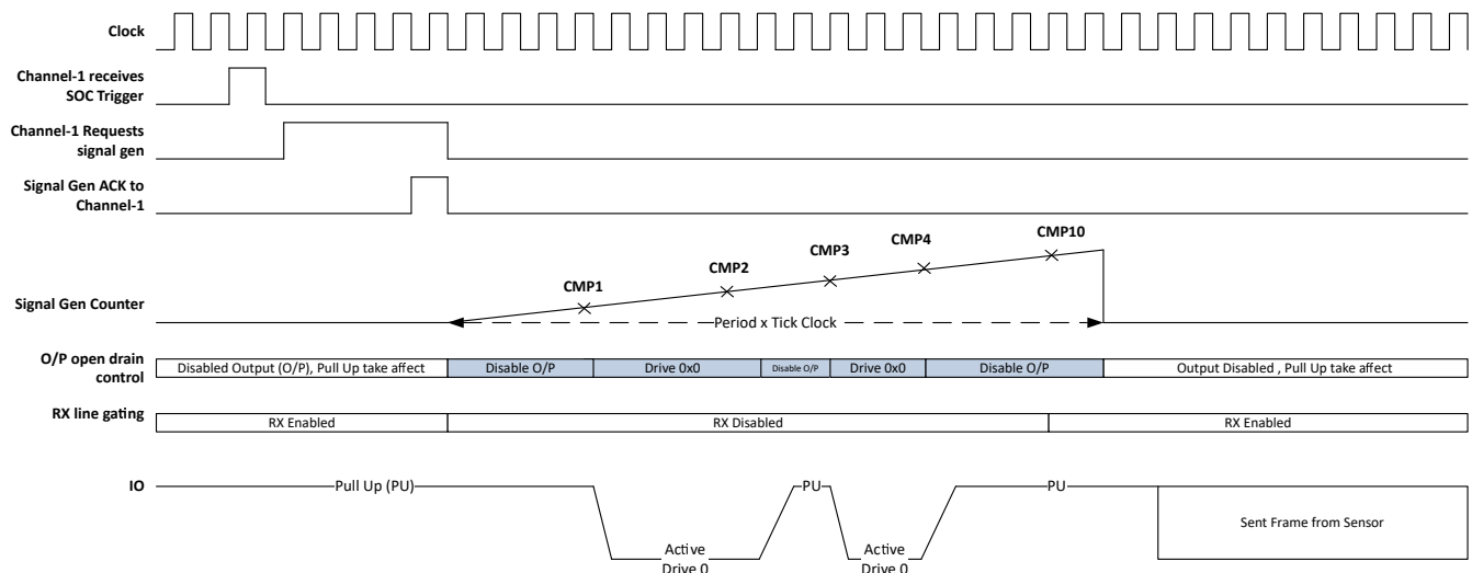
Figure 38-2. SENT Output Control
