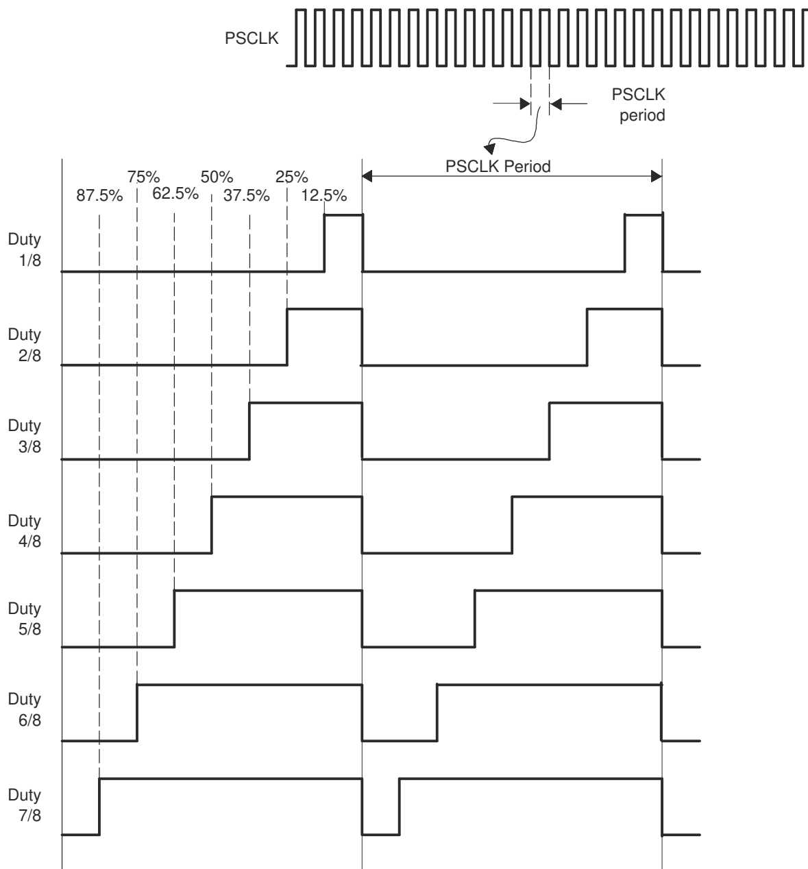
Figure 27-47. PWM Chopper Submodule Waveforms Showing the Pulse Width (Duty Cycle) Control of Sustaining Pulses
