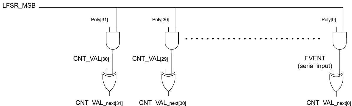
Figure 10-13. LFSR Modes
