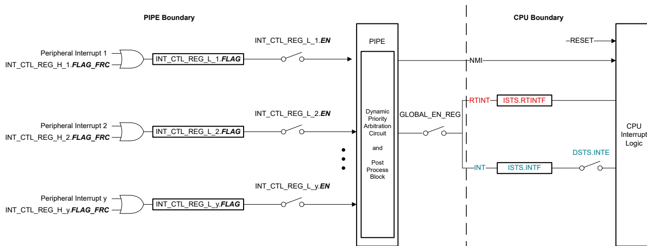
Figure 5-3. Interrupt Propagation
