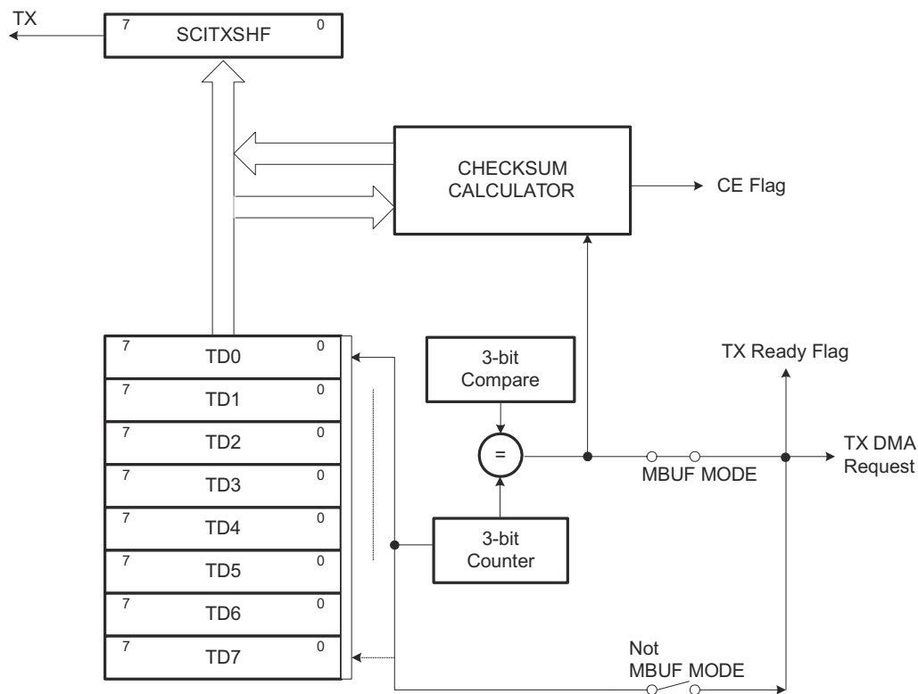
Figure 36-9. Transmit Buffers
