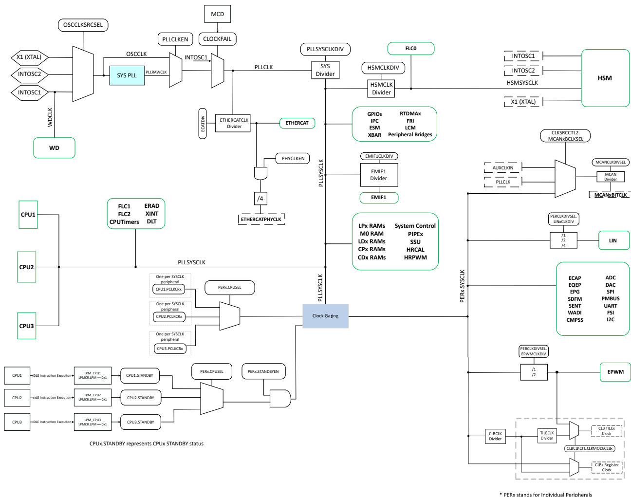
Figure 2-4. Clocking System
