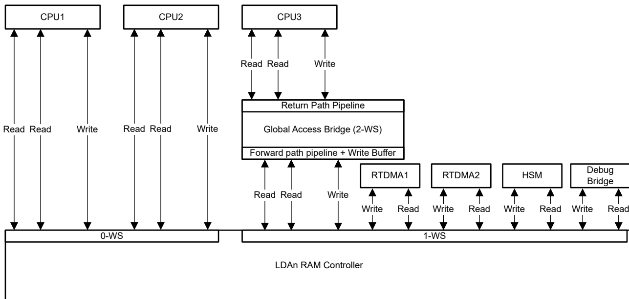
Figure 2-24. Global Access Bridge for LDAn RAMs
