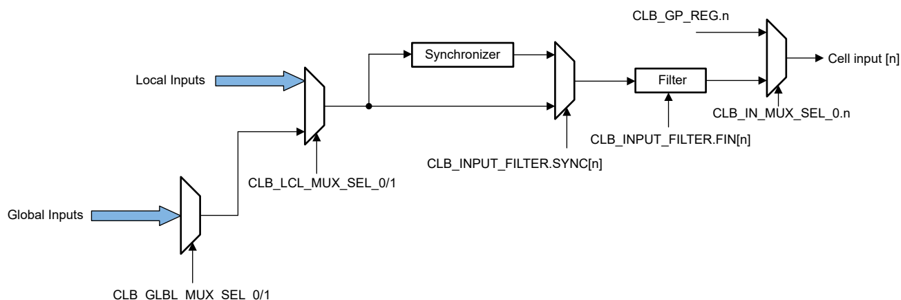
Figure 10-6. CLB Input Mux and Filter
