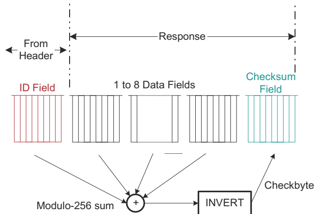
Figure 36-23. LIN 2.0-Compliant Checksum Generation at Transmitting Node
