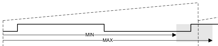
Figure 27-86. Capture Logic Boundary Condition
