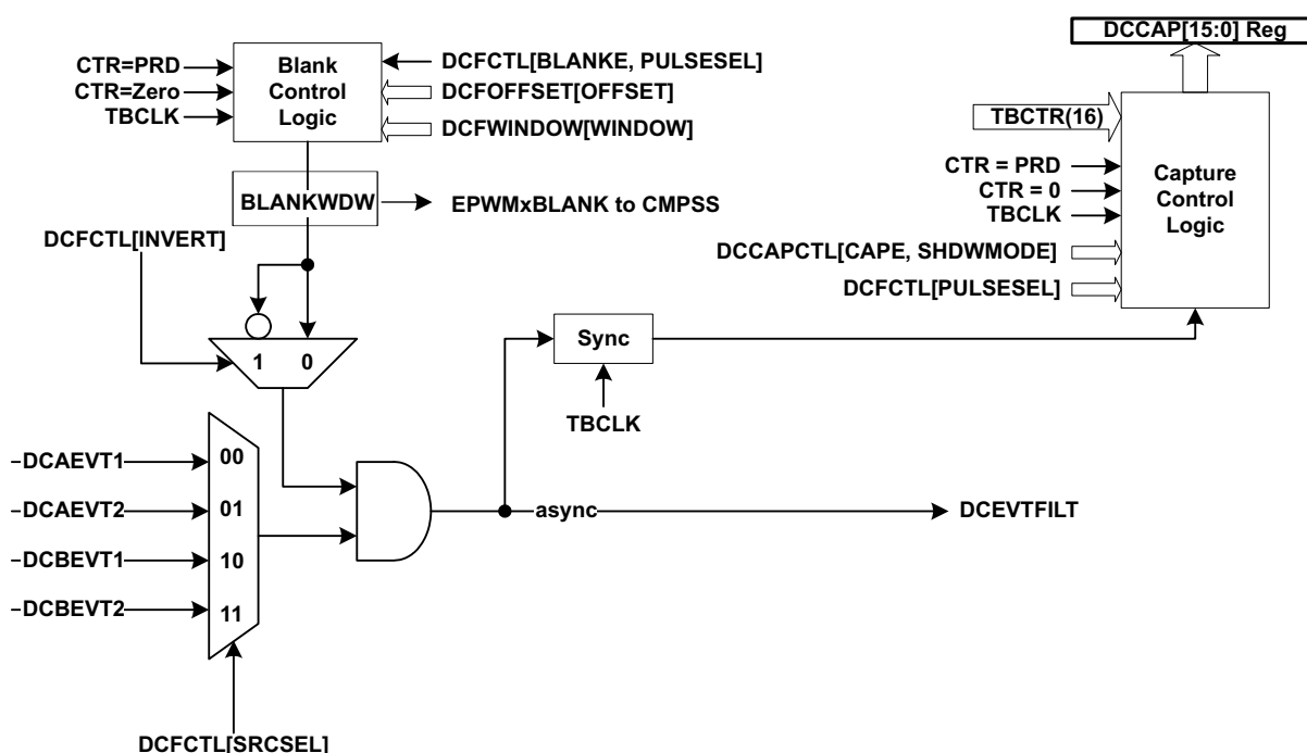
Figure 27-78. Event Filtering
