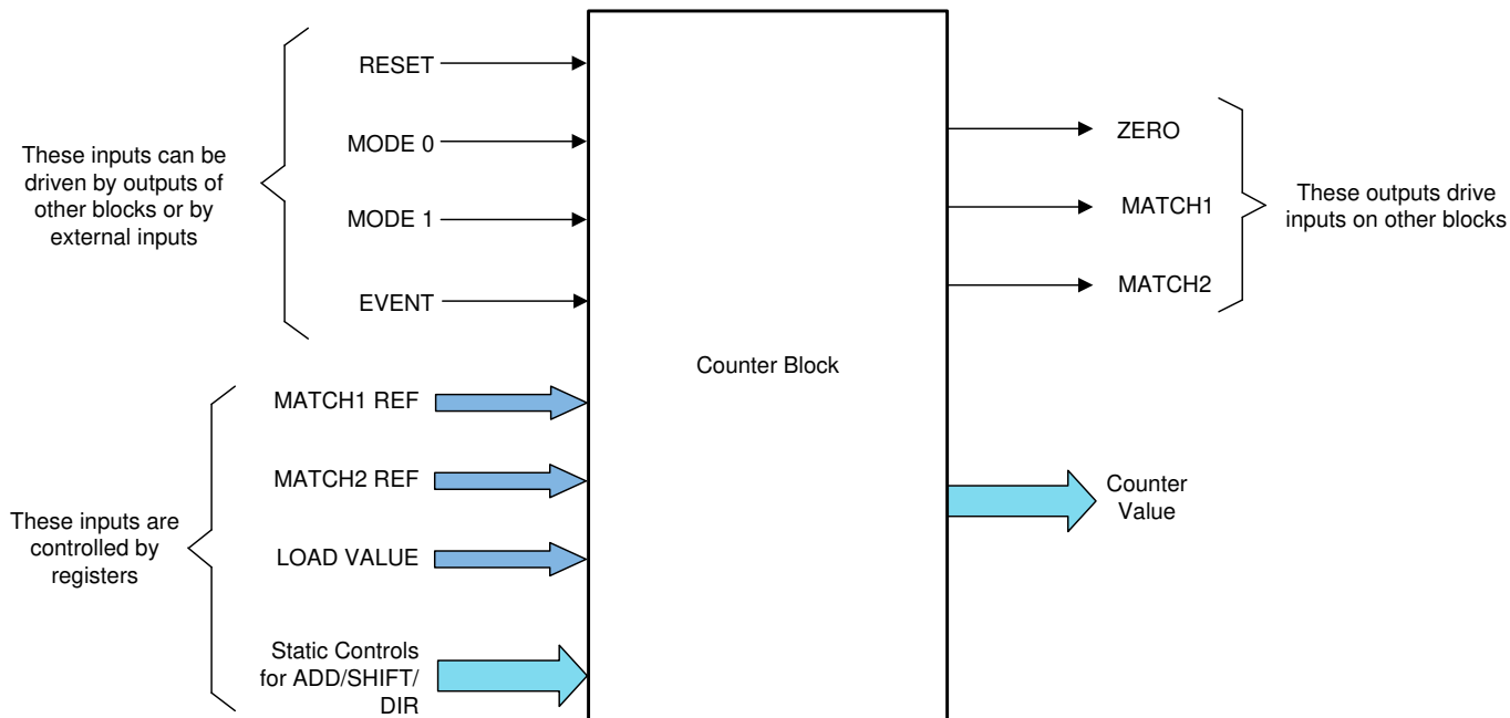
Figure 10-12. Counter Block
