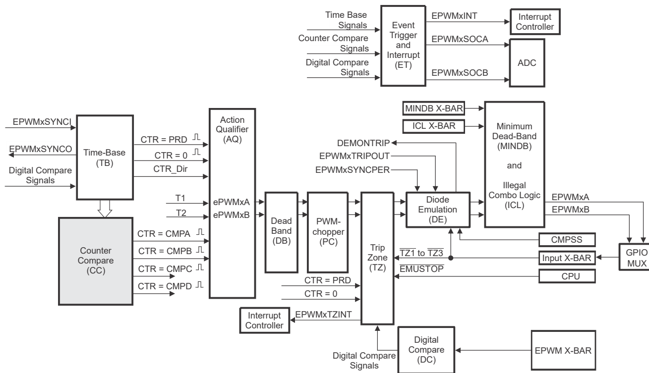
Figure 27-15. Counter-Compare Submodule
