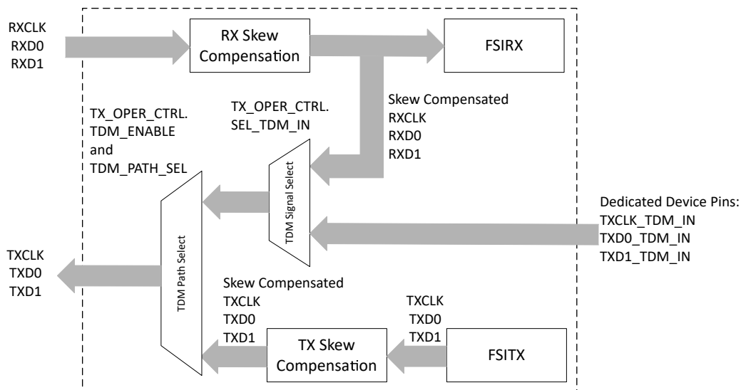
Figure 32-13. TDM Signal Selection
