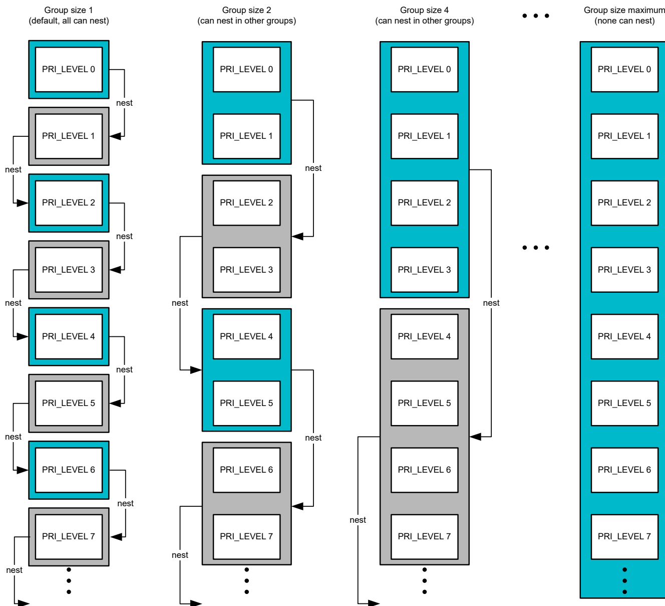
Figure 5-5. Interrupt Grouping
