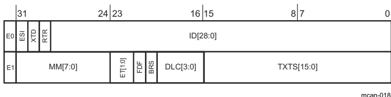
Figure 30-22. Tx Event FIFO Element Structure
