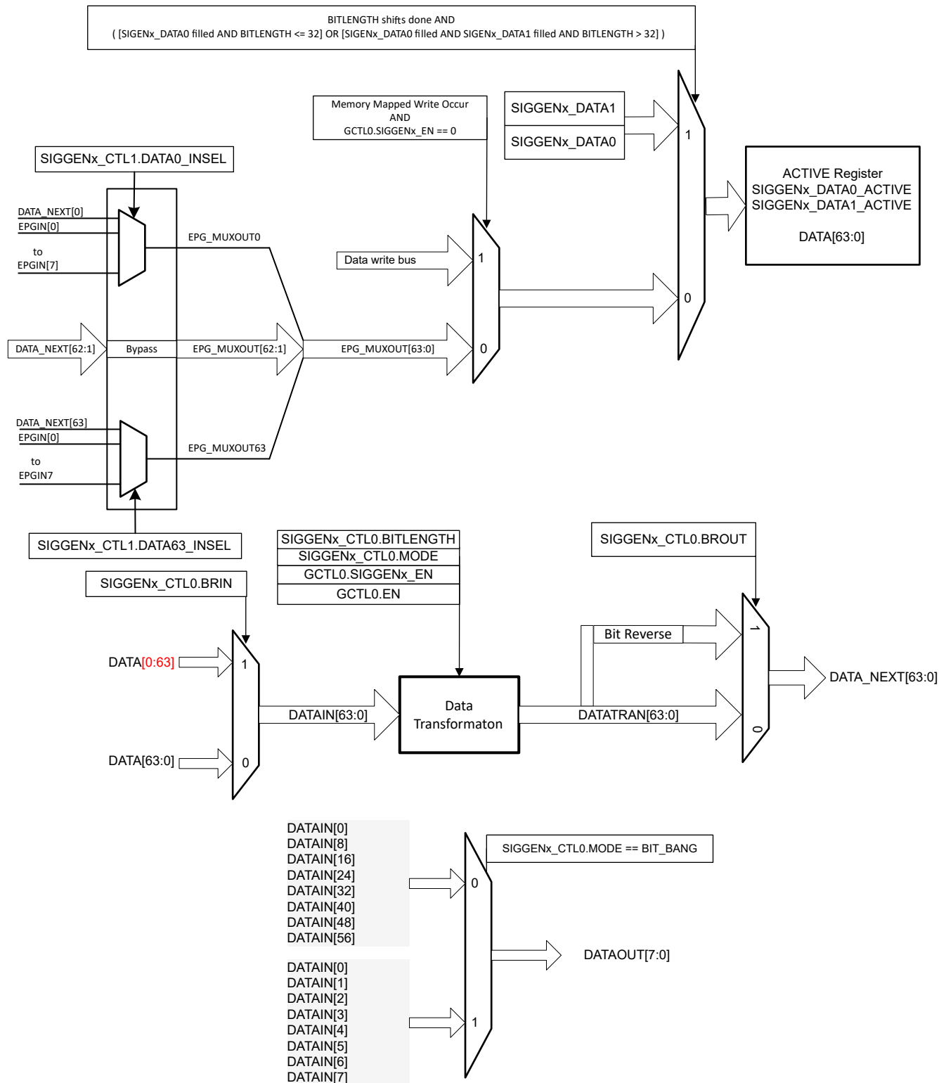
Figure 20-5. EPG Signal Generator Detailed Overview
