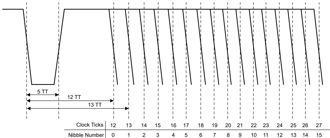
Figure 38-3. Nibble Pulse
