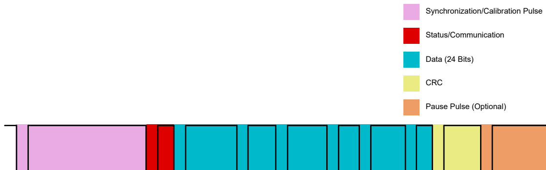
Figure 38-4. Fast Message
