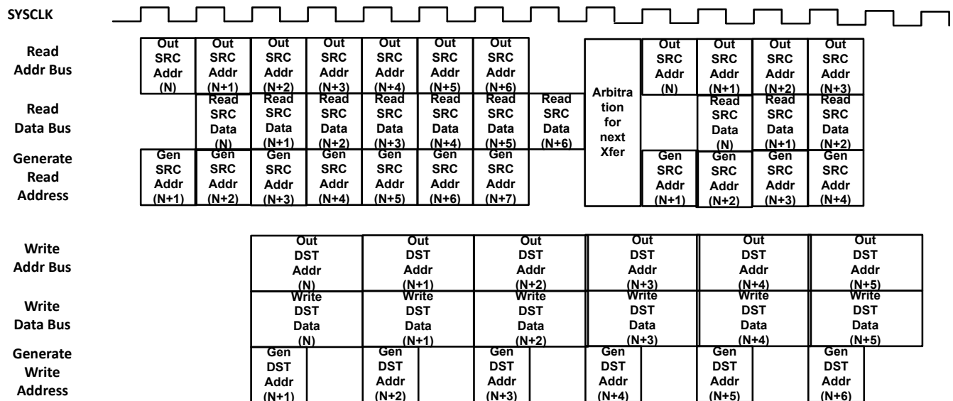
Figure 12-5. 3-stage Pipeline: With One Write Stall
