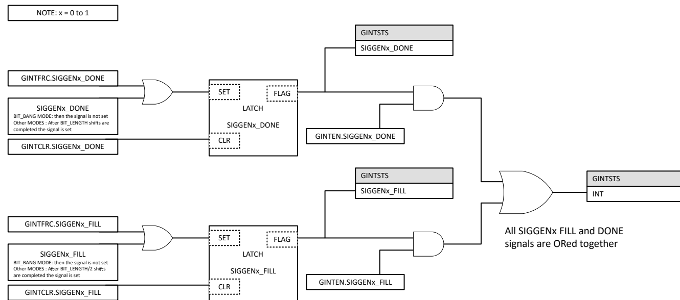
Figure 20-7. EPG Interrupt
