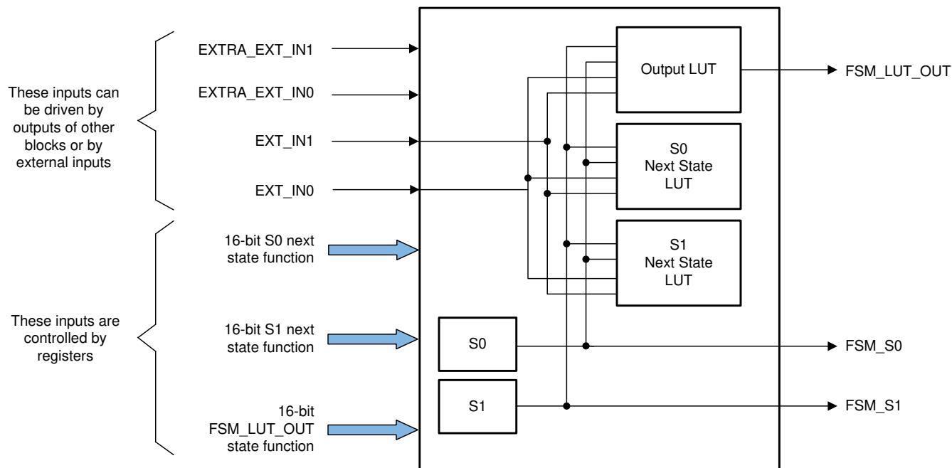
Figure 10-14. FSM Block
