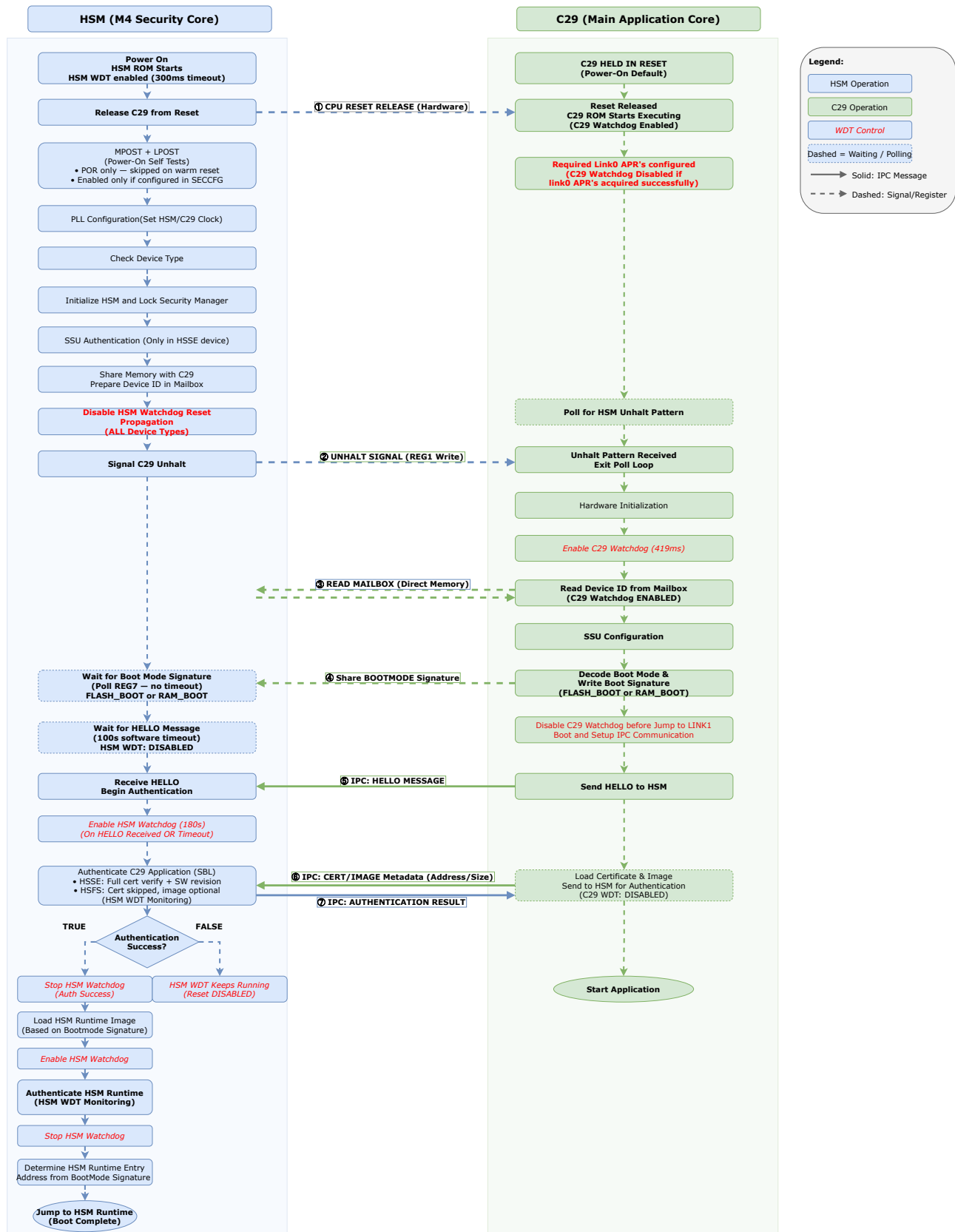
Figure 3-1. F29x device boot flow high level
