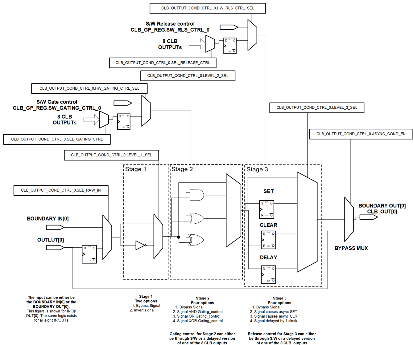
Figure 10-18. AOC Block
