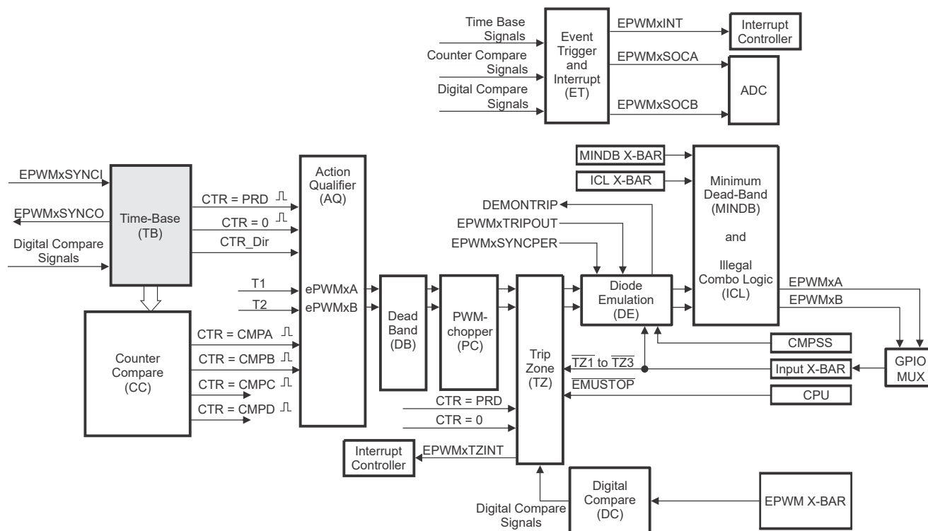
Figure 27-4. Time-Base Submodule
