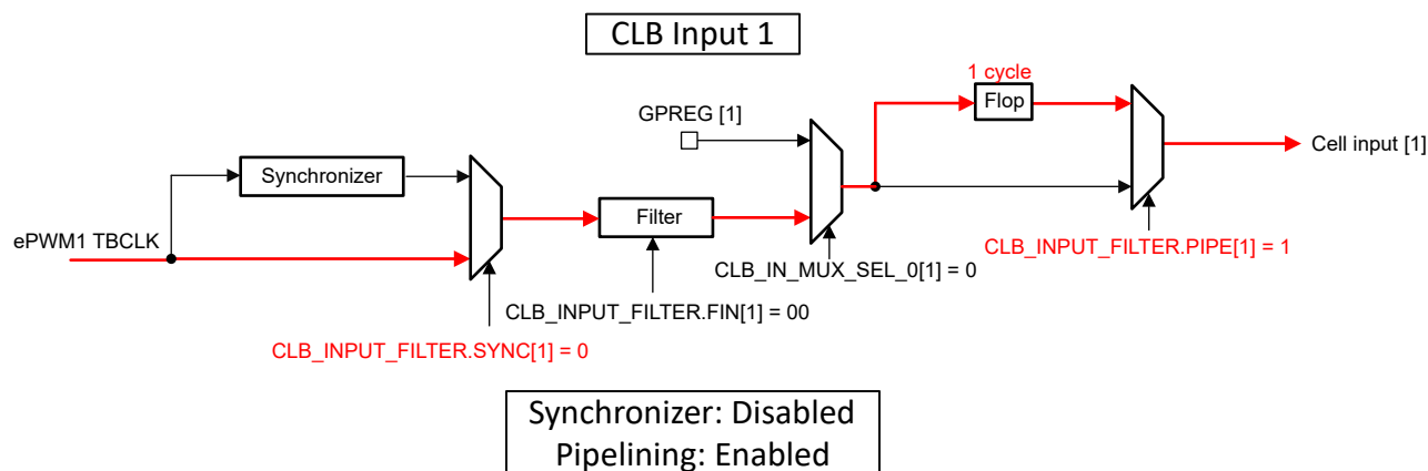
Figure 10-8. CLB Input Pipelining Example
