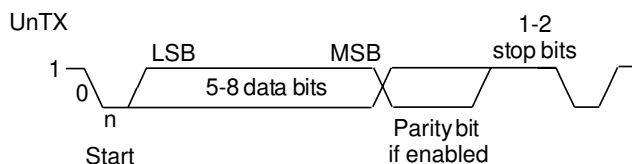
Figure 35-2. UART Character Frame
