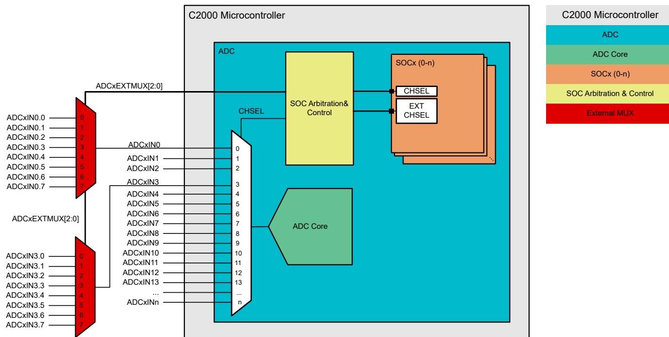
Figure 22-14. ADC with Multiple External Input Muxes and Shared Selection
