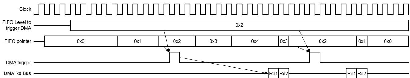
Figure 38-9. RTDMA Trigger Example
