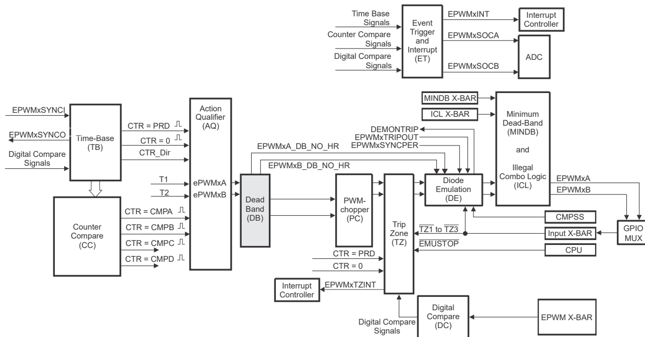
Figure 27-40. Dead_Band Submodule
