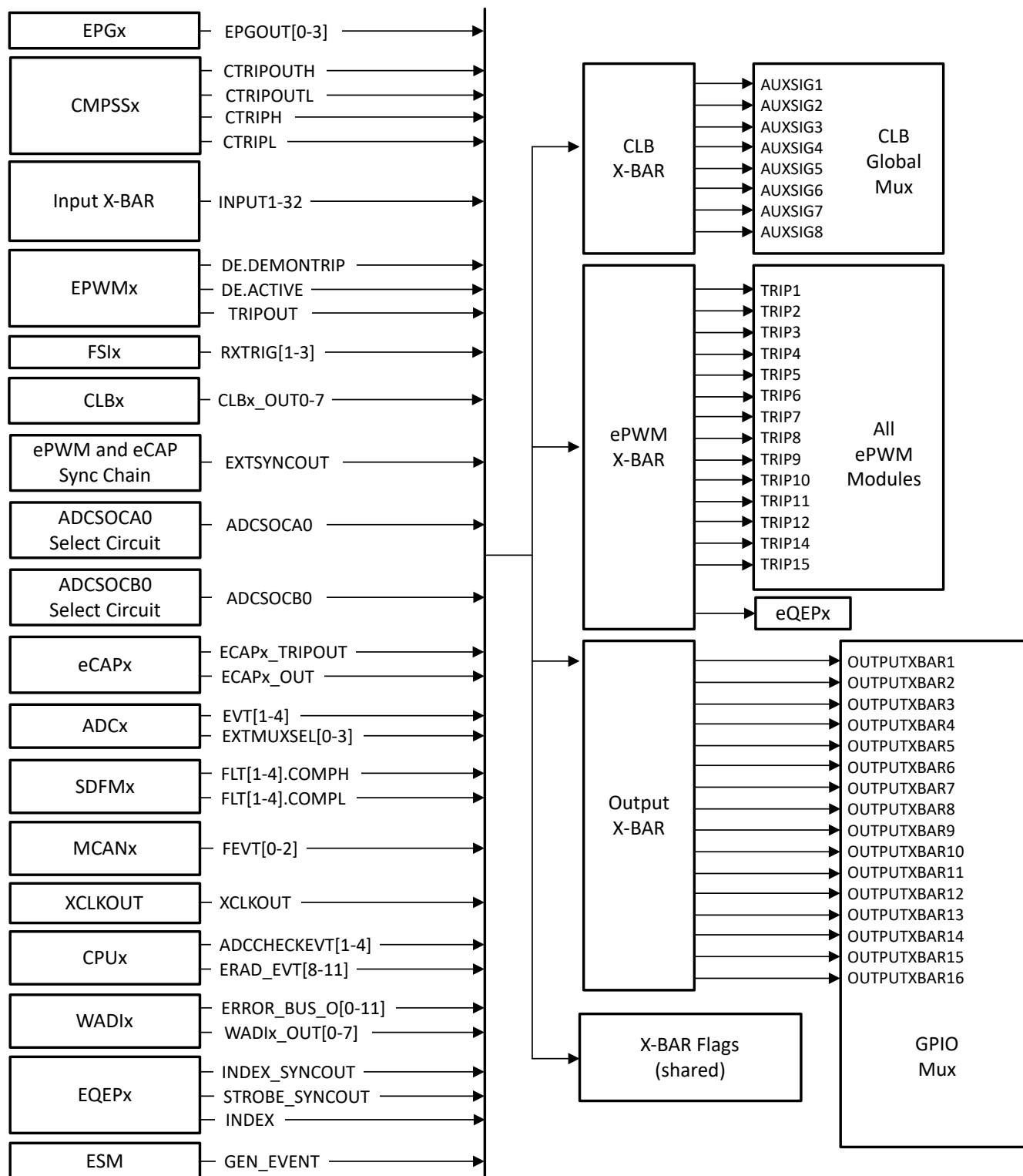
Figure 19-7. X-BAR Input Sources
