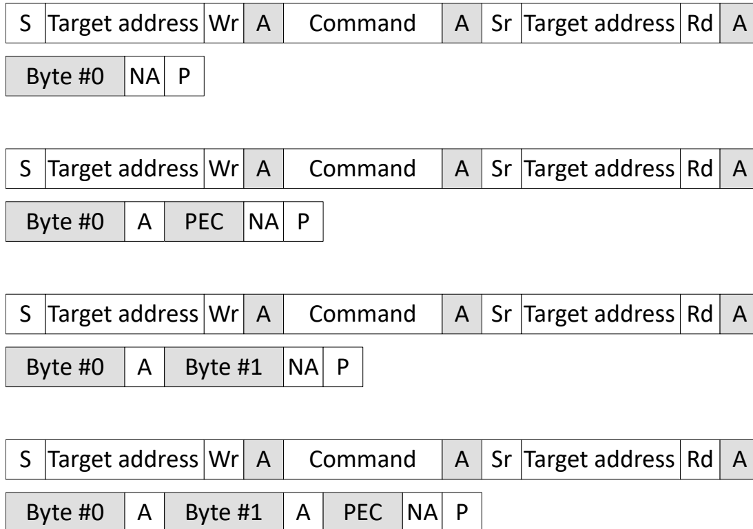
Figure 34-19. Read Byte and Read Word Messages With and Without PEC
