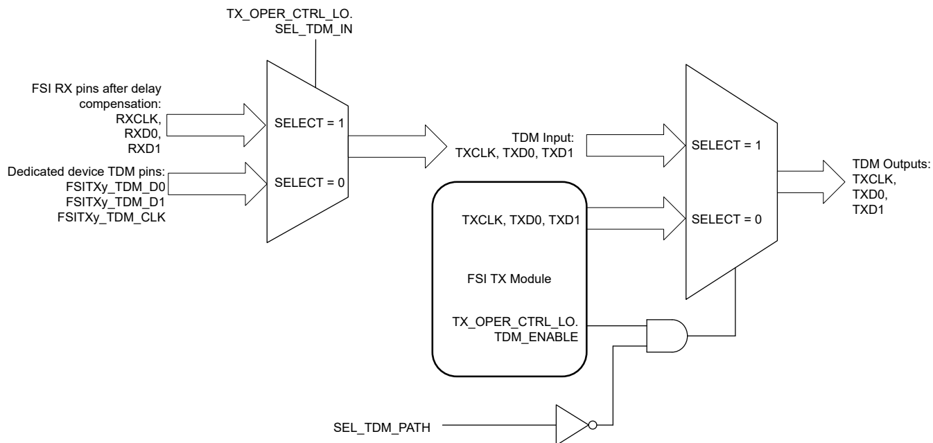
Figure 32-11. FSI Transmitter Multi-Node TDM Multiplexing
