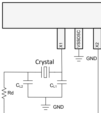
Figure 2-6. External Crystal
