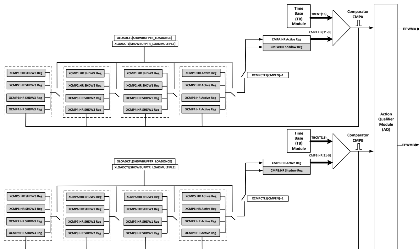
Figure 27-35. XCMP1-4 Allocated to CMPA and XCMP5-8 Allocated to CMPB
