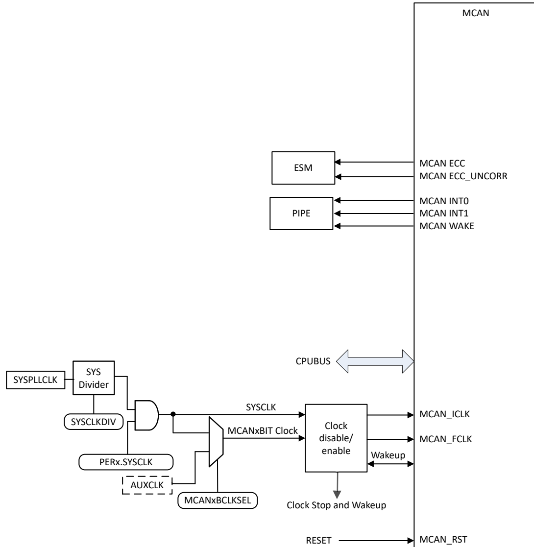
Figure 30-3. MCAN Integration
