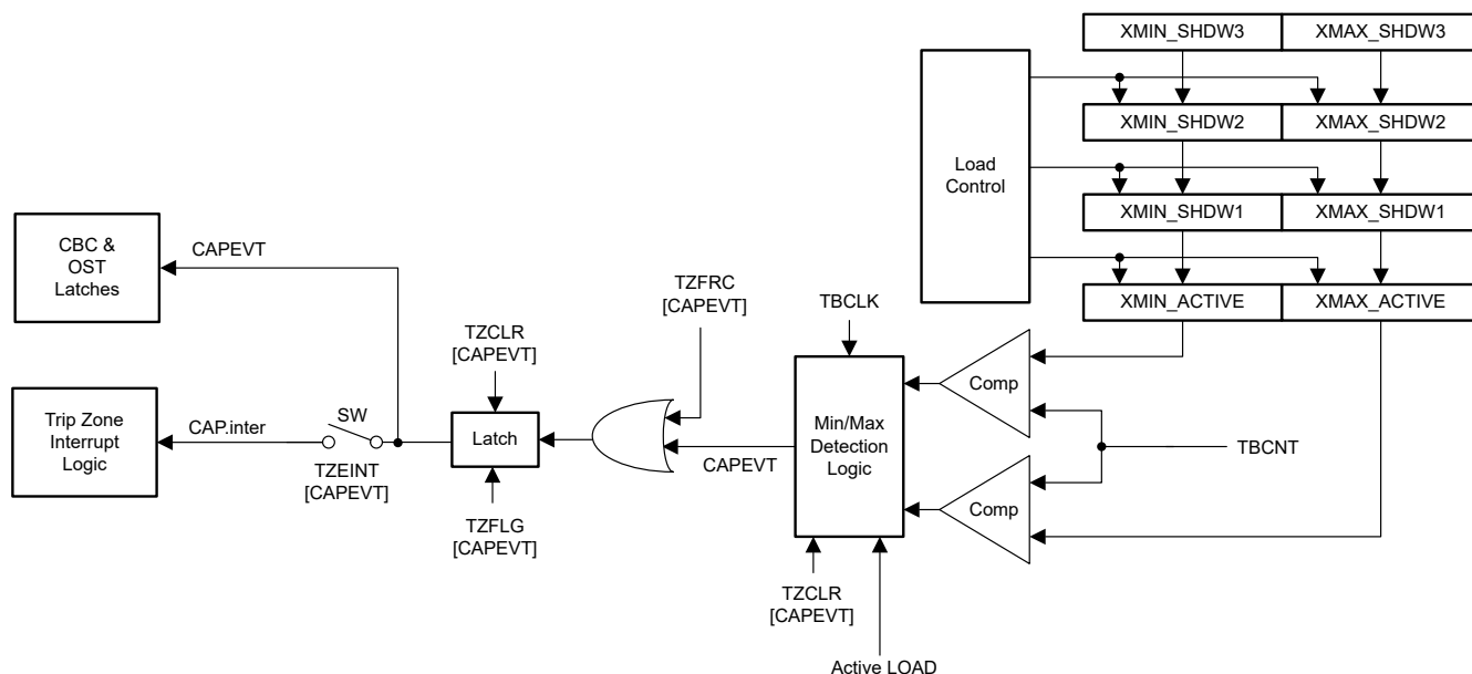
Figure 27-85. MIN and MAX Threshold Detection Logic
