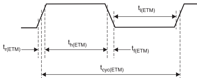
Figure 6-30. ETMTRACECLKOUT Timing
