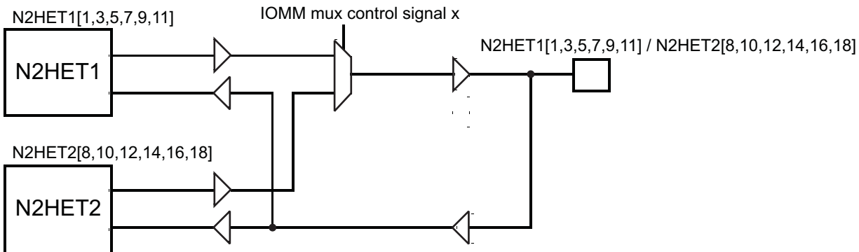
Figure 7-12. N2HET Monitoring
