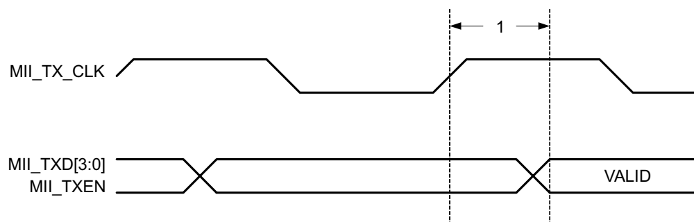
Figure 7-23. MII Transmit Timing
