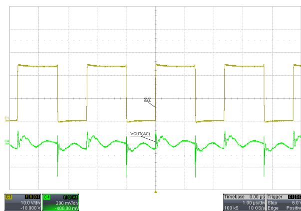
Figure 4-11. V_{IN} = 14\text{-V} , V_{OUT} = 24\text{-V} , P_{OUT} = 200\text{-W}
