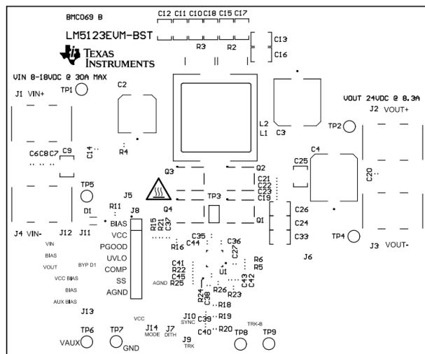
Figure 5-1. Layout: Top Silk Screen
