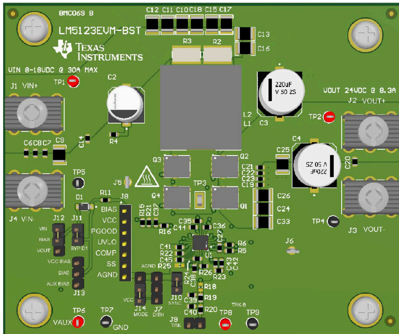
Figure 2-1. EVM Photo
