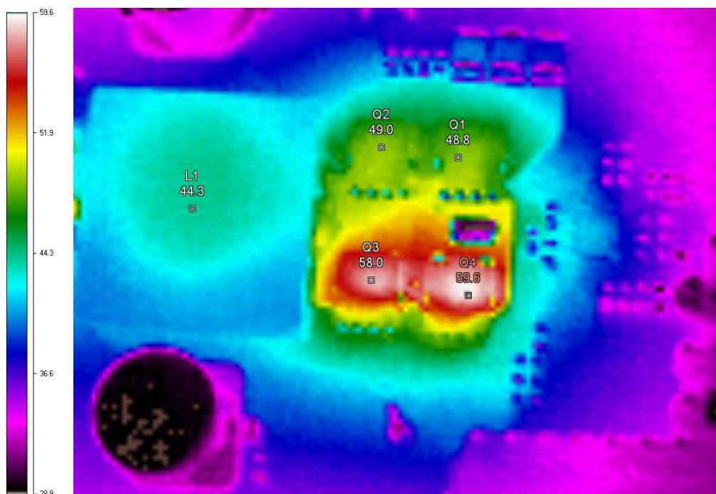
Figure 4-4. Thermal Performance: V_{IN} = 8V , V_{OUT} = 24V , P_{OUT} = 200W , No Forced Airflow
