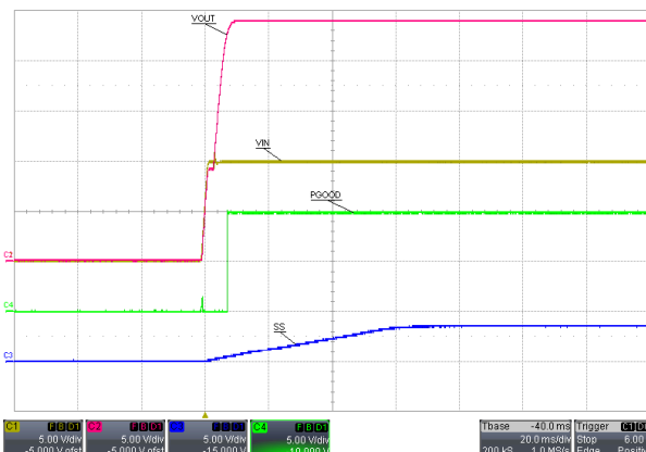
Figure 4-6. V_{IN} = 10\text{-V} , V_{OUT} = 24\text{-V} , P_{OUT} = 200\text{-W}
