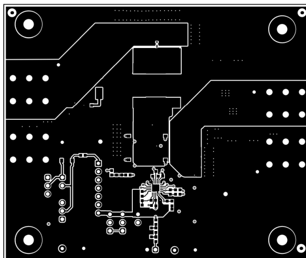
Figure 5-2. Layout: Top Layer
