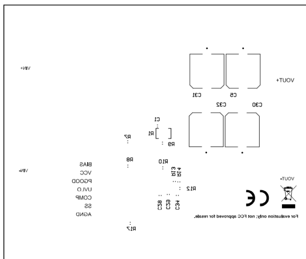
Figure 5-6. Layout: Bottom Silk Screen
