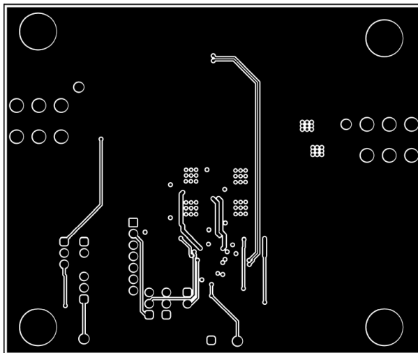
Figure 5-4. Layout: Signal Layer 2
