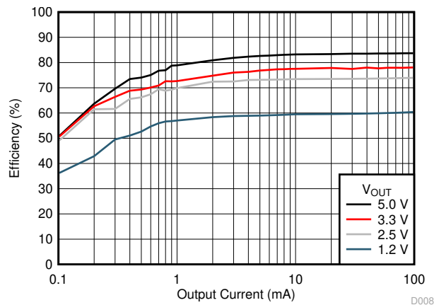
Figure 6-7. Efficiency Log Scale
