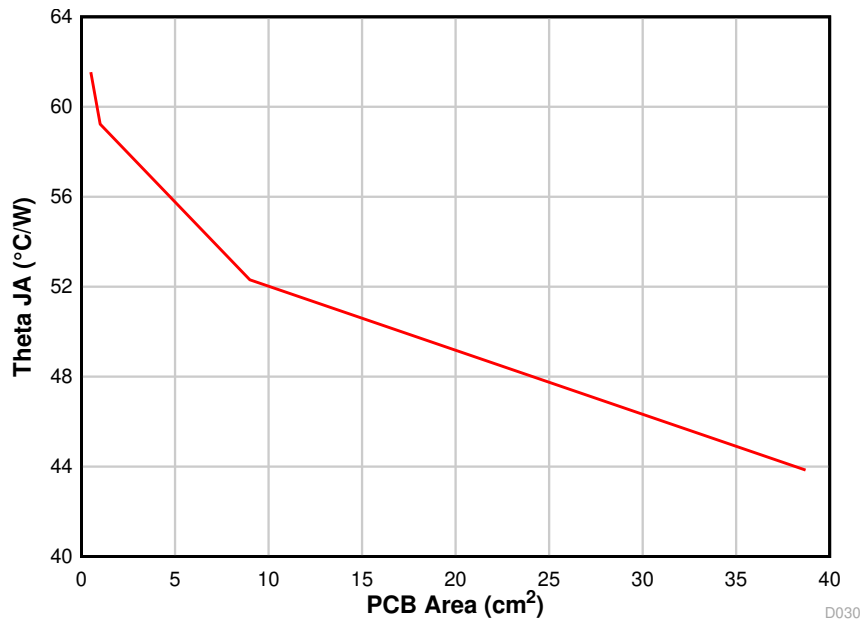
Figure 10-3. \theta_{JA} versus PCB Area
