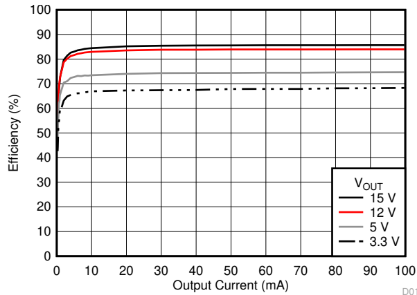
Figure 6-16. Efficiency
