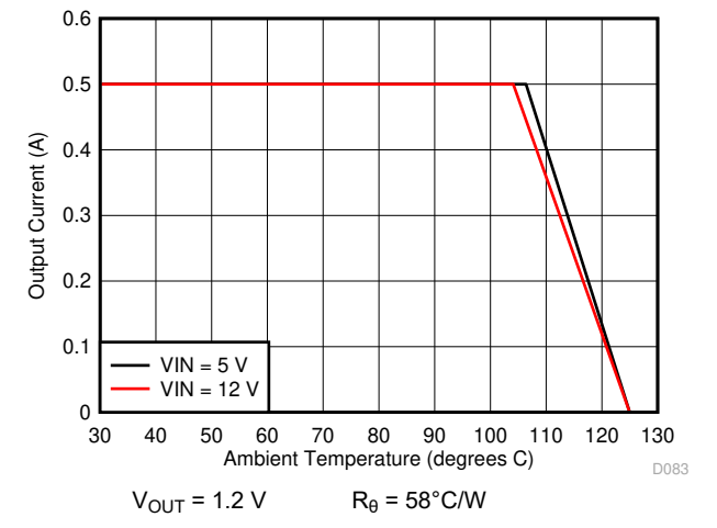
Figure 7-16. Ambient Temperature vs Output Current
