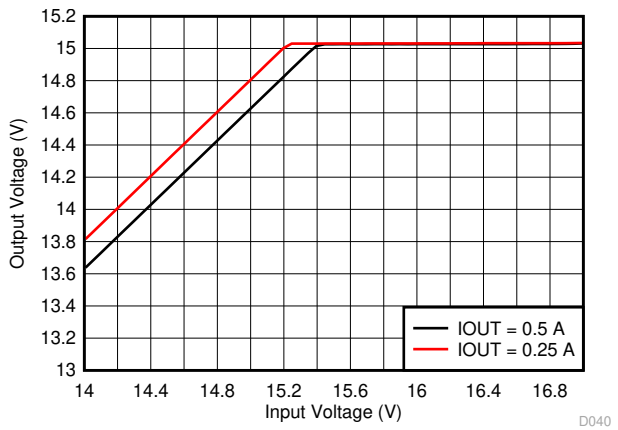
Figure 7-4. Dropout Voltage
