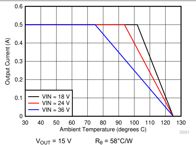
Figure 7-22. Ambient Temperature vs Output Current
