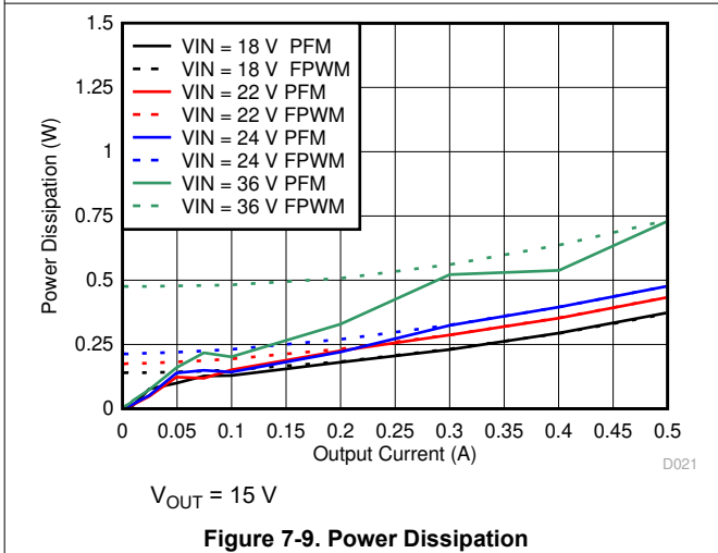
Figure 7-9. Power Dissipation
