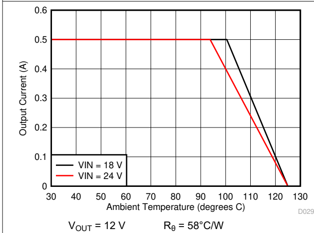
Figure 7-21. Ambient Temperature vs Output Current
