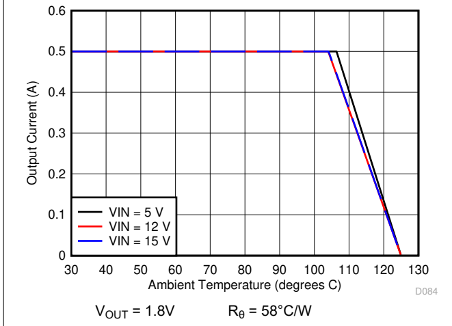
Figure 7-17. Ambient Temperature vs Output Current
