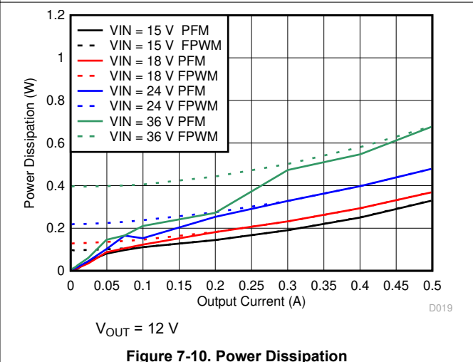
Figure 7-10. Power Dissipation
