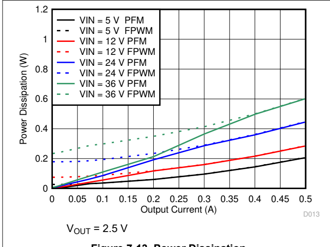
Figure 7-13. Power Dissipation
