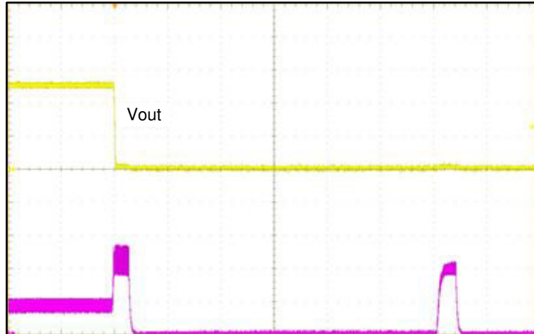
Figure 8-2. Hiccup Operation
