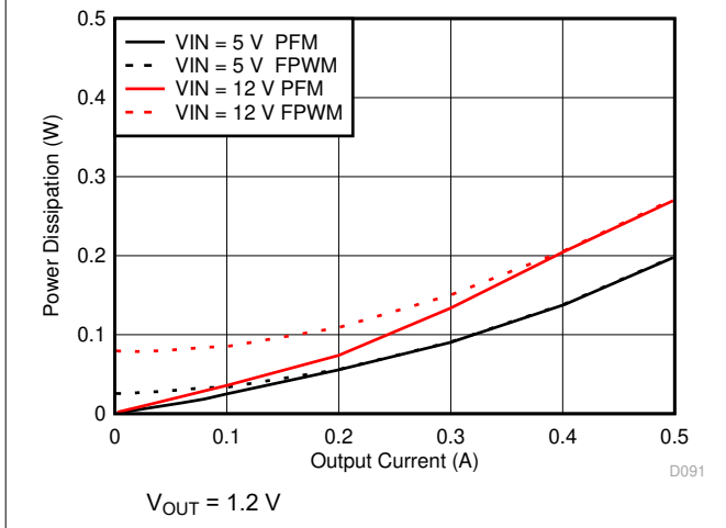
Figure 7-15. Power Dissipation
