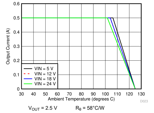
Figure 7-18. Ambient Temperature vs Output Current
