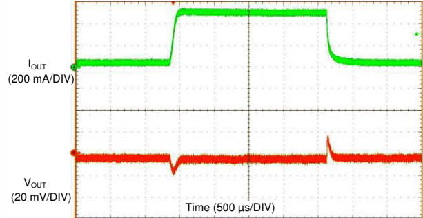
5-V Adjustable Output MODE = High 10% to 100% Load Step
