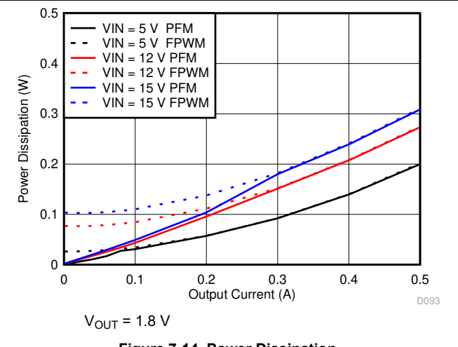
Figure 7-14. Power Dissipation
