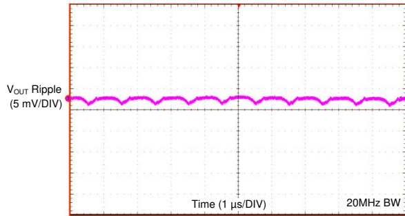
5-V Adjustable Output I_{OUT} = 0.5\text{ A}
