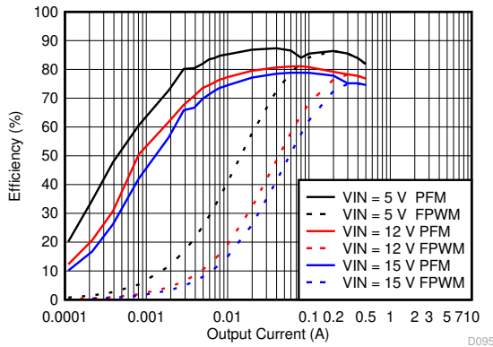
Figure 9-36. Efficiency for V_{OUT} = 1.8\text{ V}
