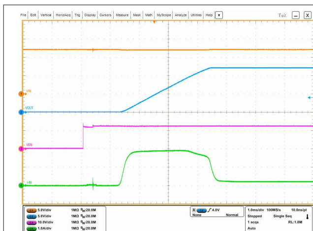
Figure 5-4. Turn ON Using EN - Inrush Current
