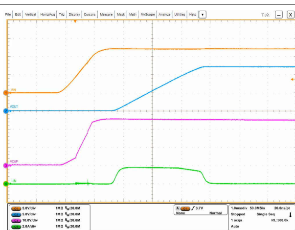
Figure 5-3. Power Up: Charge Pump and Inrush Current
