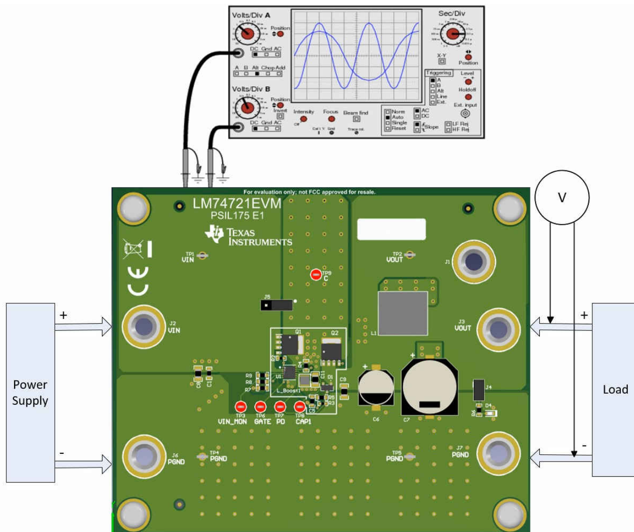
Figure 5-1. LM74721EVM Test Setup
