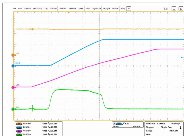
Figure 5-8. Inrush Current With No Load
