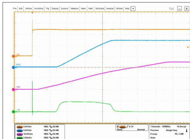
Figure 5-6. Hot-Plug 12 V
