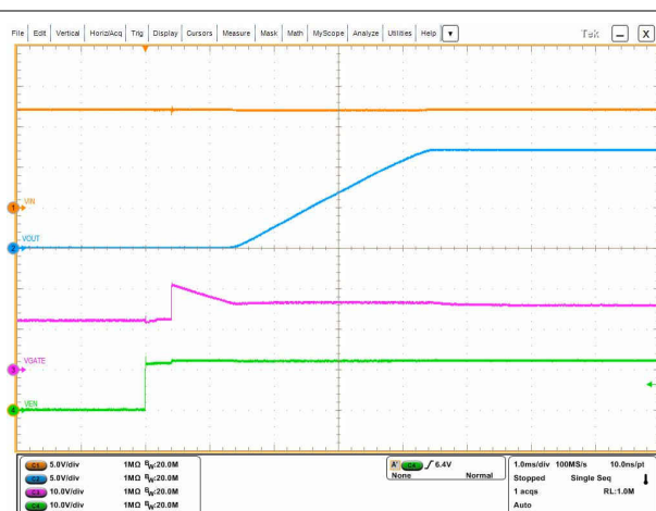
Figure 5-5. Turn ON Using EN - DGATE
