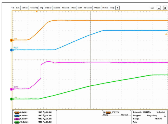
Figure 5-2. Power Up: GATE and PD
