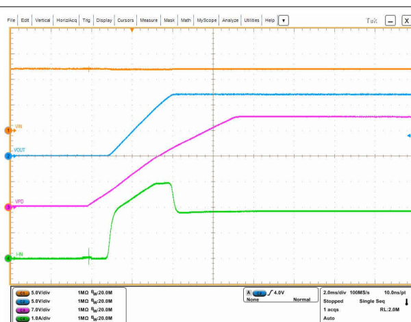
Figure 5-9. Inrush Current With 6-Ω Load
