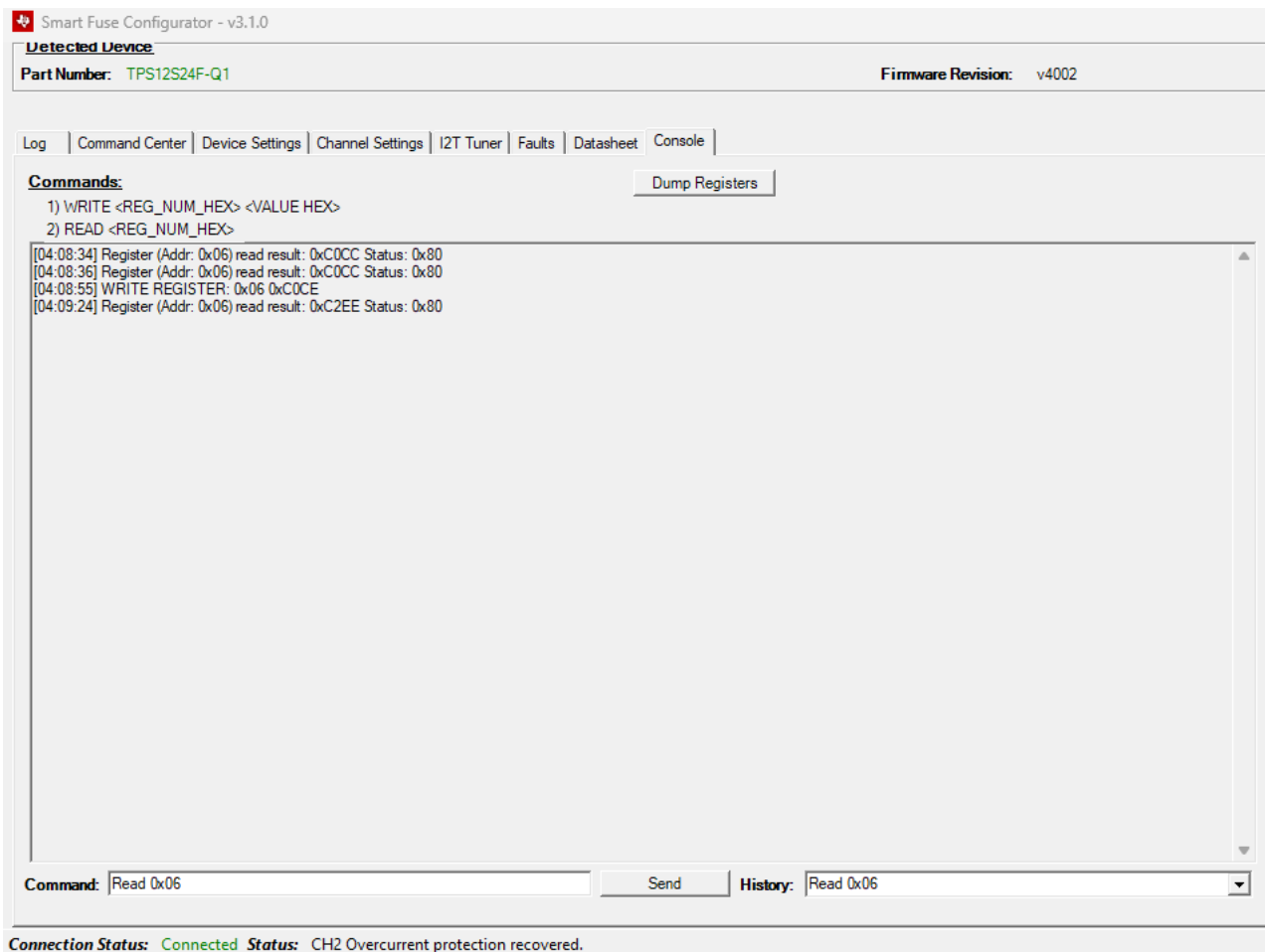
Figure 4-10. Console View
