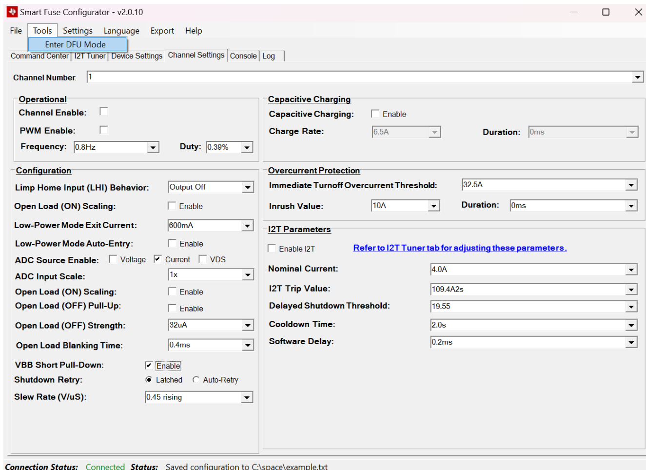
Figure 4-11. Enter Firmware Update Mode
