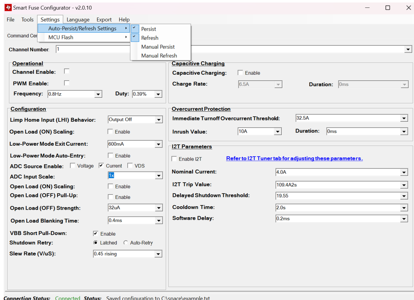
Figure 4-13. Persist Settings
