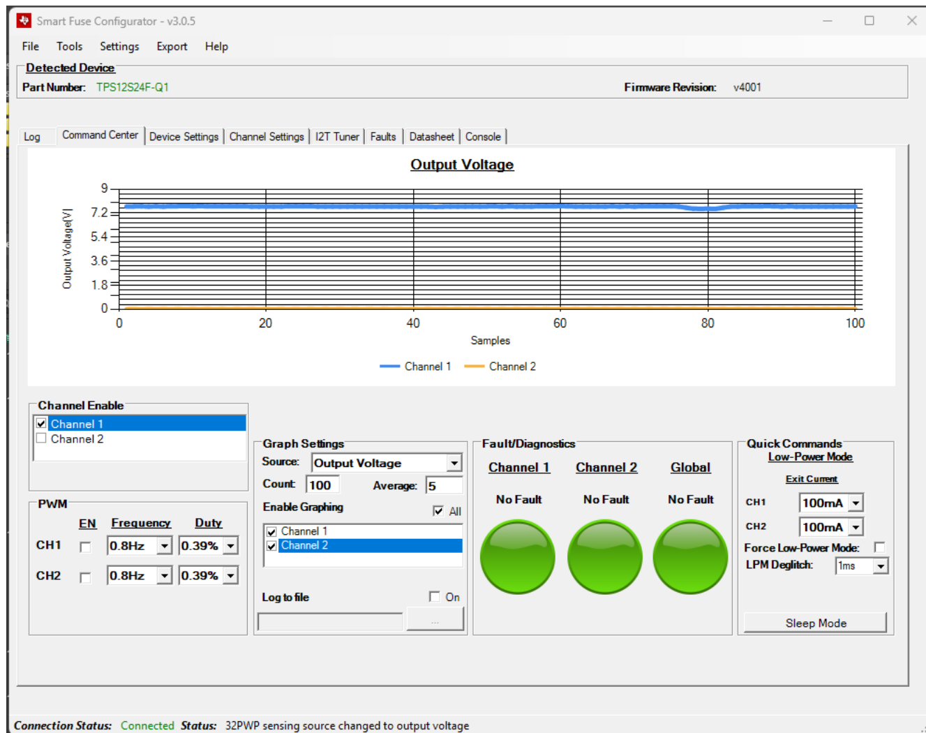
Figure 4-1. Output Voltage Graph
