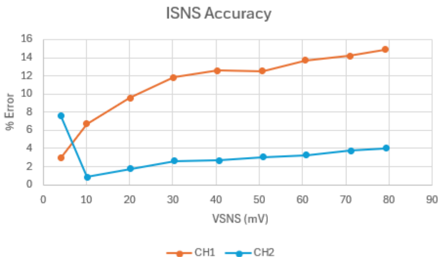
Figure 3-1. EVM ISNS Accuracy
