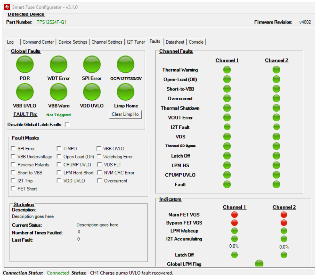
Figure 4-9. Faults Tab
