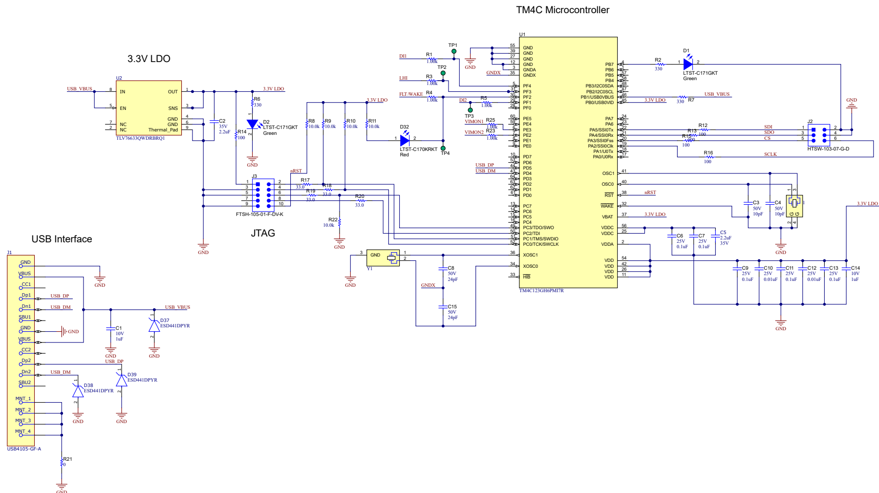
Figure 5-2. MCU Schematic
