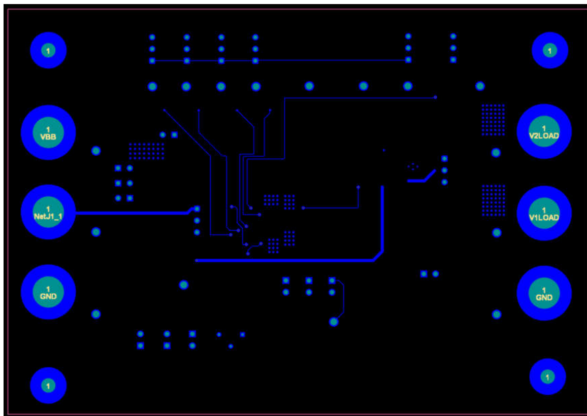
Figure 3-5. Bottom Layer
