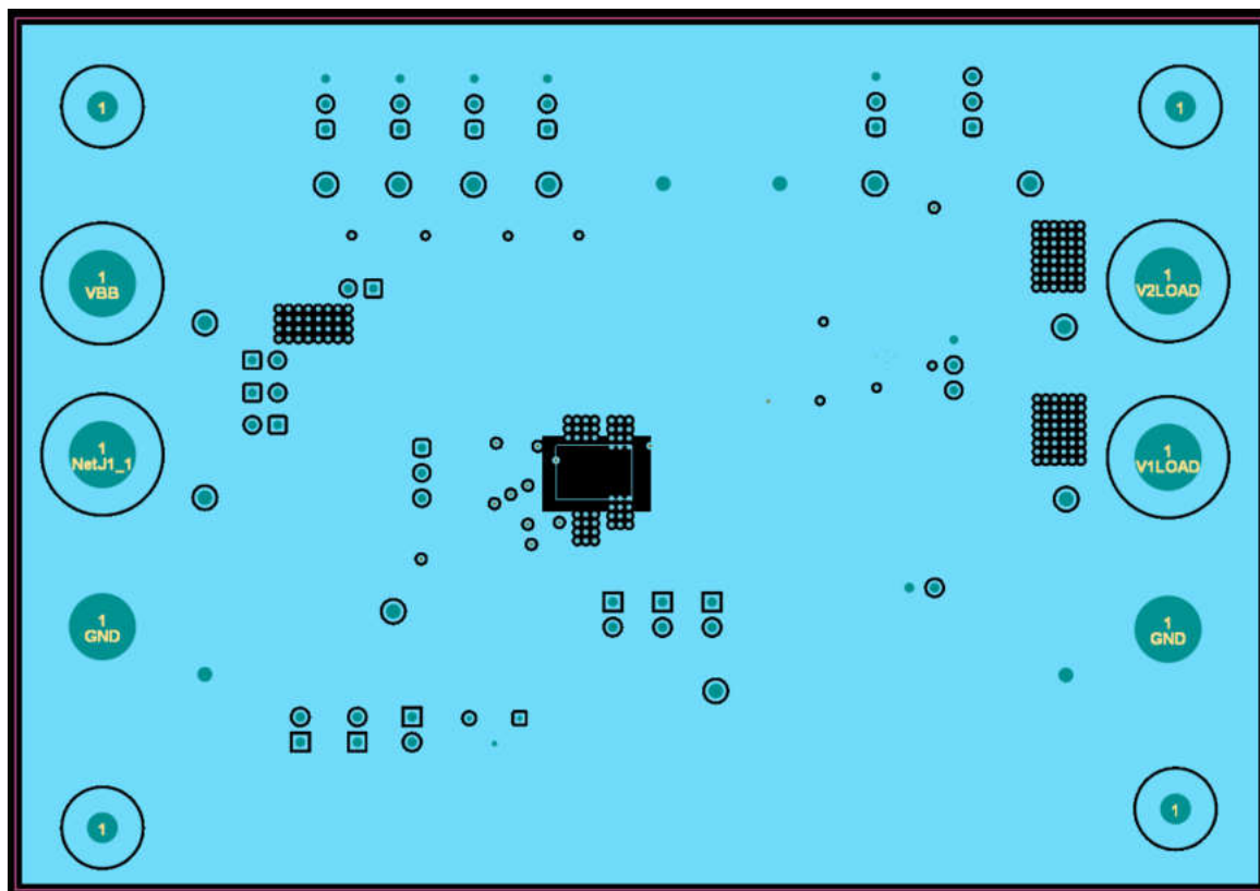
Figure 3-4. Ground Layer
