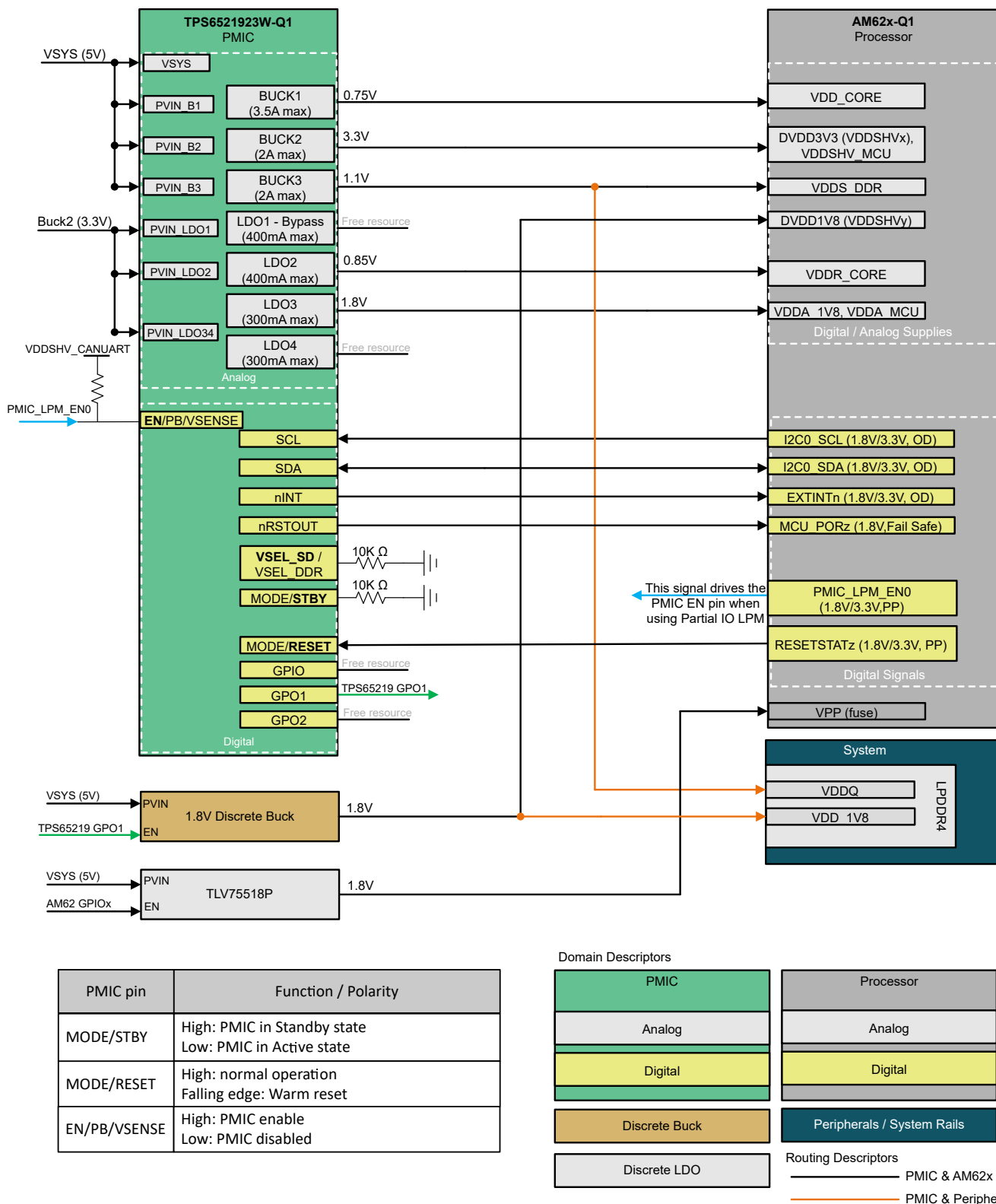
Figure 2-1. TPS6521923W-Q1 Example Power Block Diagram
