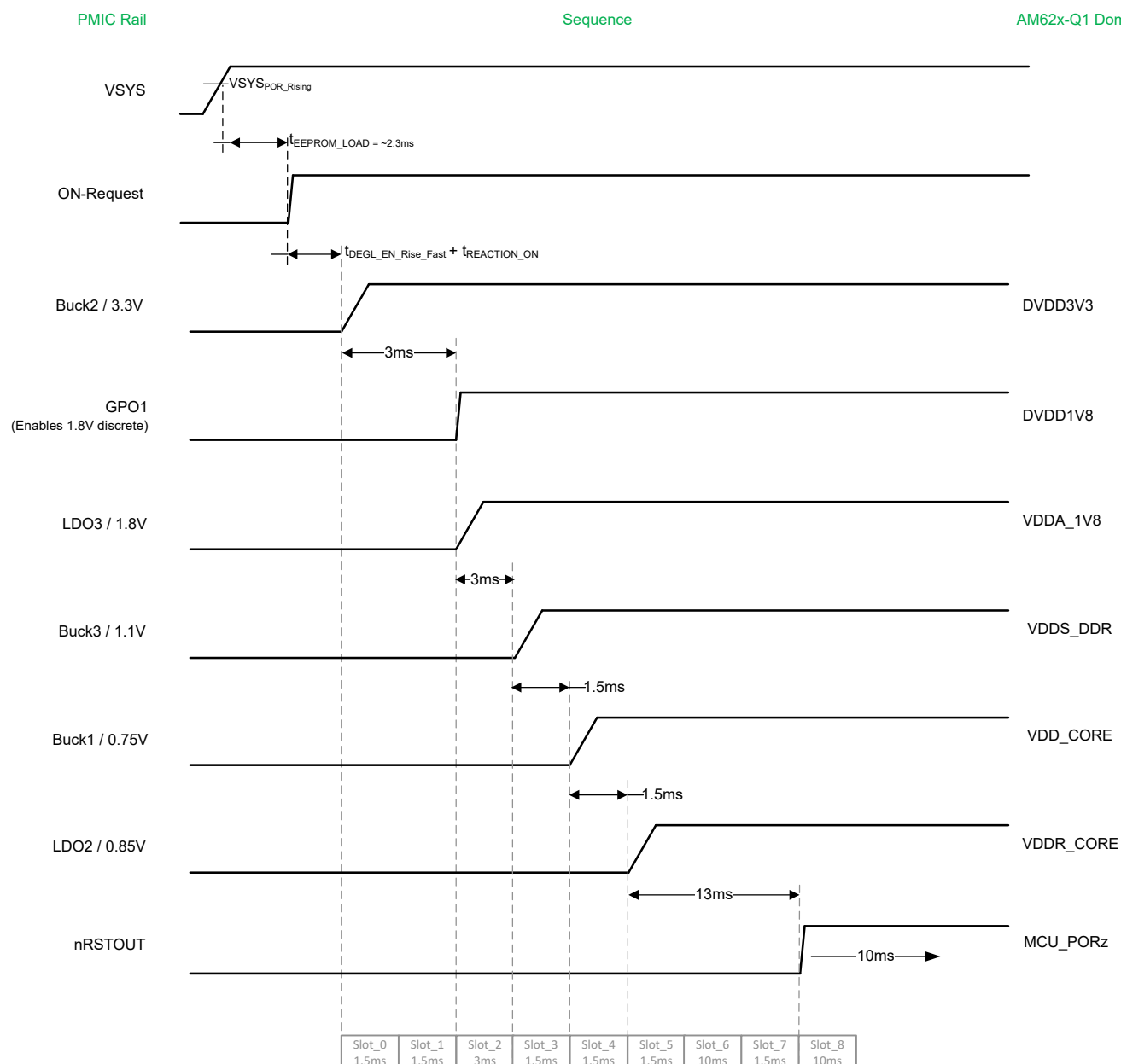
Figure 2-2. TPS6521923W-Q1 Power-Up Sequence
