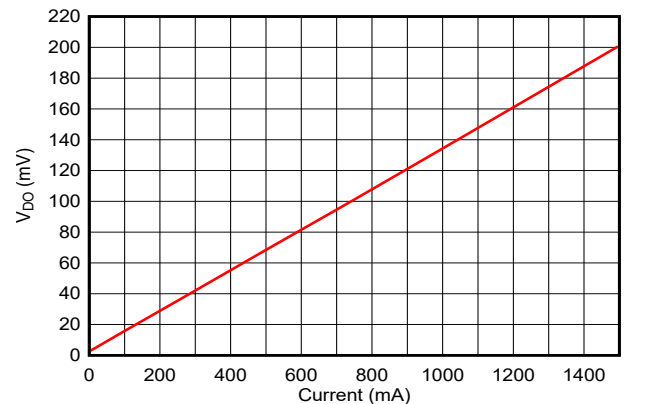
V_{IN} = 5\text{ V} V_{BIAS} = V_{IN} + 1.6\text{ V} Figure 6-29. Dropout Voltage vs Current
