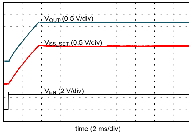
time (2 ms/div) Figure 6-66. Startup Waveform
