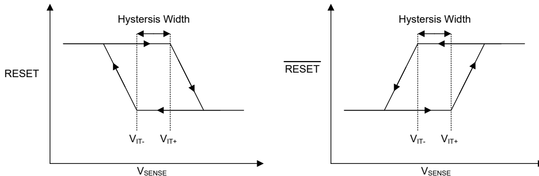
Figure 7-3. Hysteresis Diagram
