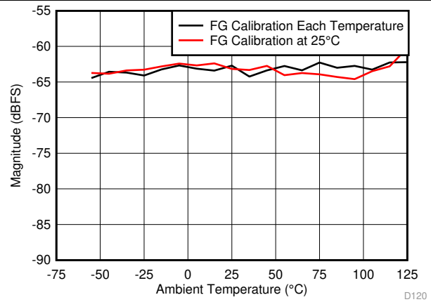
Figure 39. HD3 vs Temperature and Calibration Type
