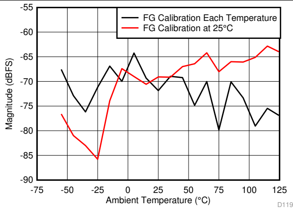
Figure 38. HD2 vs Temperature and Calibration Type
