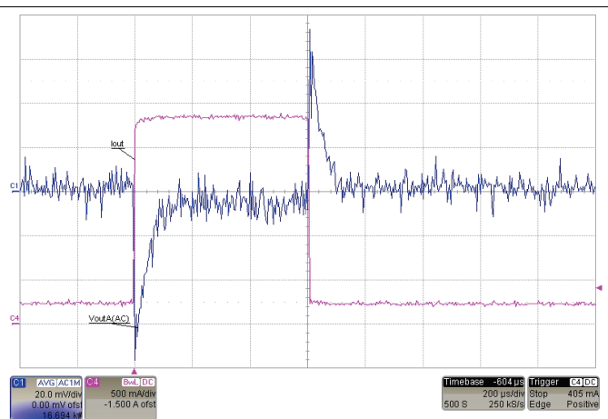
Figure 28. Buck Load-Step Response: BuckA 5 V, 200 mA to 2.4 A to 200 mA
