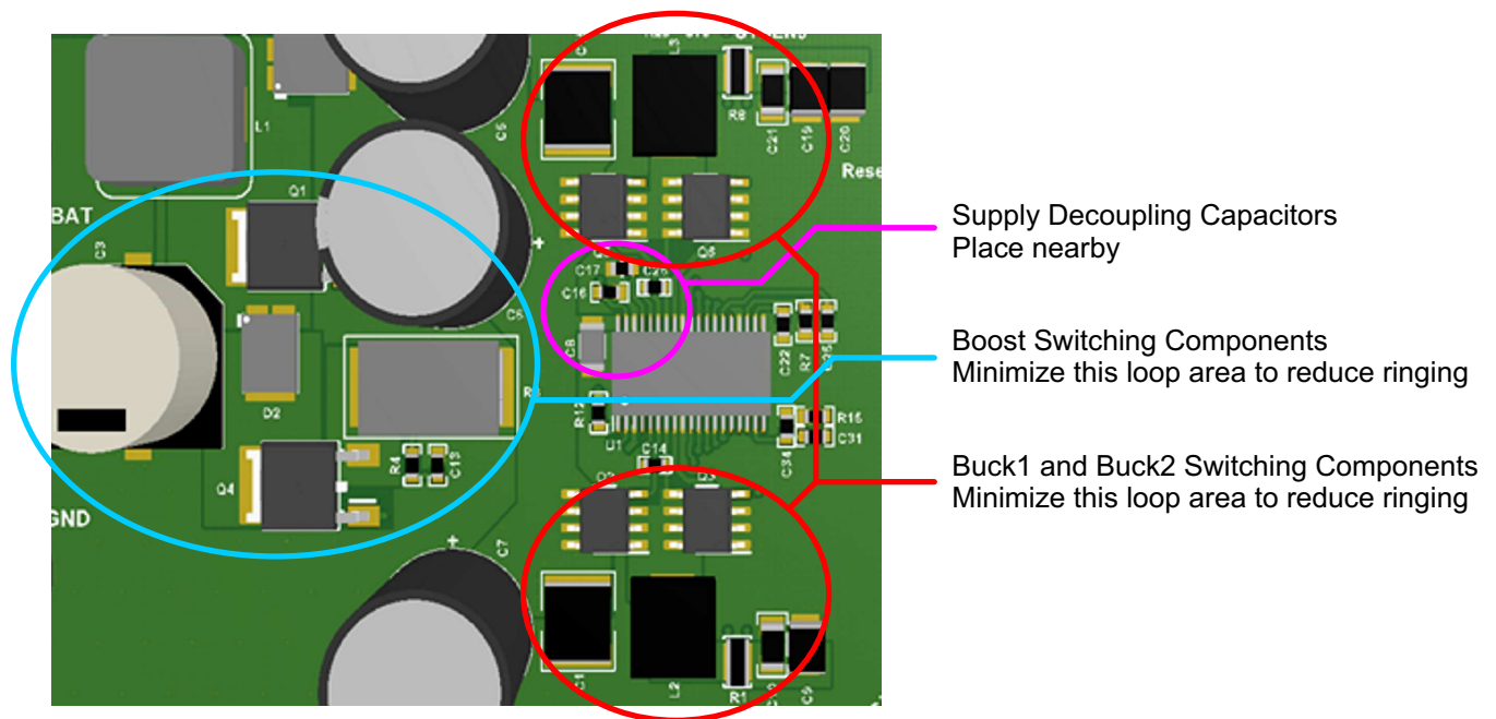
Figure 32. Layout Guidelines Highlighting Critical Paths
