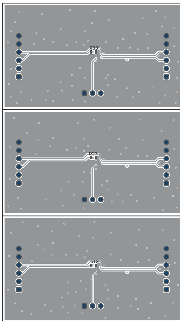
Figure 3-3. Bottom Layer
