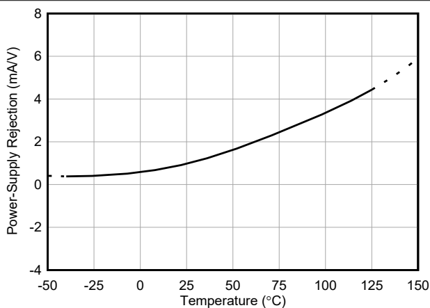
Figure 7-5. Power-Supply Rejection Ratio vs Temperature
