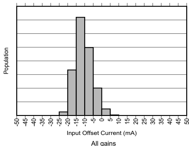
Figure 7-1. Input Offset Current Production Distribution
