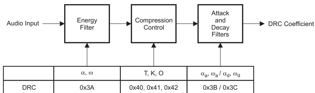
Figure 31. Dynamic Range Control
