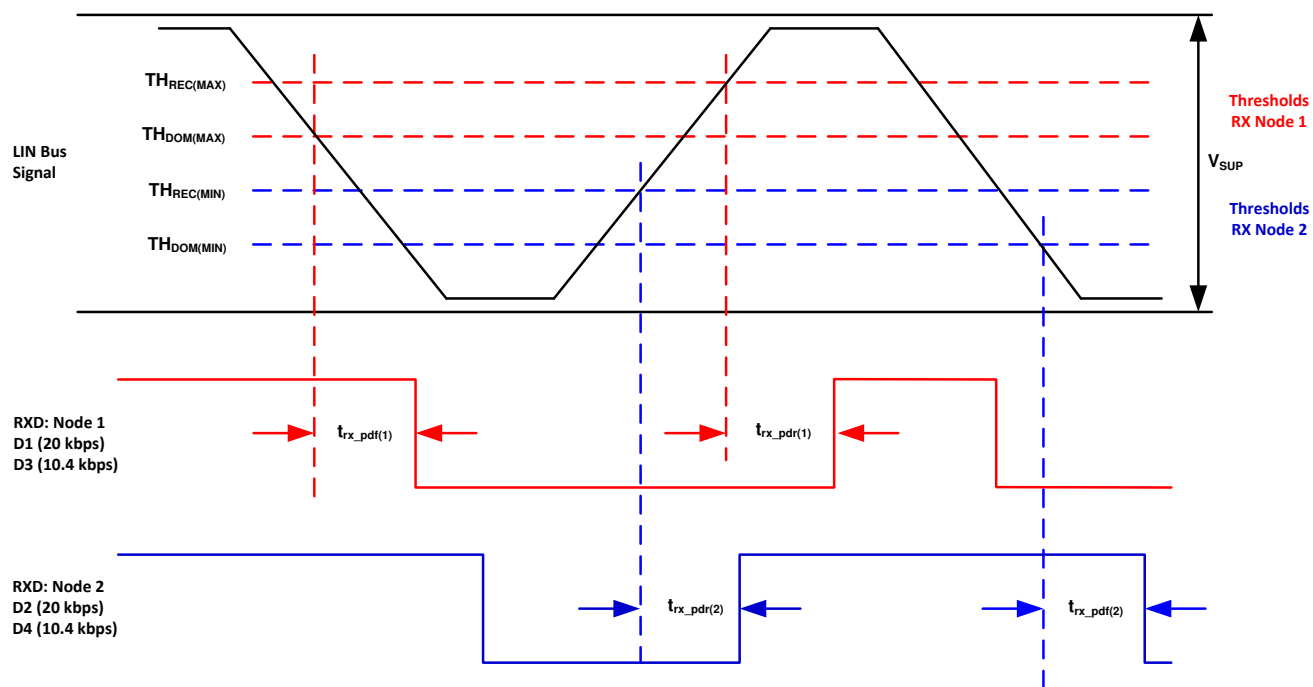
Figure 6-14. Propagation Delay
