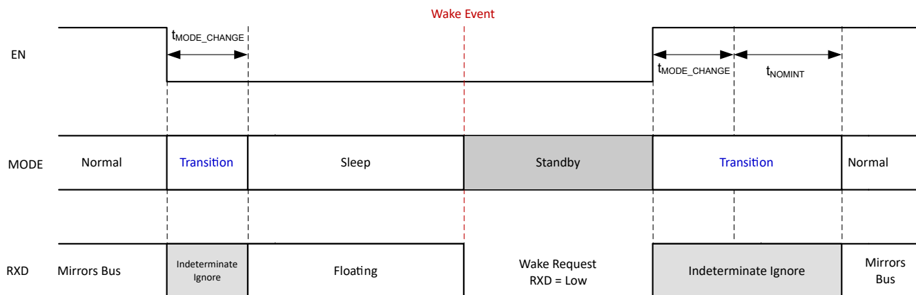
Figure 6-15. Mode Transitions
